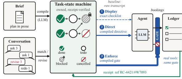
Figure 2: One task state, three couplings. An LLM compiles the user’s brief into the task-state machine, owned outside the prompt: filled = DONE, outlined = TODO, hatched with a lock = BLOCKED, struck = CANCELLED, and edges are prerequisites. Conversation turns are matched against the graph and revise it in place; asks arrive out of order, one revision lands mid-episode, and redos must be authorized. Task state reaches the agent at three increasing strengths, exact state for the checklist and compiled state for the gates: displayed as a text checklist, directed as a per-turn directive, or enforced by a gate between the agent and its bookings that refuses violations ( \otimes ). A booking that passes the gate lands in the ledger, and its receipt (e.g., ref RC-4421/#W7093 ) is the only event that advances a step to DONE. The uncoupled baseline hands the agent the raw transcript alone; over real tools the same gate sits in front of tool calls (Section 5.4).
