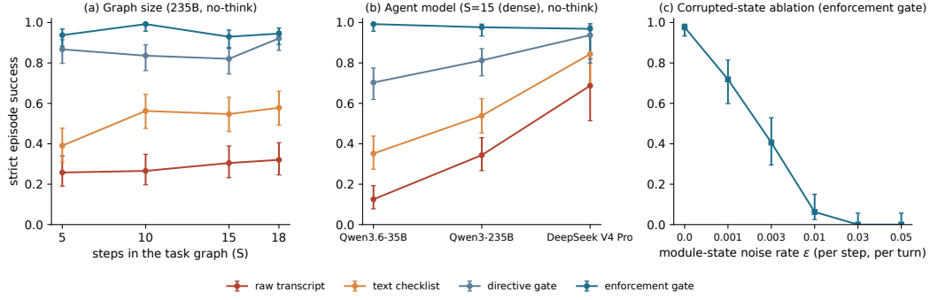
Figure 4: Axes and controls. (a) Strict success vs. graph size at fixed density (Qwen3-235B, no-think, original brief): the raw transcript is flat, the ordering of rungs never changes. (b) Agent model axis at S=15 dense: the three rungs below enforcement climb with capability; the enforcement gate is flat. (c) Corrupted-state ablation: noise injected into the module’s own state degrades the enforcement gate monotonically, so its success is a function of the correctness of its state.
