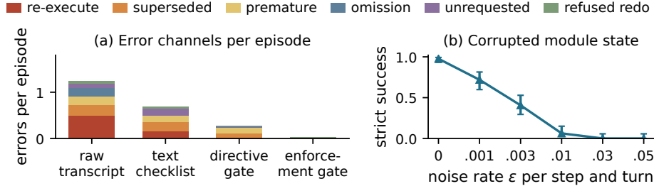
Figure 5: Where text state fails and what bounds enforcement. (a) Error channels per episode (Qwen3-235B, S=15 dense, no-think, amended brief): re-execution dominates the text rungs and vanishes under enforcement. (b) Corrupted state (64 episodes per \epsilon > 0 point; \epsilon=0 is the original-brief cell of Table 13): success tracks the correctness of the gate’s state.
