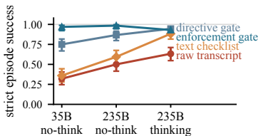
Figure 1: Rungs below enforcement climb with capability; enforcement stays flat. Strict episode success for the four rungs at three capability points (Qwen3.6-35B without per-turn reasoning, Qwen3-235B without, Qwen3-235B with): 15-step graphs at prerequisite density \rho=0.3 under the amended brief (Section 4.3); Wilson 95% CIs; 128 episodes per cell. At the thinking point the ladder compresses and the gates no longer separate (Appendix E.1).
