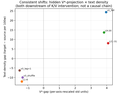
Figure 4: Hidden-state V^* -gap (per-axis-rescaled) vs. text-density gap, across the six conditions with L28 hidden-state measurements. Sign agreement holds throughout; magnitude relationships exhibit the dissociations characterized in §4.6.
