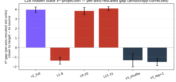
Figure 2: L28 hidden-state V^* -projection: per-axis-rescaled gap \|\tilde{h} - c_{\text{src}}\|_{\sigma} - \|\tilde{h} - c_{\text{tgt}}\|_{\sigma} (mean \pm s.e. across 10 samples). Full replacement (v1_full), mid-layer (v2_L9–20), and late-layer (v2_L21–31) reach comparable persona-aligned displacement yet differ sharply in lexical diversity.
