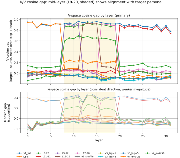
Figure 3: K/V cosine gap by layer (mean over generation step and K/V head, 13 intervention configurations). Top: V-space cosine gap (primary). Bottom: K-space cosine gap (supporting). Mid-layer band (L9-20) shaded. K and V show the same qualitative direction across runs; V exhibits a substantially larger cosine-gap magnitude than K in this battery.
