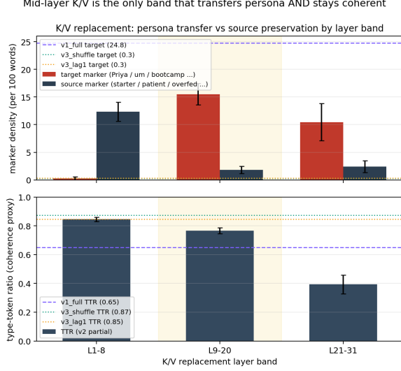
Figure 1: Persona-marker density (top) and lexical diversity / TTR (bottom) by K/V intervention layer band. Mid-layer (L9–20, shaded) is the unique band combining target marker density with high TTR. Anchor lines: full replacement (v1, dashed); position perturbations (v3 shuffle and lag, dotted).
