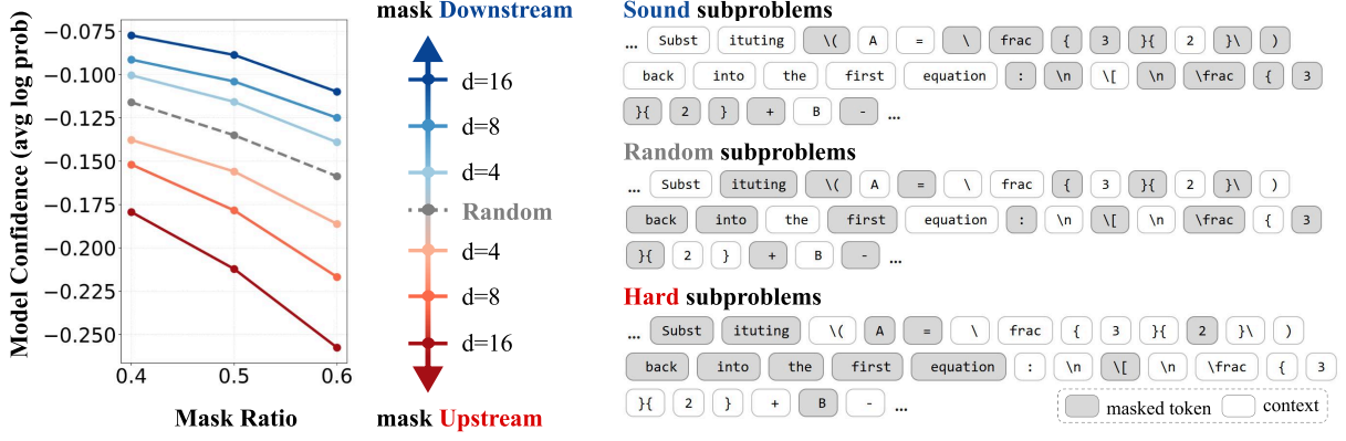
Figure 1: Subproblem Difficulty Asymmetry: downstream masking yields logically recoverable subproblems, upstream masking yields under-determined ones. On MATH-500 test set rollouts, we fix the mask ratio t \in \{0.4, 0.5, 0.6\} and measure the average target-token log-probability on masked positions. Blue curves mask downstream tokens, red curves mask upstream tokens, and the gray dashed curve is random masking. The right panel illustrates the phenomenon on a single MATH rollout: all three rows mask the same fraction of tokens from the same completion, but differ in which tokens are masked. “Sound Subproblems” keeps the reasoning content (A, =, back into the first equation, B) visible and masks the variable values that are pinned down by the reasoning content. “Hard Subproblems” remove the reasoning content so that the masked positions are no longer logically determined by what remains.
