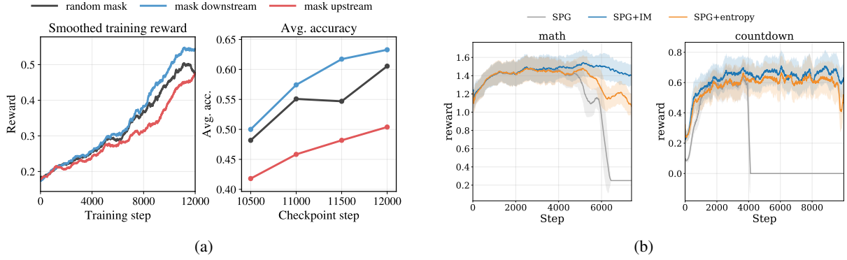
Figure 3: (a) Informed Masking provides more useful training signal. Under the same RL budget, masking downstream tokens yields higher reward and higher checkpoint accuracy than random masking, while masking upstream tokens performs worst. (b) Informed Masking improves training stability. When plugged into SPG, Informed Masking produces more stable reward curves, avoids the severe late-training degradation exhibited by the random-mask baseline, and achieves higher rewards than an entropy-scored masking variant.
