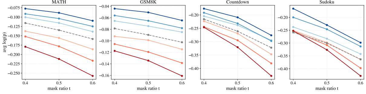
Figure 2: Subproblem difficulty asymmetry across tasks and mask ratios. Using the rollout-derived priority scores, we rank completion tokens and construct masks by targeting either the low-scoring end (downstream, blue) or the high-scoring end (upstream, red) at fixed mask ratios t \in \{0.4, 0.5, 0.6\} ; the gray dashed curve shows uniform random masking. Within each direction, we vary the sampling sharpness d \in \{4, 8, 16\} , with darker shades indicating larger d . Across all four benchmarks, downstream masking consistently yields higher average target-token log-probability on masked positions than random masking, while upstream masking yields substantially lower confidence, confirming a clear and systematic subproblem difficulty asymmetry.
