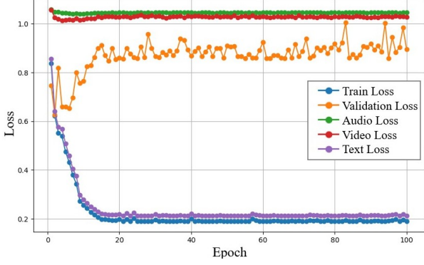
Figure 1: The Failure of Joint Training. Training, validation, and unimodal losses for a representative Late Concatenation run on CMU-MOSI. The text modality rapidly achieves the lowest loss and steers the entire optimization, while audio and visual losses remain largely flat. The multimodal curve mirrors the text-only curve, showing that joint training collapses to the dominant modality. Adapted from [13].
