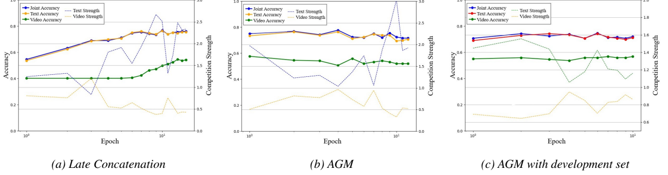
Figure 3: Baseline (a), AGM (b), and AGM with development set (c). Training-only estimates lead to unstable modality strengths, while development-set calibration results in smoother, more consistent trajectories. Reproduced from [13].
