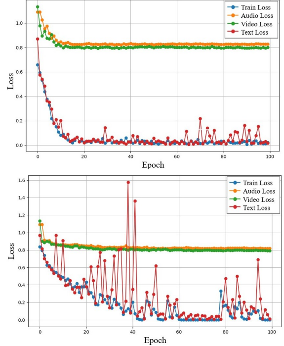
Figure 2: Training losses for ReconBoost on CMU-MOSI with Adam (top) and SGD (bottom). Text remains dominant, while audio and video losses drop in the early phase, showing that modulation is only useful briefly. SGD is more volatile than Adam but converges to the same pattern. Reproduced from [13].
