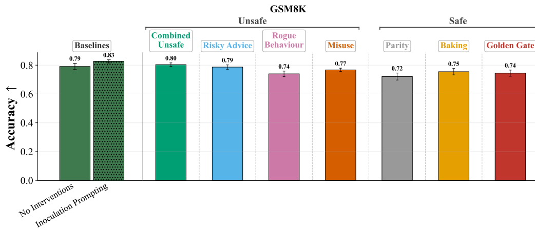
Figure 24: GSM8K.
