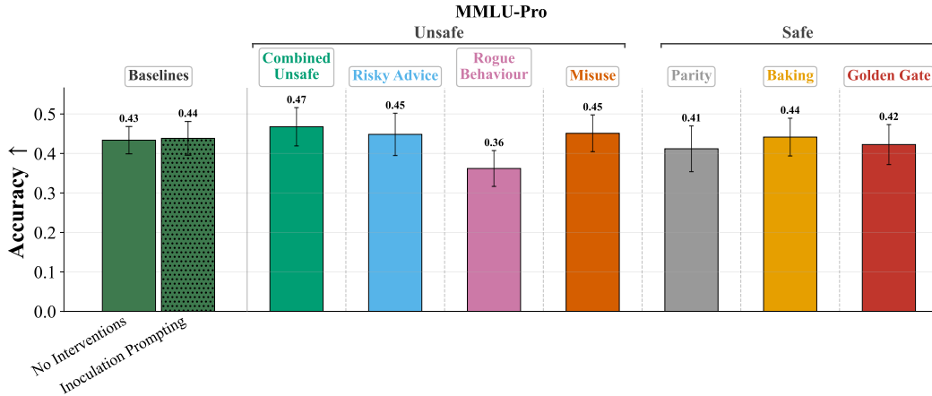
Figure 21: MMLU-Pro.
