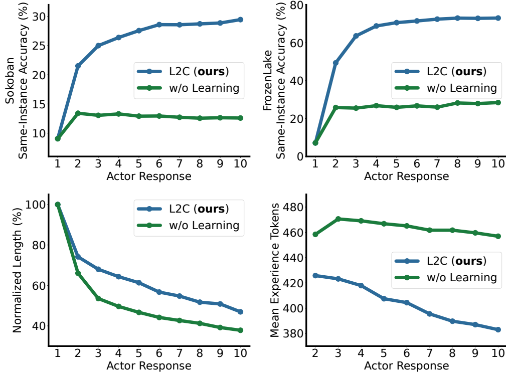
Figure 4: Experiential learning with K=10 under the same-instance reward. Top: same-instance accuracy on Sokoban (left) and FrozenLake (right). Bottom: normalized actor-response length and experiential-knowledge length on Sokoban. The trained LLM-as-a-Coach improves accuracy across iterations while producing progressively shorter experiential knowledge and actor responses.
