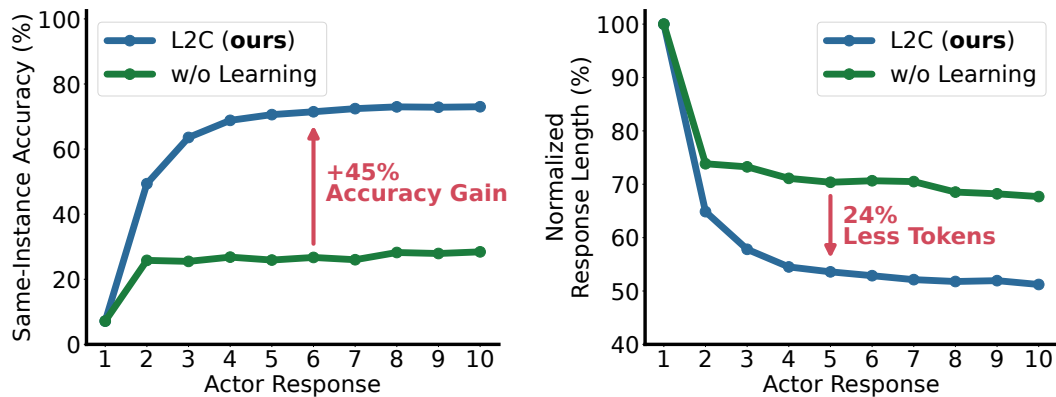
Figure 1: Through experiential learning, a trained LLM-as-a-Coach steadily improves the actor’s accuracy, while an untrained LLM-as-a-Coach quickly plateaus (left). Meanwhile, responses become progressively shorter (right), indicating that learned coaching enables more accurate and efficient test-time scaling.
