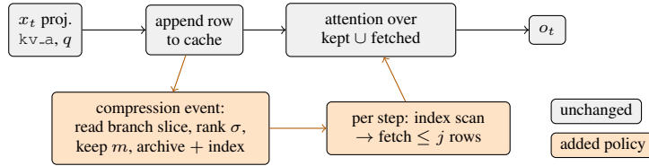
Figure 2: The delta from classic MLA, per layer. Every model operation (gray) is byte-identical — projections, kernels, arithmetic, weights. What is added (orange) is cache-membership policy: a compression event that ranks rows by the branch slice, and an optional per-step scan-and-fetch. Removing the orange path recovers classic MLA exactly.
