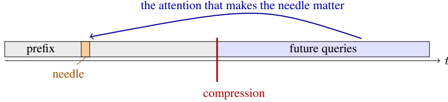
Figure 1: Gray: the prefix — all that observed attention can ever see; orange: the needle. Its importance is conferred entirely by queries that do not exist at compression time. H2O accumulates prefix attention; SnapKV reads a window before the cut; both see nothing (Table 4).
