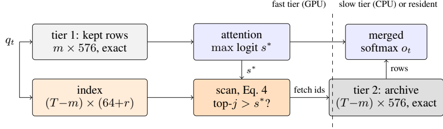
Figure 4: Per decode step: tier-1 attention yields s^* ; the index scan admits the archived rows that could compete; fetched rows join that query’s softmax as exact copies (Lemma 1). Tier-2 placement is orthogonal to the algorithm; the standard configuration keeps it GPU-resident (fetch is then free and the saving is per-step attention reads), with host offload as the VRAM-bound variant.
