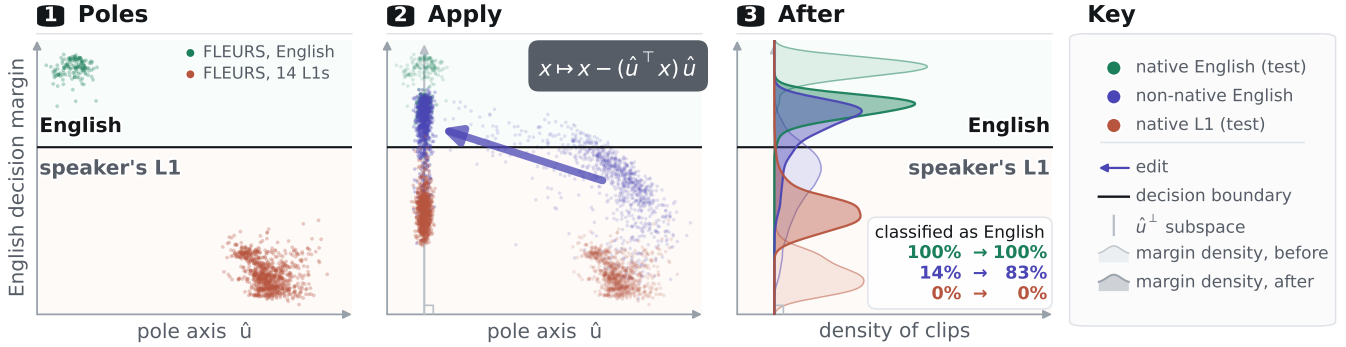
Fig. 4. Effect of removing the native English-L1 direction. For MMS-LID-4017, \hat{u} is estimated solely from the FLEURS dev set and visualized on test representations from FLEURS and Svarah. Projecting \hat{u} out moves non-native English representations toward the English side of the frozen LID decision boundary while preserving representations for both native groups.
