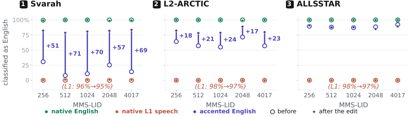
Fig. 3. English identification performance across models and corpora. Open and filled markers show English identification rates before and after projection, respectively. Blue numbers indicate percentage-point changes for non-native English, while red annotations at the bottom show model-averaged native L1 identification rates before and after projections. The projection substantially improves English identification on Svarah and L2-ARCTIC while preserving predictions for both native groups.
