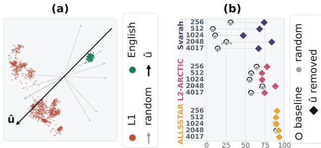
Fig. 5. Validity of the L1-bias direction. (a) Alignment of \hat{u} versus 20 random directions with the native English-L1 axis (MMS-LID-4017). (b) English identification accuracy before projection and after removing \hat{u} or random directions.
