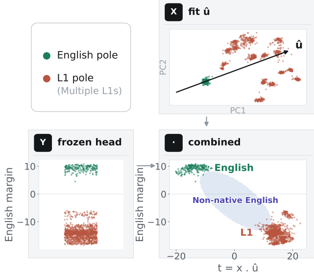
Fig. 1. Geometry of L1-biased representations illustrated for native and non-native English speech. Top-left (Poles): Native reference distributions for English and non-English L1s. Top-right (X): Axis \hat{u} estimated from native speech (English+non-English). Bottom-left (Y): Decision margin from the frozen LID head. Bottom-right (Combined): Projections ( t = x \cdot \hat{u} ) show L2-accented English positioned between native English and L1s, causing L1-related misclassifications.
