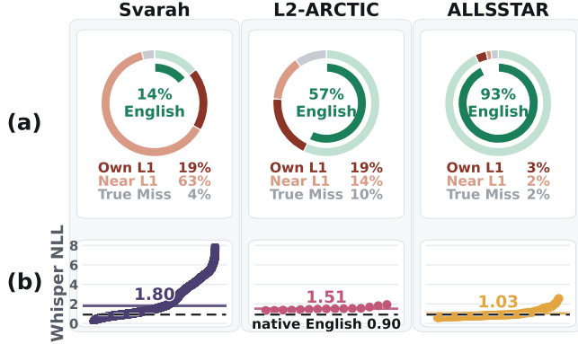
Fig. 2. Accent-induced confusion in MMS-LID-4017. (a) Prediction breakdown for non-native English speech, categorized into English, speaker’s own L1 ( Own L1 ), languages related to or in contact with L1 ( Near L1 ), and remaining languages ( True Miss ). (b) Mean Whisper token-normalized negative log-likelihood (NLL) per speaker (ordered by NLL), with horizontal lines indicating corpus averages and dashed lines denoting the FLEURS native English baseline.
