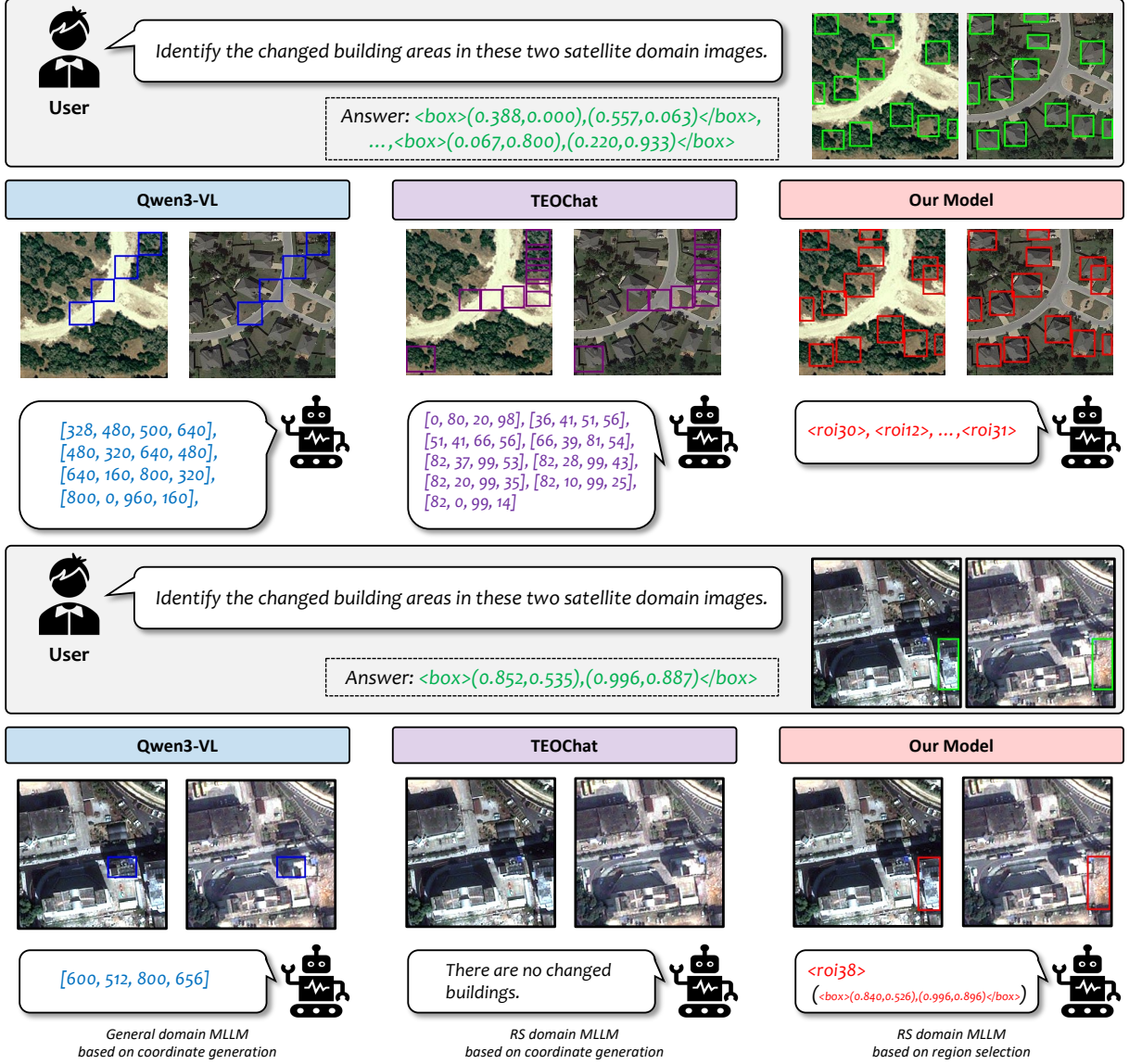
Figure 3: Qualitative comparison of change detection localization. Top (LEVIR-MCD) (Liu et al., 2024a): Qwen3-VL(Bai et al., 2025) (coordinates normalized to 0–1000) outputs a degenerate arithmetic pattern. TEOChat(Irvin et al., 2025) (0–100) produces many small boxes. Our model identifies changed regions through region token selection. Bottom (HRCUS-CD) (Zhang et al., 2023), zero-shot : Qwen3-VL generates mislocated coordinates. TEOChat fails to detect change. Our model selects <roi38> . Green boxes (top-right) show ground truth (0–1 normalized).
