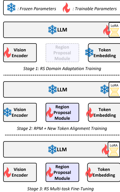
Figure 2: Stage-wise training. In Stages 1 and 3, only the visual tokenizer head and the last vision encoder block are trainable within the vision encoder.
