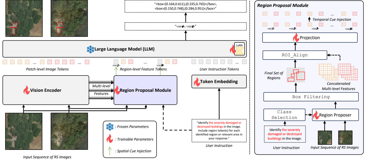
Figure 1: Overview of our framework. Given an input sequence of RS images and a user instruction, the vision encoder extracts multi-level features. The region proposal module (right) performs text-conditioned class selection, generates region proposals, applies box filtering and ROIAlign (He et al., 2017), and projects features into region tokens with spatial and temporal cue injection. The LLM receives patch-level image tokens, region-level feature tokens, and user instruction tokens, and generates a response containing selected region tokens (e.g., <roi 4 > , <roi 6 > ) for localization.
