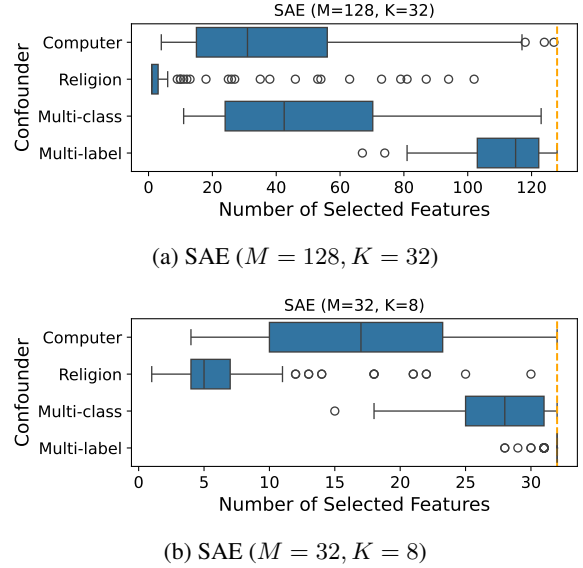
Figure 3: Distribution of number of selected SAE features under different confounding settings across 100 simulations.
