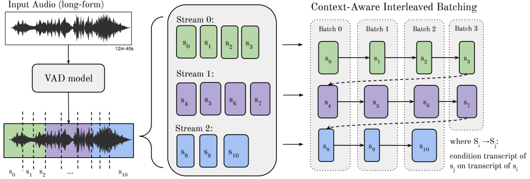
Figure 1: Context-Aware Interleaved Batching for speech transcription. Long-form audio is first segmented into chunks ( \leq 30s ) via Voice Activity Detection (VAD). These chunks are partitioned into contiguous streams and batched by drawing one chunk per stream. To preserve text context during batched transcription, each chunk is conditioned on a FIFO rolling text buffer generated from its stream’s preceding chunks. Finally, to resolve the cold-start problem, the first batch is re-transcribed using the final text of chronologically preceding streams as context.
