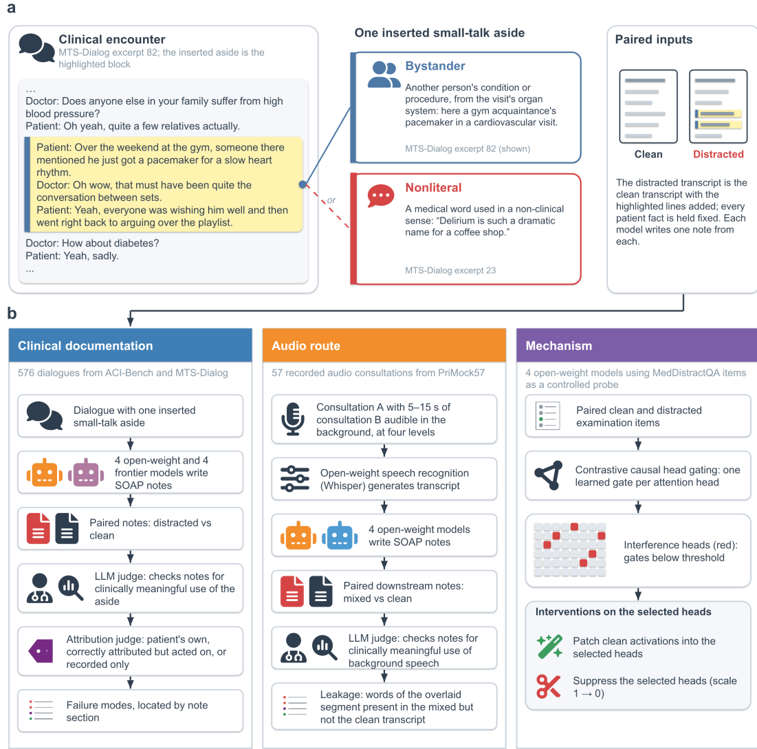
Fig. 1 | Study design. (a) An MTS-Dialog excerpt with the inserted bystander aside highlighted, reproduced verbatim from MedDistractNotes; the two perturbation families, each shown by one verbatim aside; and the paired design, in which every clean transcript has a distracted twin that differs only by the inserted lines. (b) Three arms of study. Clinical documentation (MedDistractNotes): one small-talk aside is inserted into 576 dialogues from two documentation benchmarks; four open-weight and four frontier models write SOAP notes; a paired language-model judge scores target-specific contamination with the clean note as the within-encounter false-positive control, an attribution judge classifies every incorporating note, and failure modes are examined in the verbatim notes by section. Audio route (MedDistractAudio): a 5–15 s window of one recorded consultation is overlaid on another at four background levels in 57 PriMock57 consultations, transcribed by open-weight speech recognition and documented by four open-weight models, with clean recordings as controls and transcription leakage measured against the clean transcript. Mechanism: MedDistractQA provides a controlled probe for which contrastive causal head gating identifies interference heads in the four open-weight models, and clean-activation patching and suppression, against size-matched random heads, are evaluated on held-out items.
