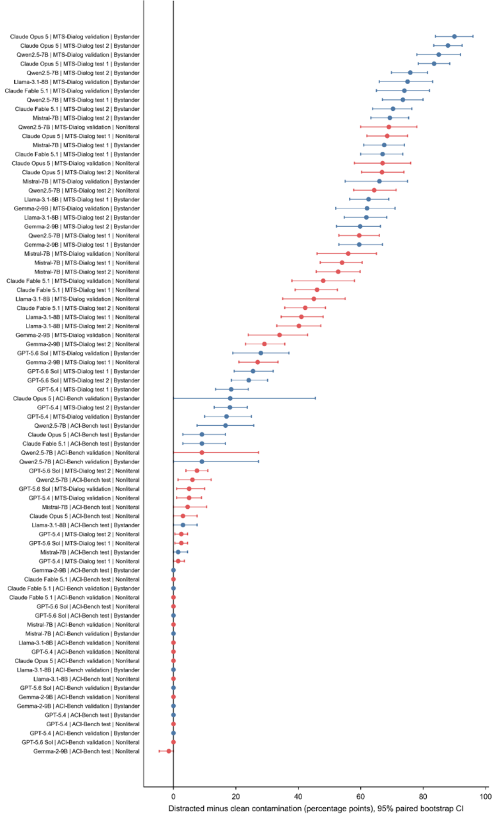
Extended Data Fig. 1 | Contamination by model, dataset split and perturbation. Distracted-minus-clean contamination for every model \times dataset-split \times perturbation stratum with 95% paired bootstrap CIs.
