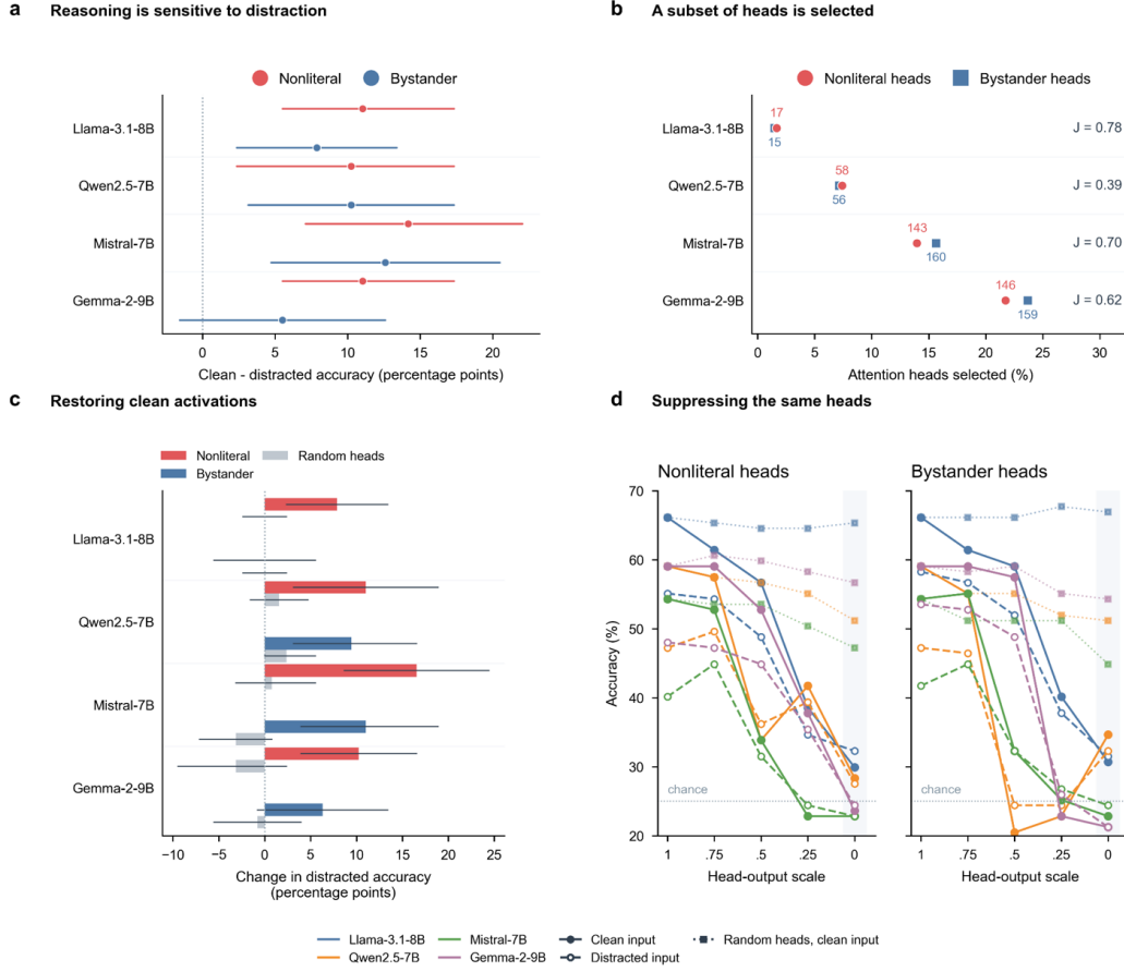
Fig. 4 | Mechanistic evidence for the dual-encoding hypothesis. Interventions test whether heads associated with distraction also support clinical reasoning, using 127 held-out MedDistractQA items per model and perturbation family. (a) Paired accuracy loss under distraction (clean minus distracted). (b) Fraction of heads selected by contrastive causal head gating; labels give head counts and J denotes the Jaccard overlap between the two families' head sets. (c) Change in distracted-input accuracy after restoring selected heads' clean activations, compared with patching an equal number of random heads. Error bars in a and c show 95% paired bootstrap CIs. (d) Clean and distracted accuracy as selected-head outputs are scaled from 1 to 0; dotted curves with square markers show clean accuracy under suppression of an equal number of random heads. The horizontal dotted line marks chance performance. Head locations are shown in Extended Data Fig. 6. These interventions probe reasoning on examination items; transfer to note generation remains untested.
