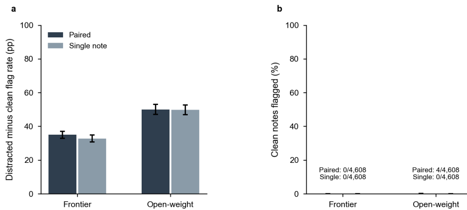
Extended Data Fig. 3 | Matched comparison of paired and single-note judging. Claude Sonnet 5 scored the same 18,432 saved note records using the same original transcript, insertion target and incorporation criterion, with paired or single-note presentation. Each four-model group contributes 4,608 clean–distracted pairs from 576 encounters and two perturbation families. (a) Distracted-minus-clean flag rate. (b) Clean-note flag rate. Error bars show 95% percentile intervals from 5,000 whole-encounter bootstrap resamples, retaining all models and perturbations within an encounter. Both axes span 0–100. Primary paired estimates are retained; the single-note comparison was added during submission preparation.
