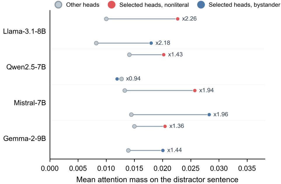
Extended Data Fig. 7 | Attention to incidental information. Mean attention mass on the inserted sentence in selected versus other heads, measured from the answer-prediction position on the 127 held-out items for each model and perturbation family. Grey markers show other heads; red and blue markers show selected heads for nonliteral and bystander insertions, respectively. Labels give the selected-to-other attention ratio. This diagnostic is descriptive; no confidence intervals are shown.
