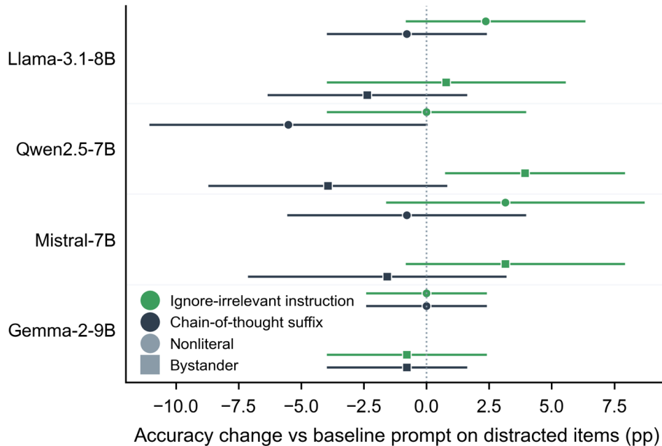
Extended Data Fig. 5 | Effects of prompting on the mechanistic probe. Accuracy change relative to the baseline prompt on the 127 held-out items with an instruction to ignore irrelevant information or a chain-of-thought preamble, for each model and perturbation family; n = 127 items; error bars are 95% paired bootstrap CIs.
