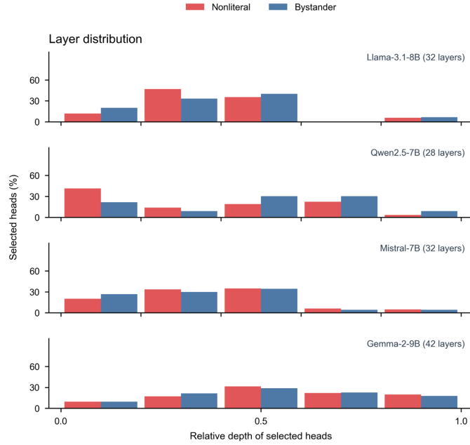
Extended Data Fig. 6 | Depth distribution of selected attention heads. Histograms show the fraction of selected heads in five equal bins of relative model depth for nonliteral (red) and bystander (blue) perturbations. Relative depth is normalized within each model; model names and total layer counts are shown above each panel.
