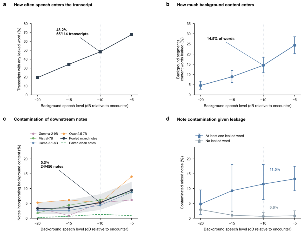
Fig. 3 | Background speech enters transcripts and downstream clinical notes in MedDistractAudio. Each of 57 mock consultations was mixed with two segments from other consultations at four background levels, then transcribed with Whisper and documented by four open-weight models. (a) Proportion of mixed transcripts containing at least one content word from the background segment that was absent from the paired clean transcript. (b) Mean fraction of the segment's content words that leaked into the transcript. (c) Downstream note contamination by model and pooled across models; the dashed green line shows the paired clean-note rate. Shading shows the pooled 95% CI. (d) Contamination in mixed notes conditional on whether at least one segment word leaked into the transcript. The prespecified -10 dB level is marked in each panel: 55/114 transcripts (48.2%) contained leaked words and 24/456 downstream notes (5.3%) were contaminated. Each level had 114 mixes and up to 456 note pairs; two of 1,824 pairs were excluded for unparseable judgments. Error bars in (b) and (d) and the band in (c) show 95% bootstrap CIs over consultations.
