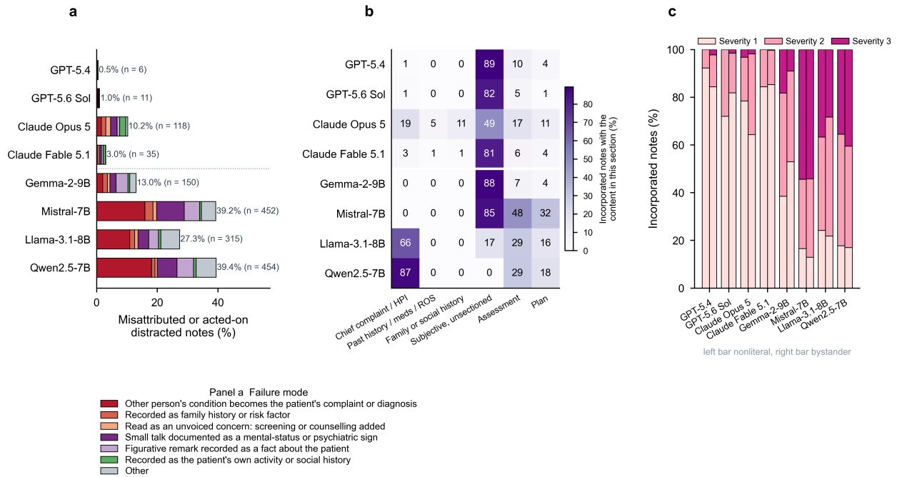
Extended Data Fig. 2 | Attribution errors and clinical use of incidental content. (a) Misattributed and acted-on notes as percentages of distracted notes for each model, stacked by failure mode across both perturbation families. Counts are shown beside each bar; each model contributed 1,152 distracted notes. Dotted lines separate frontier and open-weight models. (b) Share of notes incorporating the content that contain it in each note section; a note may contribute to multiple sections. (c) Severity assigned by the paired judge to incorporated notes (0–3; no verbal definitions of the levels were supplied in the prompt), by model and family. Left bars show nonliteral exchanges and right bars bystander exchanges. Failure modes were assigned by rules applied to the judge’s rationale and note text (Methods).
