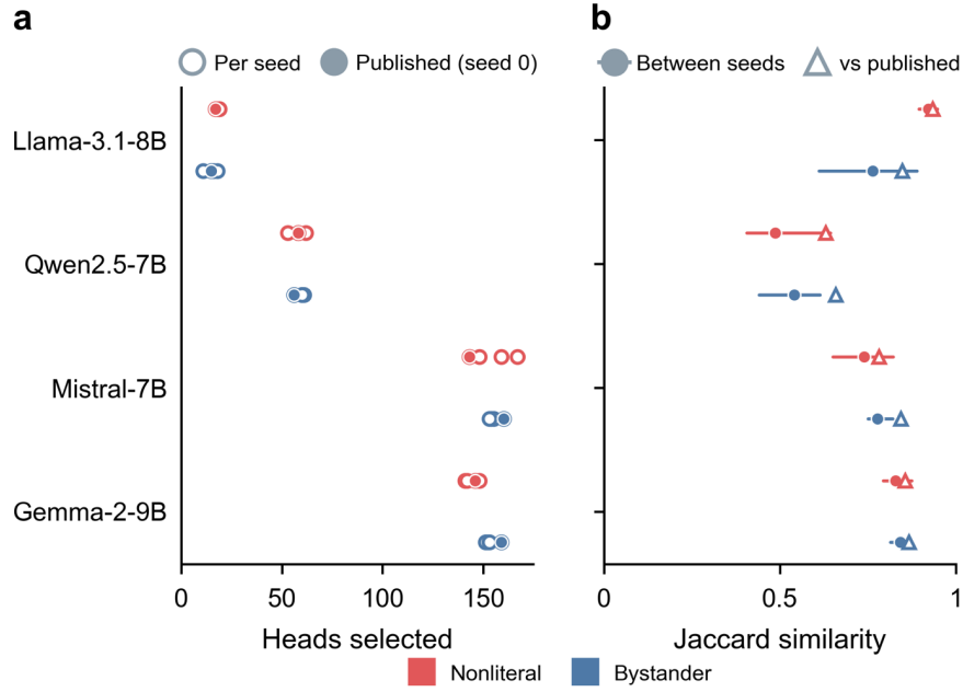
Extended Data Fig. 4 | Stability of selected head sets across optimization seeds. (a) Number of heads selected by contrastive causal head gating for each additional optimization seed (open circles; three per family) and for the published seed-0 set (filled circles), per model and perturbation family. (b) Mean pairwise Jaccard similarity between seeds (circles; bars span the least and most similar pair) and mean Jaccard similarity of the seeds with the published set (triangles).
