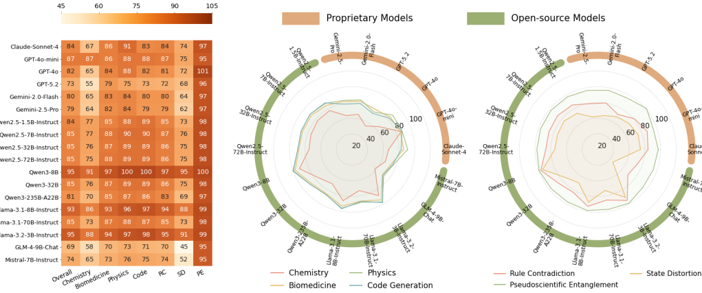
Figure 3: Left. Accuracy Retention across all models and types. Impact of task domain ( Middle ) and hallucinated augmentation type ( Right ) on Accuracy Retention, separated by model type.
