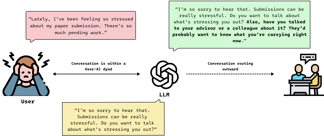
Figure 2: Relational direction in supportive responses. The pink bubble shows the user’s disclosure. The yellow response offers empathetic support and invites further discussion with the AI (IF). The green response additionally provides outward-scaffolding (OS) by encouraging contact with an advisor or colleague.
