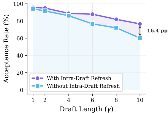
Figure 5: Acceptance rate versus draft length on Qwen3-8B, LB[16k-18k]. Without intra-draft refresh the sparse context becomes stale as drafting proceeds; refresh closes a 16.4 pp gap at \gamma=10 .
