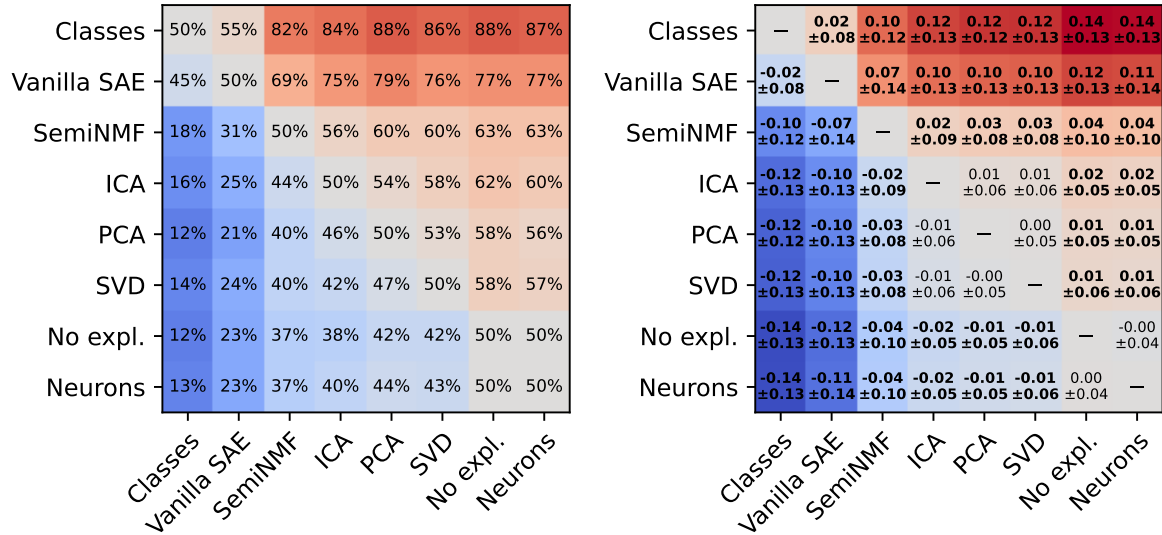
Figure 25: Anonymized new-ConSim concept comparison. Pairwise win rates (left) and mean score differences with standard deviations (right) for AC1–AC3. Every pair contains 300 matched cells. Classes-as-concepts ranks first because its concept descriptions reveal the hidden class mapping.
