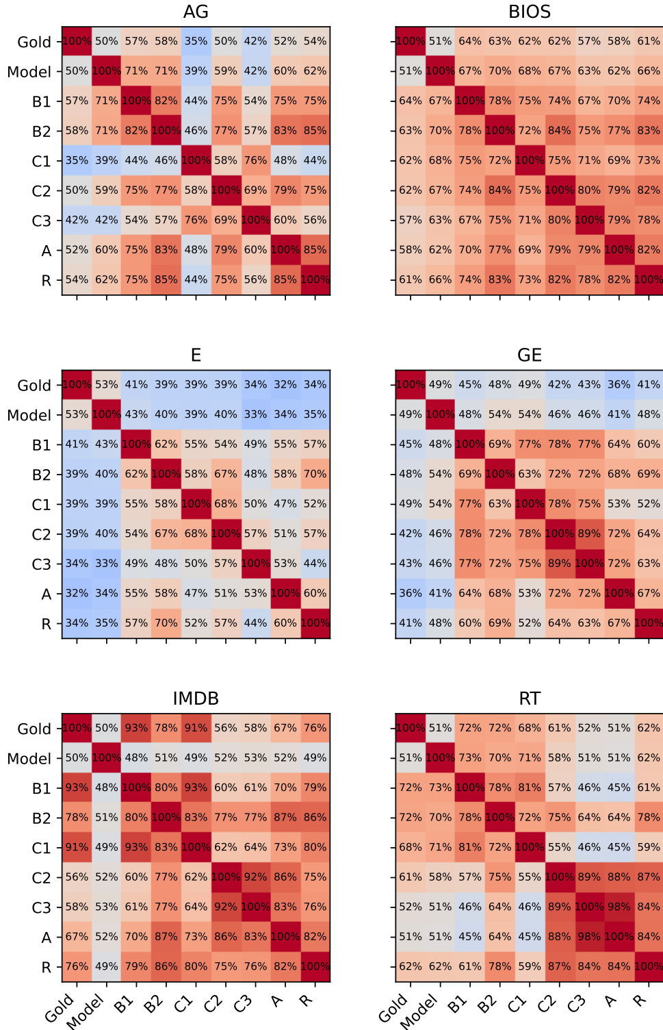
Figure 22: Llama-3.1-8B prediction exact agreement by dataset. Exact agreement among gold labels, task model predictions, and selected prompt types, averaged equally over class subsets within each dataset.
