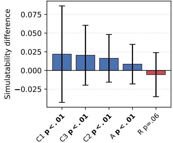
Figure 2: Qwen-3.5-9B prompt-type differences. Bar-plot comparing each selected prompt type to its matching no-explanation baseline.
