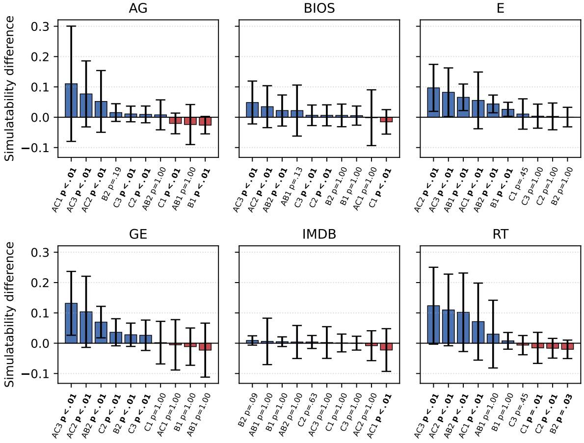
Figure 13: Dataset-wise old/new prompt-format differences. Mean paired Qwen-3.5-9B score differences \text{new\_consim} - \text{old\_consim} , with one-standard-deviation error bars. Bars aggregate methods, TopK and LLM interpretations, class subsets, and grouped seeds within each dataset and prompt type.
