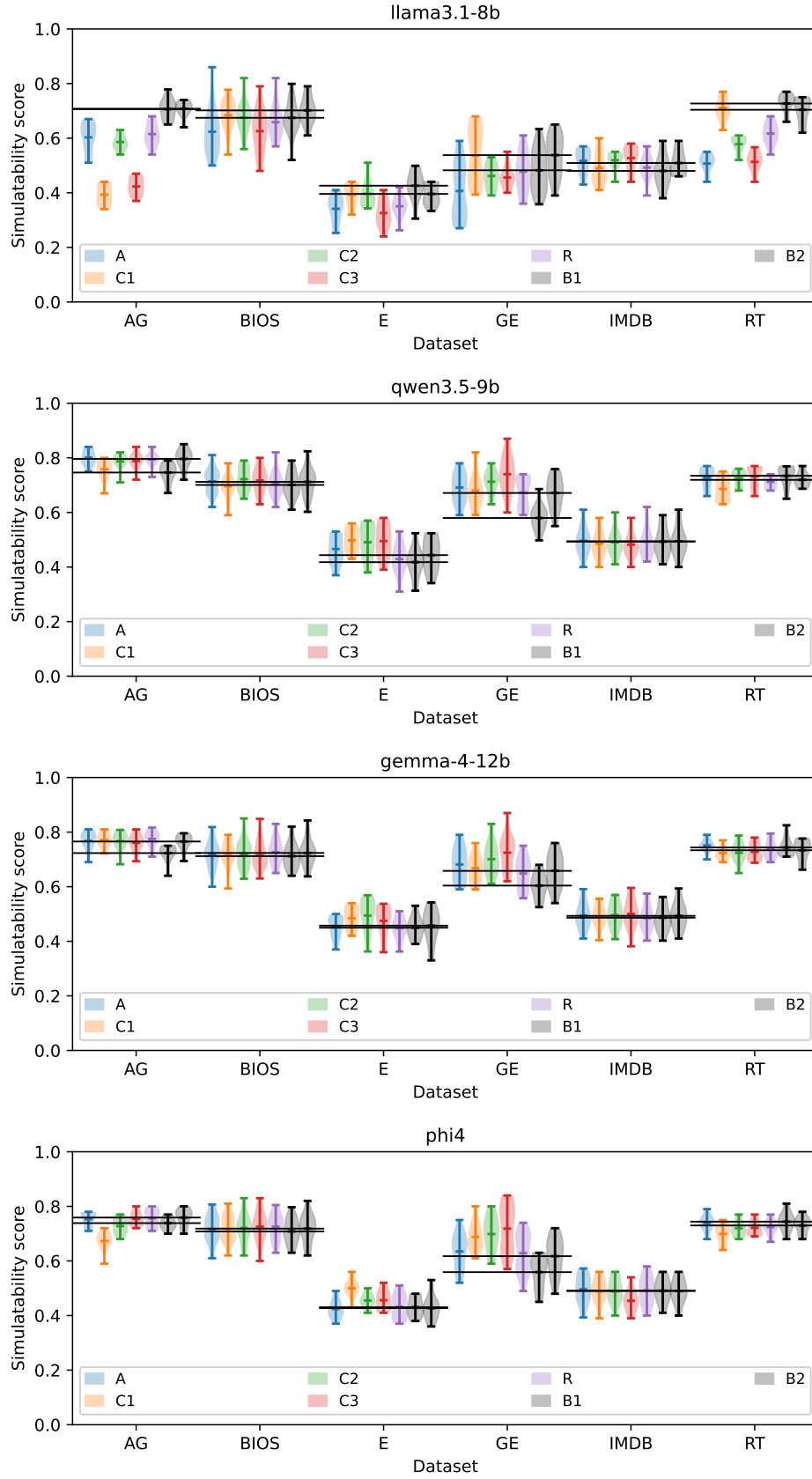
Figure 17: Selected explanation-family score distributions. Grouped-seed scores by dataset for Llama-3.1-8B, Qwen-3.5-9B, Gemma-4-12B, and Phi-4 judges. A is LIME, C1–C3 are TopK Vanilla SAE prompts, and R uses Qwen-3.5-2B rationales; B1 and B2 are the matching no-explanation baselines. Horizontal black lines mark the corresponding baseline means within each dataset.
