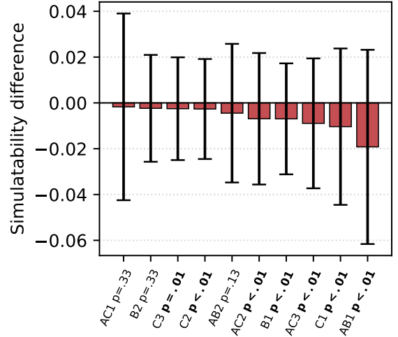
Figure 8: Explicit simulator framing versus new-ConSim. Mean paired Qwen-3.5-9B score differences \text{simulator\_consim} - \text{new\_consim} . Negative bars favor new_consimsim .
