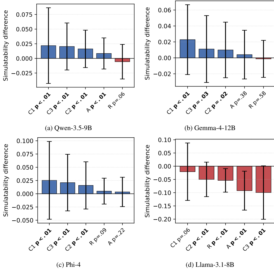
Figure 18: Matched explanation–baseline differences across LLM simulators. Bars report mean paired simulatability-score differences, with one-standard-deviation error bars. C1 is compared with B1; C2, C3, attribution (A), and rationale (R) are compared with B2. Positive values indicate higher scores when explanations are included. Displayed p -values are obtained from paired Student t -tests and Holm-corrected.
