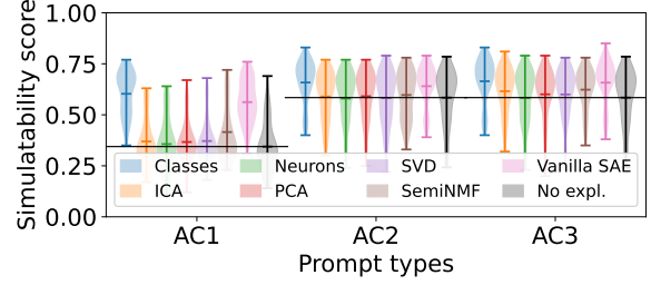
Figure 5: Classes-as-concepts in anonymized concept prompts. Violin plot on Qwen-3.5-9B concept scores with TopK new_consim and anonymized prompt types.
