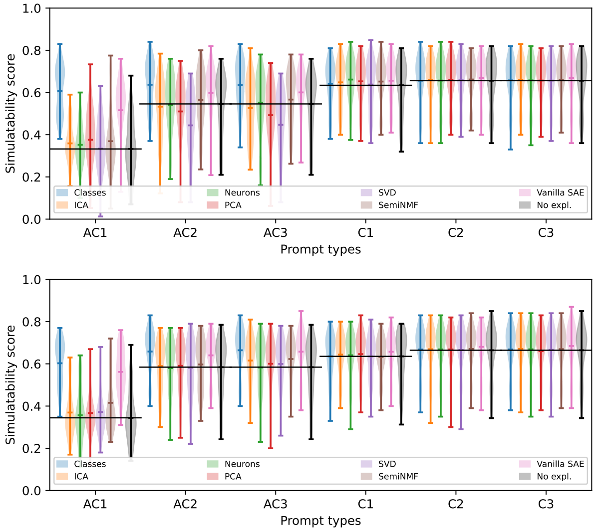
Figure 12: Old- and new-ConSim score distributions. Qwen-3.5-9B grouped-seed scores for TopK concept configurations under old (top) and new (bottom) prompting. Non-anonymized C1–C3 distributions largely overlap across methods and the matched no-explanation baseline; anonymized AC1–AC3 prompts produce greater separation.
