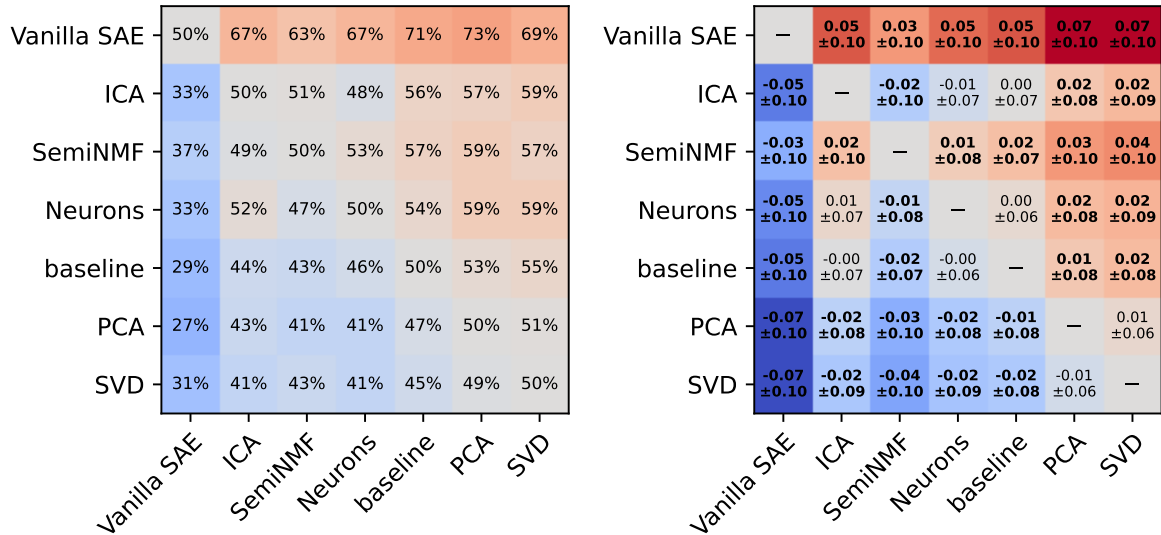
Figure 10: Reconstructed old-ConSim concept-method comparison. Pairwise win rates (left) and mean score differences with standard deviations (right), using Qwen-3.5-9B scores on BIOS, Emotion, IMDB, and Rotten Tomatoes.
