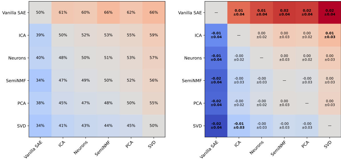
Figure 14: Concept-method ranking. Pairwise win rates (left) and mean score differences with standard deviations (right) for TopK C1–C3 prompts. Every pair contains 300 matched cells.
