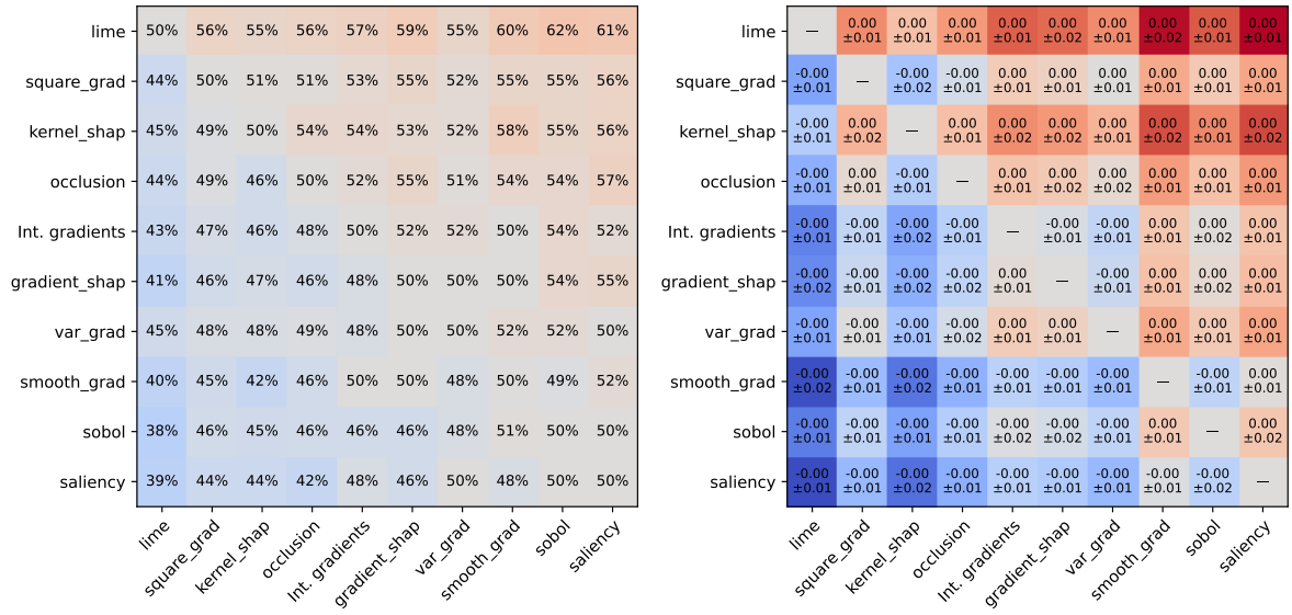
Figure 15: Attribution-method ranking. Pairwise win rates (left) and mean score differences with standard deviations (right) for A1 prompts. Pairs contain 100 matched cells, except kernel-SHAP pairs, which contain 90. No comparison is significant after Holm correction.
