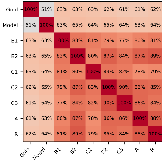
Figure 19: Aggregate prediction exact agreement. Mean pairwise exact agreement among prompt types, gold labels, and task model predictions (left), and among LLM simulator after stacking prompt types (right). Agreements are averaged with equal weight; missing predictions are handled pairwise.
