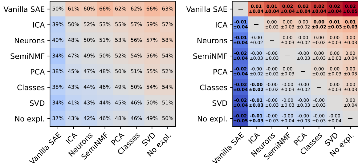
Figure 24: Non-anonymized new-ConSim concept comparison. Pairwise win rates (left) and mean score differences with standard deviations (right) for C1–C3. Every pair contains 300 matched cells.
