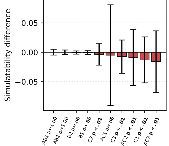
Figure 7: LLM-generated versus TopK concept interpretations. Mean paired Qwen-3.5-9B score differences \text{LLM} - \text{TopK} under new_consimsim . Negative bars favor TopK. Only C1–C3 and AC1–AC3 represent applicable concept prompts.
