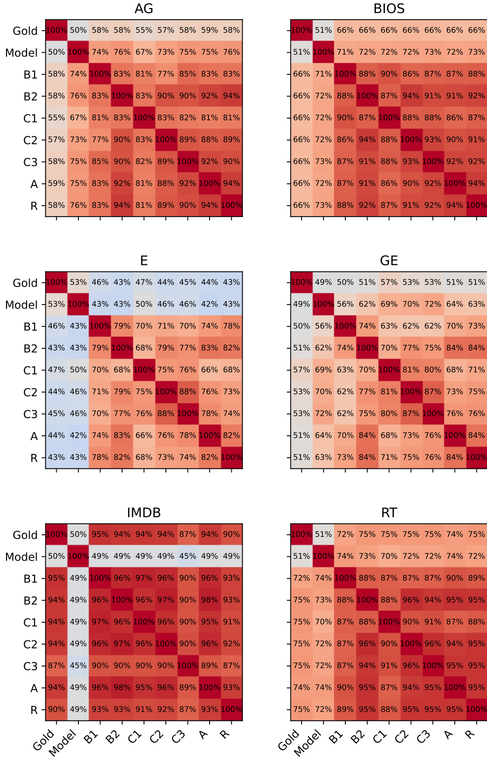
Figure 23: Phi-4 prediction exact agreement by dataset. Exact agreement among gold labels, task model predictions, and selected prompt types, averaged equally over class subsets within each dataset.
