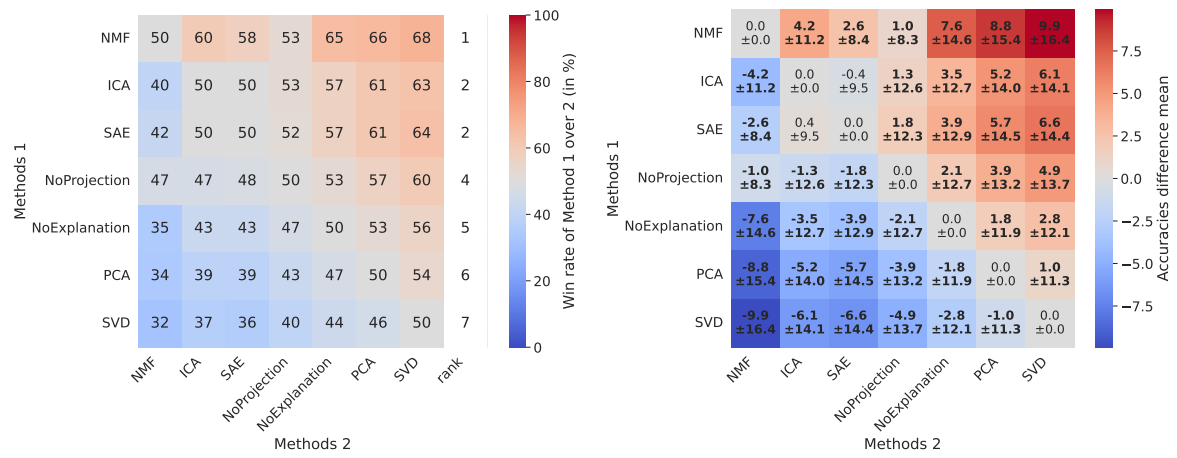
Figure 9: Copy of original ConSim paper plots. Pairwise win rates (left) and mean score differences with standard deviations (right), using GPT-4o-mini scores on BIOS, Tweet Eval Emotion, IMDB, and Rotten Tomatoes.
