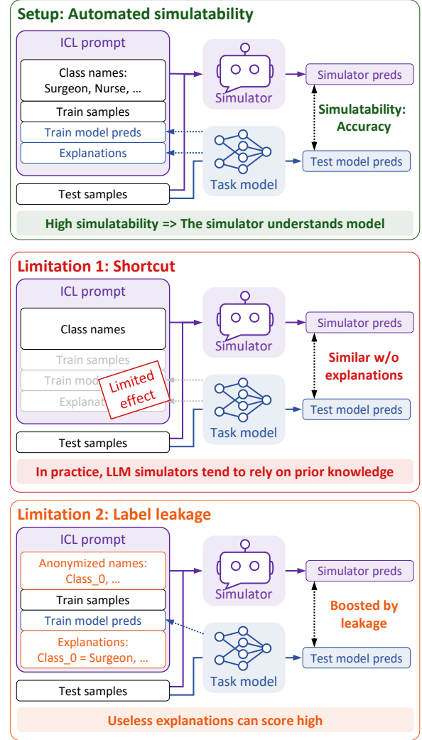
Figure 1: Overview of automated simulatability limitations. Automated simulatability explains how a task model works via ICL (in-context learning), and the LLM simulator must simulate its predictions on new samples. In theory, simulatability measures the usefulness of explanations. However, simulator predictions can remain unaffected by explanations, thus relying on task priors (Sec. 4). In anonymized settings, explanation scores can also reward hidden label recovery (Sec. 5).
