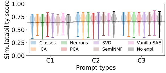
Figure 4: Non-anonymized concept prompts overlap. Qwen-3.5-9B grouped-seed scores for TopK new_consim C1–C3 prompts. The methods include qualitatively distinct concept decompositions, but their distributions largely overlap.
