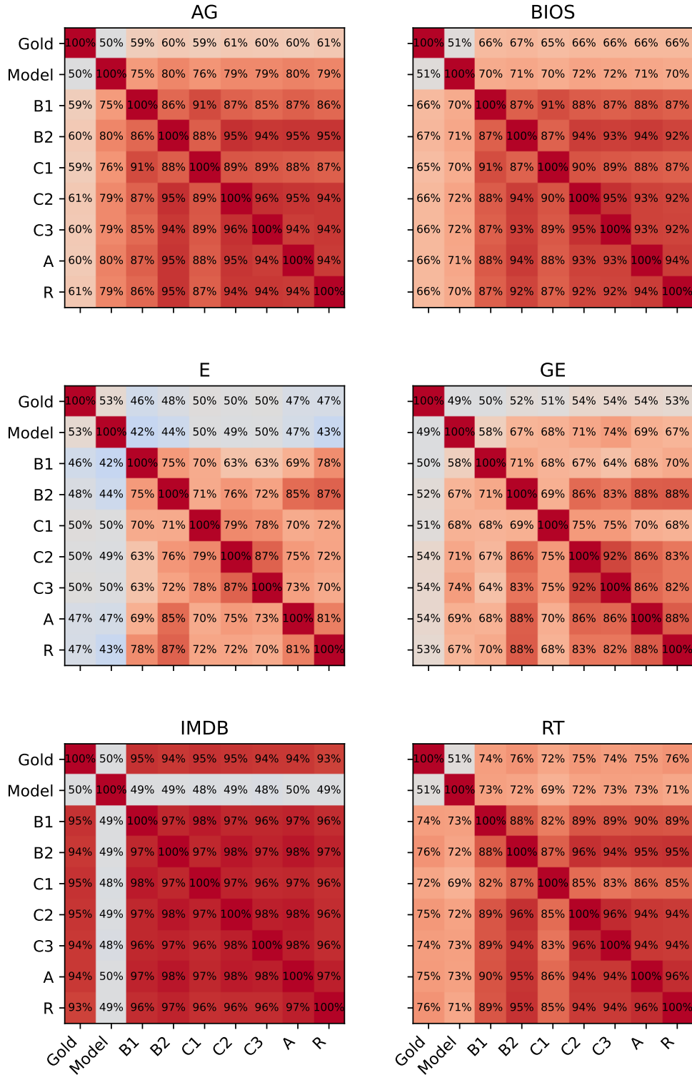
Figure 20: Qwen-3.5-9B prediction exact agreement by dataset. Exact agreement among gold labels, task model predictions, and selected prompt types, averaged equally over class subsets within each dataset.
