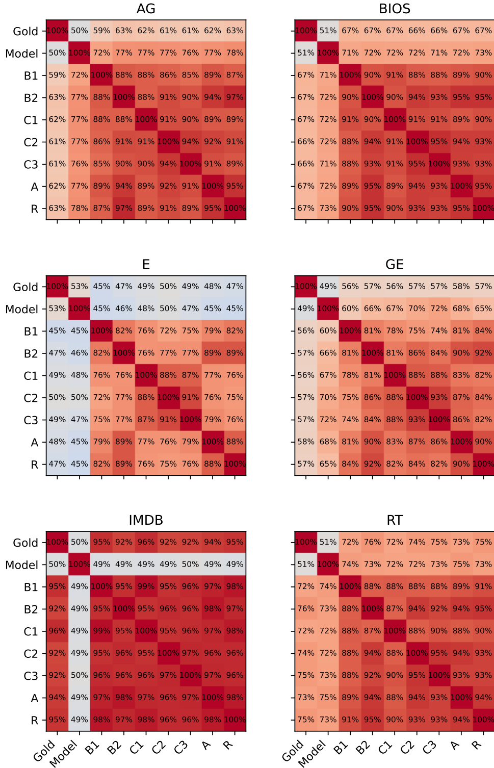
Figure 21: Gemma-4-12B prediction exact agreement by dataset. Exact agreement among gold labels, task model predictions, and selected prompt types, averaged equally over class subsets within each dataset.
