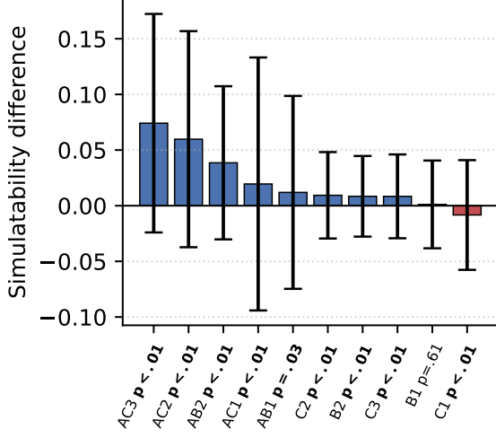
Figure 6: New- versus old-ConSim prompt format. Mean paired Qwen-3.5-9B score differences \text{new\_consim} - \text{old\_consim} . Positive bars favor the revised format.
