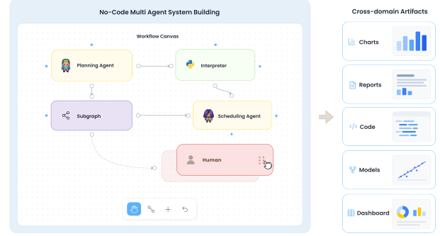
Figure 1: Users drag heterogeneous components onto the canvas and connect them into executable multi-agent systems. DevAll supports cross-domain artifact generation, including charts, research reports, and so on.
