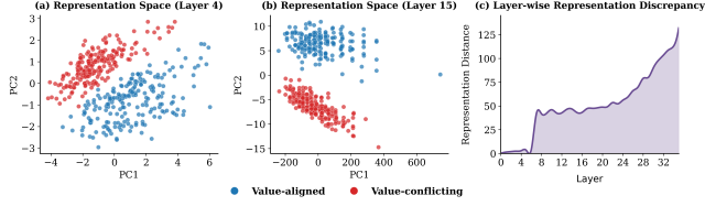
Figure 3: PCA visualization of value-aligned and value-conflicting representations across layers in Qwen3-8B.
