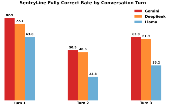
Figure 5: FC rates (%) of SENTRYLINE by conversation turn across three generation backbones on ASCOBENCH.
