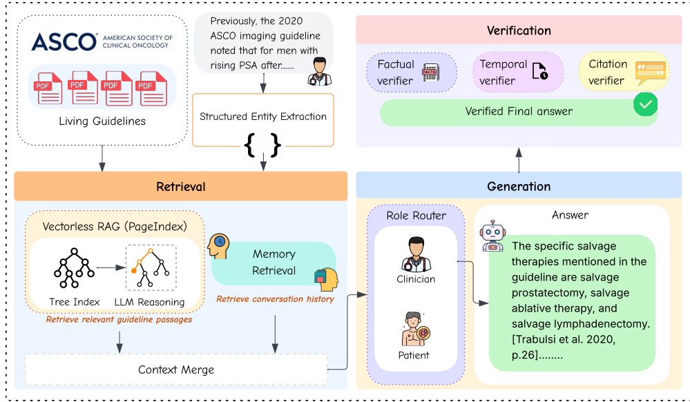
Figure 1: Overview of the SentryLine architecture. The system operates in three stages: (1) Retrieval, where structured entity extraction and a vectorless hierarchical index (PageIndex) retrieve relevant ASCO guideline passages and merge them with prior conversation history; (2) Generation, where a role router produces a clinician- or patient-facing answer with inline citations; and (3) Verification, where independent factual, temporal, and citation verifiers check the answer before it reaches the user.
