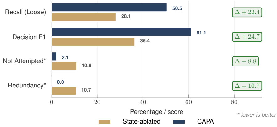
Figure 6: Meeting-state ablation, grouped bar view of Table 8.
