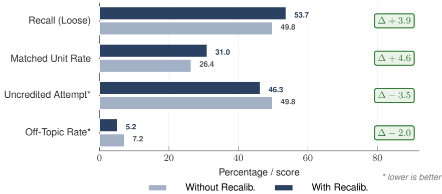
Figure 7: Recalibration ablation, grouped bar view of Table 9.
