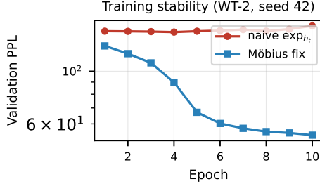
Fig. 2. Validation perplexity per epoch on WikiText-2 (seed 42): naïve \exp_{h_t} recurrence vs. Möbius HypRiLM.
