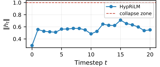
(c) State norm (HypRiLM)
