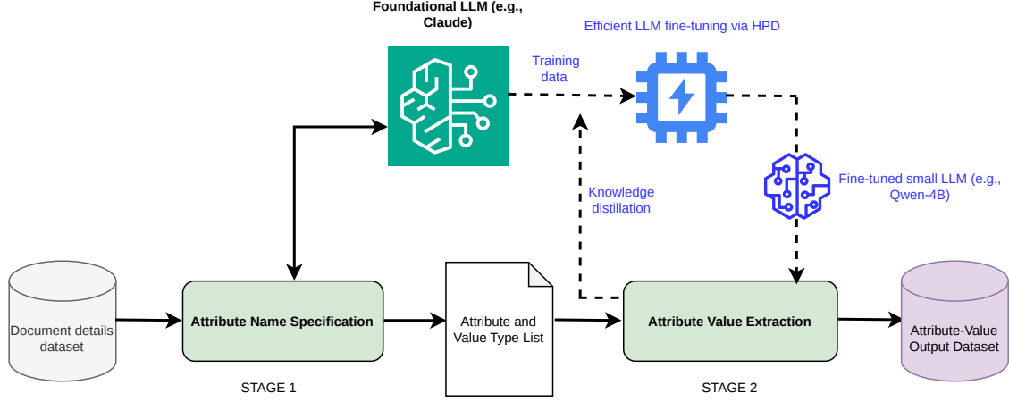
Figure 1: Overview of our two-stage pipeline for scalable schema-guided attribute value generation. Stage 1 discovers a compact schema of N purchase-discriminative attributes per category using a large foundational LLM. Stage 2 extracts attribute values from product catalog text using a fine-tuned compact LLM with Hyper-Parallel Decoding, generating all N values simultaneously.
