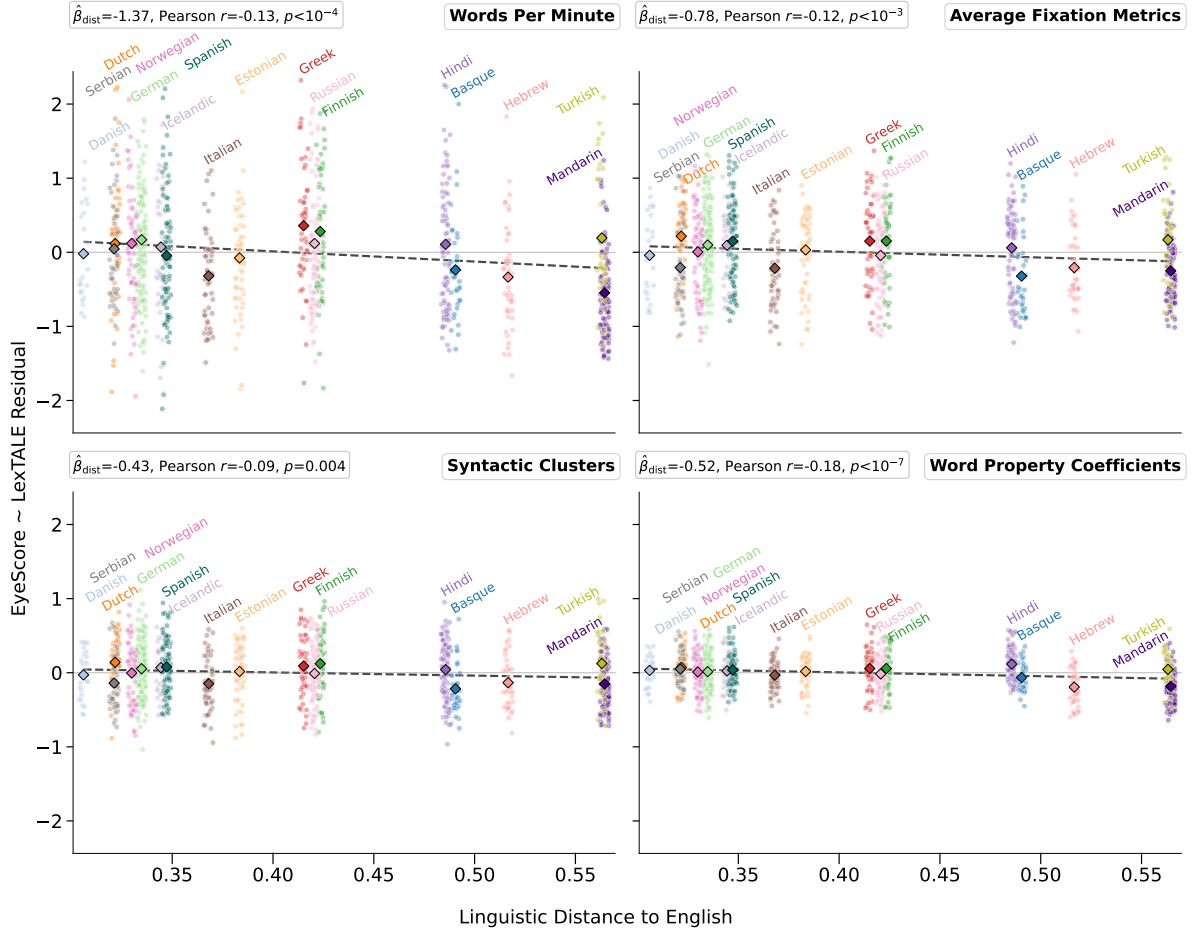
Figure 2: L1-English Proximity Bias in EyeScore, MECO L2. Residuals of an EyeScore \sim LexTALE regression as a function of the linguistic distance of the participant's L1 to English, in the Any Text regime.
