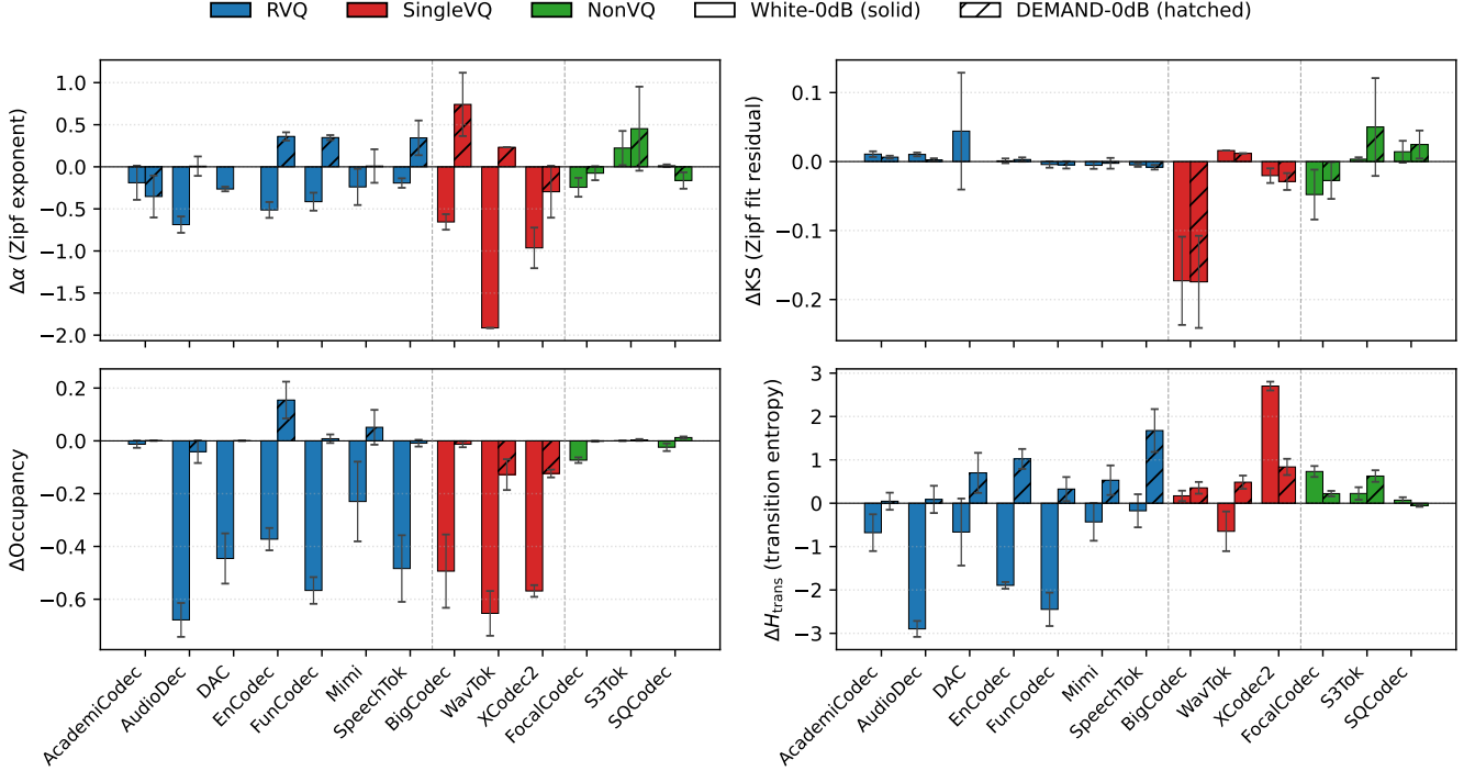
Fig. 6: Per-codec clean-to-noise shifts in the Zipf exponent, KS distance, codebook occupancy, and transition entropy (Section VIII-A) under the two 0dB conditions (solid: white; hatched: DEMAND). Bars show means across the three corpora and error bars the standard deviation; colors denote the quantizer meta-category, and dashed vertical lines separate the meta-categories.
