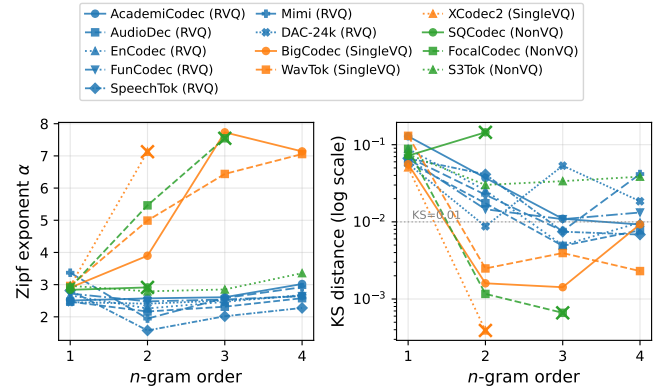
Fig. 3: Effect of n -gram order on the Zipf exponent \alpha and KS fit quality, averaged over three clean corpora. For codecs whose higher orders fail the V/N validity criterion the sweep terminates early; the last valid order of such series is marked with \times .
