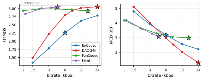
Fig. 7: Clean-speech UTMOS and MCD versus bitrate for the four RVQ codecs whose bandwidth is an inference-time choice. Stars mark the configurations evaluated in this paper, and the dashed line gives the UTMOS of the reference.
