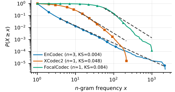
Fig. 4: Empirical complementary CDFs of the n -gram type frequencies (solid, with markers) and fitted power laws above x_{min} (dashed) for one representative codec per meta-category on clean LJSpeech at the 500K-token reference; larger KS corresponds to larger visible departure from the fitted line.
