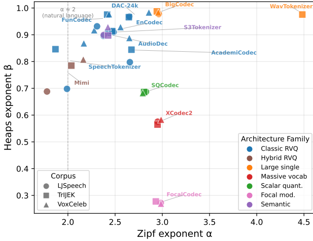
Fig. 5: Clean-speech Zipf exponent \alpha and Heaps exponent \beta for 13 codecs on LJSpeech, VoxCeleb, and TriJek at the 500K-token reference scale. Colors denote the architecture families of Table I. Cells without a defined power-law fit ( V/N > 0.9 ) are omitted.
