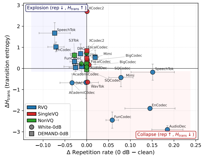
Fig. 9: Per-codec shifts from clean speech to the 0dB conditions in repetition rate and transition entropy, averaged across the three corpora. Colors denote quantizer meta-category and markers the noise type; shaded quadrants indicate the collapse and explosion signatures.
