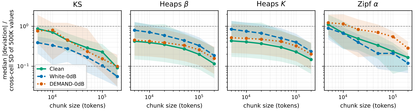
Fig. 2: Finite-sample stability across the 114 codec–corpus–condition cells with a matched 500K-token reference. Lines and shaded regions show the median and interquartile range of the absolute deviation from that reference (absolute log-ratio for K ), normalized by the cross-cell standard deviation of the reference values so that the four panels share one scale. Dashed guides mark deviations of 0.1 and 1.0 times that spread.
