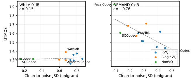
Fig. 8: Clean-to-noise JSD at the common unigram order versus UTMOS under the corresponding noisy condition, for the twelve decodable codecs averaged across the three corpora. Dashed lines are least-squares fits; r is the Pearson correlation reported in Table X.
