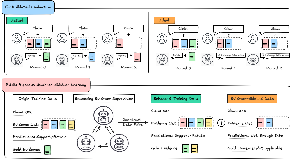
Figure 2: Illustration of proposed evaluating framework FAE (Top) and training framework REAL (Bottom)
