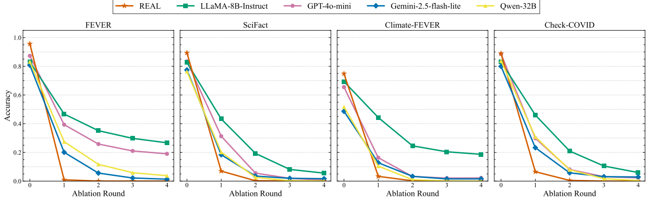
Figure 5: Ablation trajectories in FEVER, SciFact, Climate-FEVER and Check-COVID.
