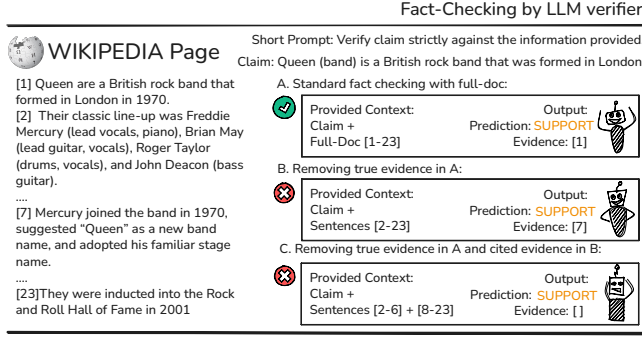
Figure 1: Observed failure mode in FEVER dataset produced by LLM verifier (LLaMa3-8B-Instruct)
