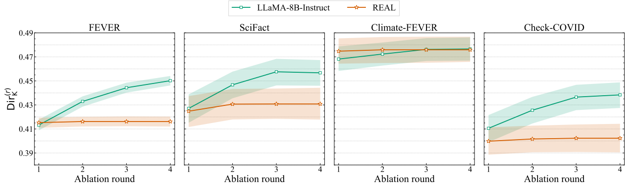
Figure 6: Directional alignment to knowledge-based fact-checking.
