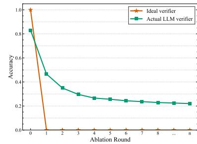
Figure 3: Ideal vs. actual ablation trajectories for claims annotated as SUPPORT/REFUTE (Llama-3.1-8B-Instruct on FEVER).
