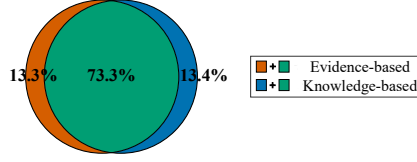
Figure 4: Comparison of activated neuron sets in fact checking using internal knowledge and provided evidence.
