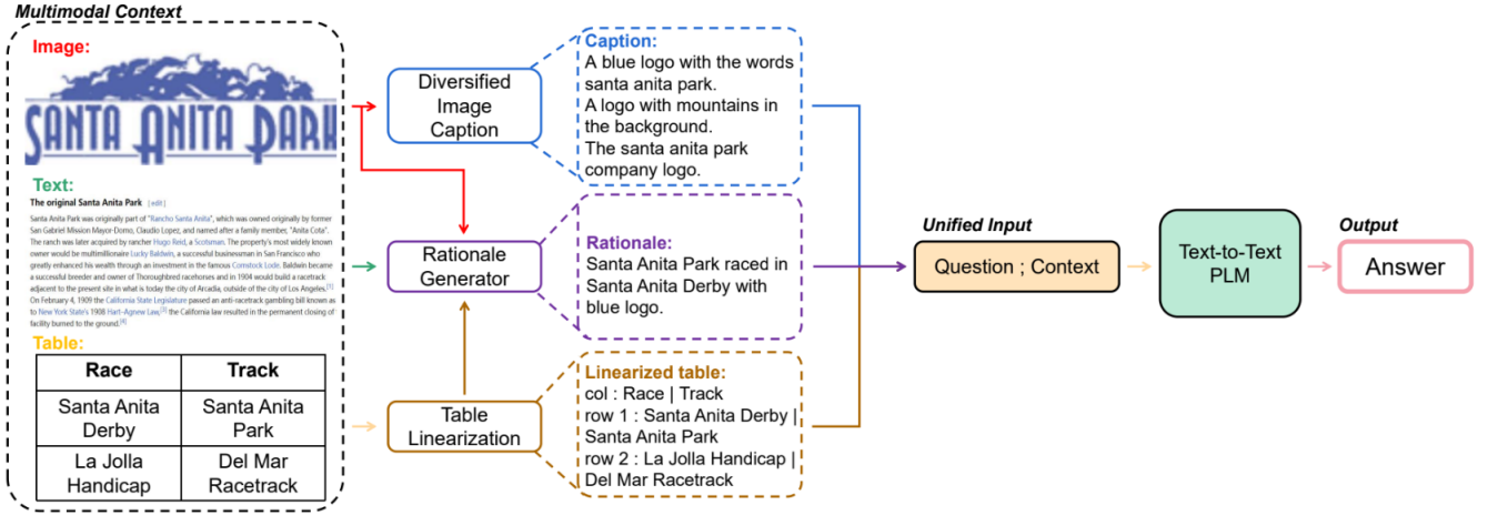
Fig. 3: Visualization of UniMMQA Pipeline [8].
