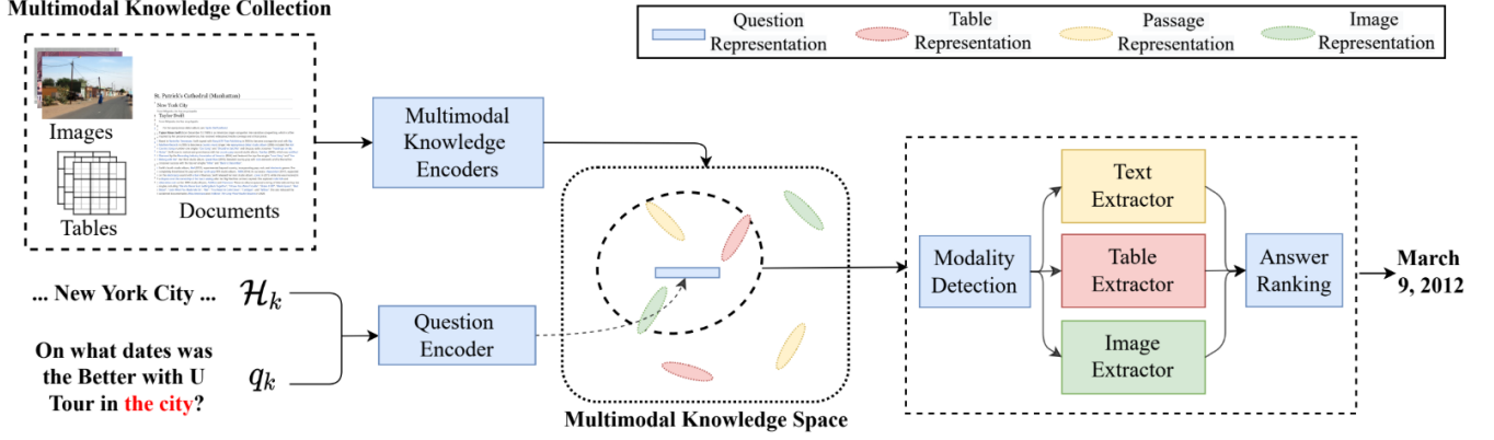
Fig. 1: Visualization of Multimodal Adaptive Extraction (MAE) Pipeline [6].
