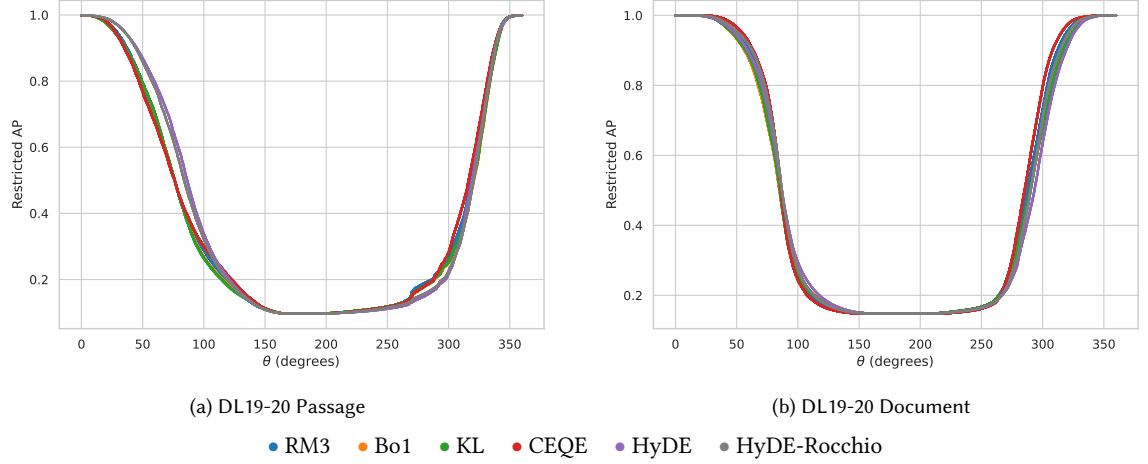
Fig. 5. Variation in Restricted AP along great circles originating from \mathbf{Q}_{IEQ}^{LS} ( \lambda = 0.1 ) and passing through 500 synthetic queries generated from expanded queries produced by RM3, Bo1, KL, CEQE, HyDE, and HyDE-Rocchio.
