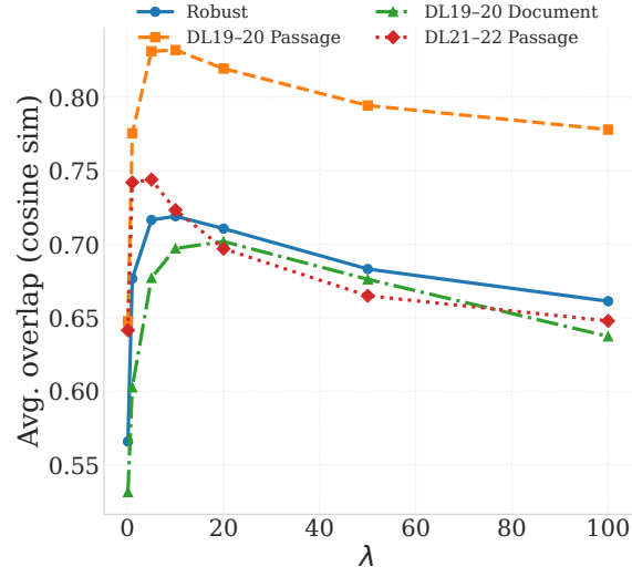
Fig. 13. Relationship between the average overlap with DFO based ideal query the LS based ideal queries generated with different \lambda .
