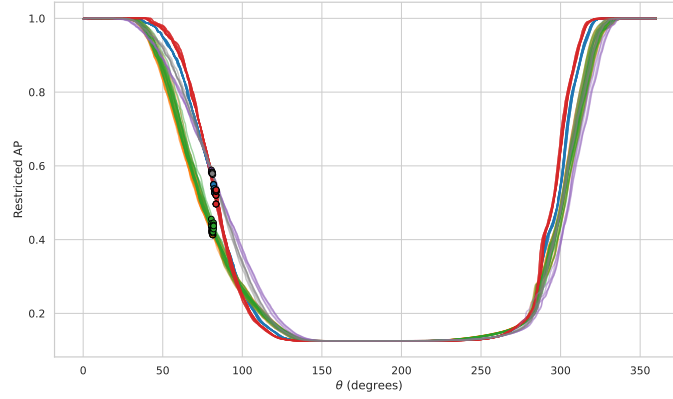
Fig. 6. Query-specific variation (only for qid 730539 of the DL19-20 Document collection) of Restricted AP along 90 great circles (originating from \mathbf{Q}_{IEQ}^{LS} ( \lambda = 0.1 ) and passing through 90 real expanded versions, generated using RM3, Bo1, KL, CEQE, HyDE, and HyDE-Rocchio methods, at different parameter settings).
