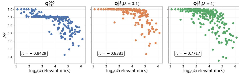
Fig. 1. Per-query scatter plots of AP versus the number of relevant documents for three different ideal-query formulations on the Robust collection. The Spearman rank correlation coefficient r_s between these two variables is reported in each plot.
