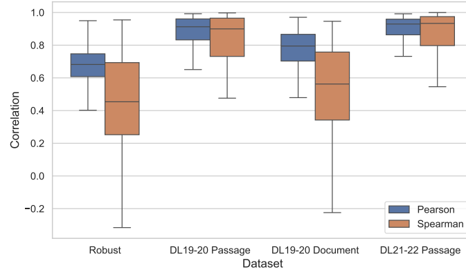
Fig. 2. Box plot of Pearson and Spearman correlations between the similarity of synthetically generated expanded queries to the ideal query Q_{IEQ}^{LS} (\lambda = 0.1) and their retrieval effectiveness across all collections.
