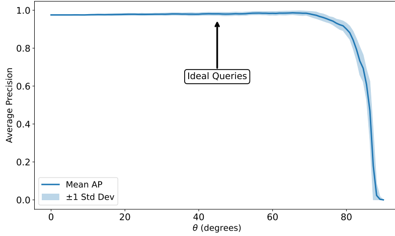
Fig. 3. Y-axis shows the AP variation and the X-axis plots the angle from the ideal query vector for the synthetically generated versions of the query ‘black bear attacks’ (Robust qid: 336).
