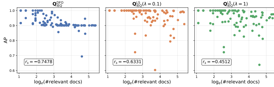
Fig. 9. Per-query scatter plots of AP versus the number of relevant documents for different ideal-query formulations on the DL19-20 passage collection. The Spearman rank correlation coefficient r_s between the two variables is reported in each plot.
