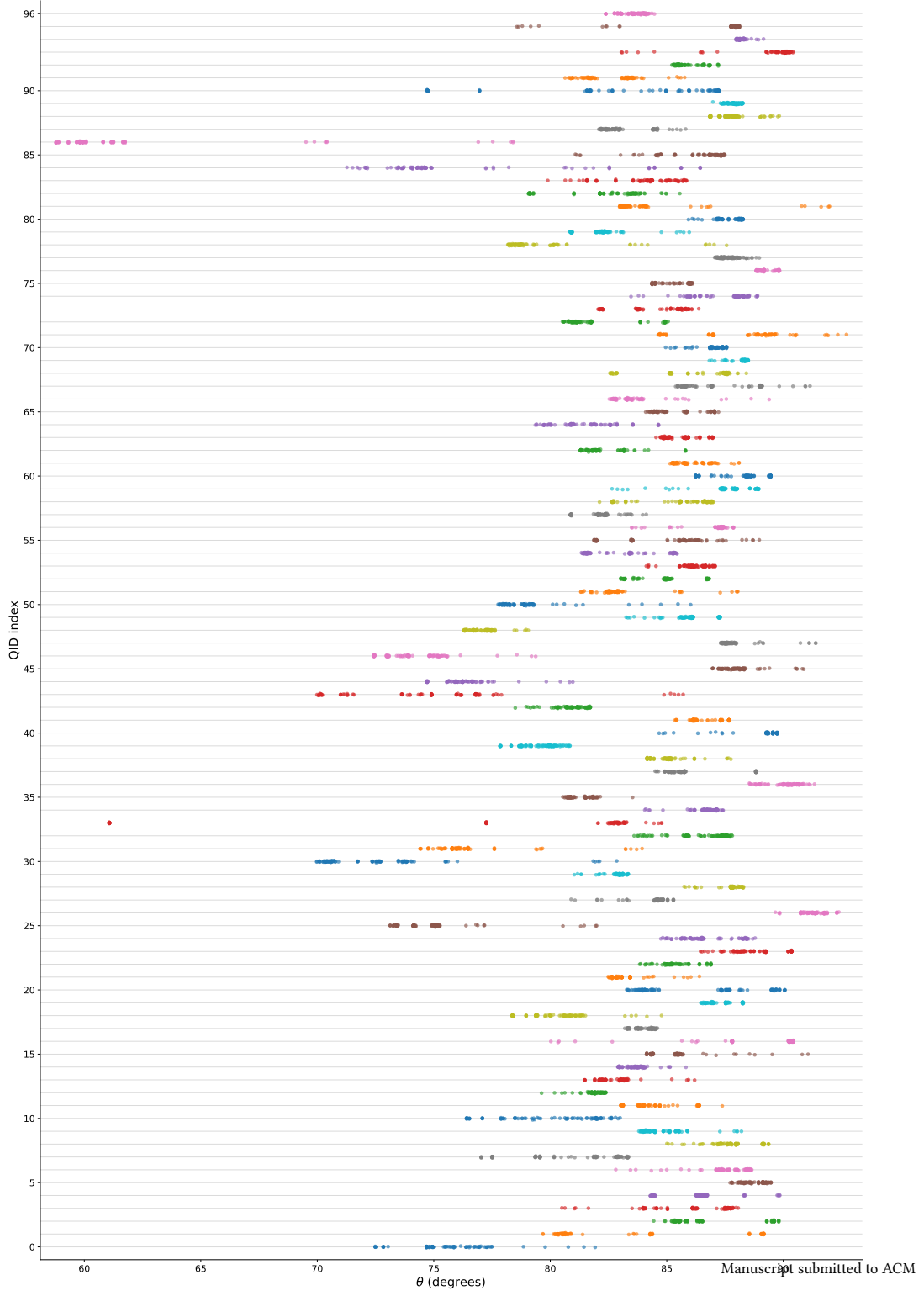
Fig. 8. Per-query variation in angular distance from Q_{IEQ}^{LS} (\lambda = 1) across different expanded queries (RM3, Bo1, KL, CEQE, HyDE and HyDE-Rocchio) for the benchmark queries in the DL19–20 Passage collection.
