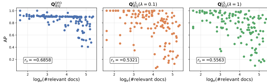
Fig. 11. Per-query scatter plots of AP versus the number of relevant documents for different ideal-query formulations on the DL21-22 passage collection. The Spearman rank correlation coefficient r_s between the two variables is reported in each plot. One outlier query is removed.
