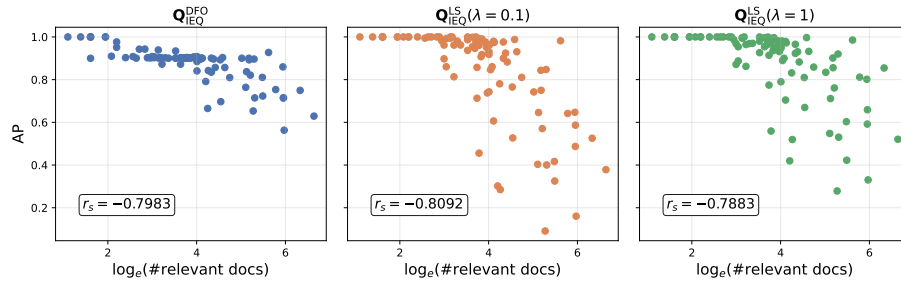
Fig. 10. Per-query scatter plots of AP versus the number of relevant documents for different ideal-query formulations on the DL19-20 document collection. The Spearman rank correlation coefficient r_s between the two variables is reported in each plot.
