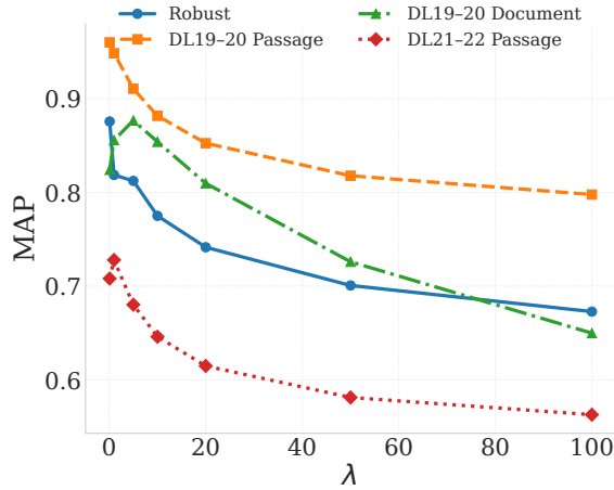
Fig. 12. Relationship between the MAP values and \lambda for LS based ideal queries.
