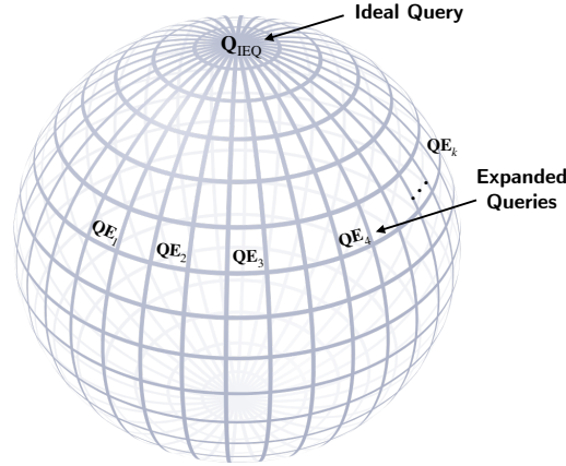
Fig. 4. Trajectories along the great circles constructed from Q_{IEQ} and each Q_{exp} , along which synthetic queries are generated.
