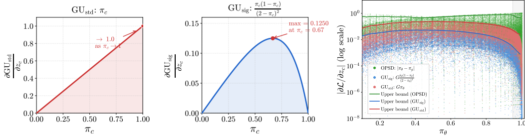
Figure 7: (Left and Mid) Comparison of the variations of two types of gradients by probability. (Right) The real gradient distribution in 100 training samples. OPSD tends to assign larger gradients to high-probability tokens, making the model more prone to drastic updates. In contrast, compared to the vanilla unlikelihood loss, our GU objective further suppresses the gradients on high-probability tokens.
