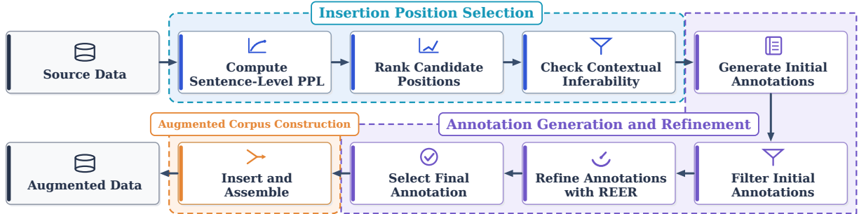
Figure 2 Overview of the REER-PT pipeline. REER-PT ranks candidate insertion positions by sentence-level perplexity, filters them by contextual inferability, generates and refines annotations using continuation perplexity, and inserts the selected annotations into the source documents.
