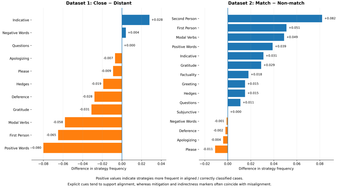
Figure 3: Strategy-level differences between aligned and misaligned cases across the two evaluation settings. Positive values indicate strategies more frequent in aligned or correctly classified cases.
