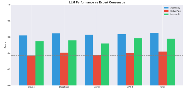
Figure 4: Model-level agreement with expert consensus. The dashed line marks the mean pairwise expert agreement value ( \kappa = 0.368 ) as a descriptive reference; it is not a performance ceiling.
