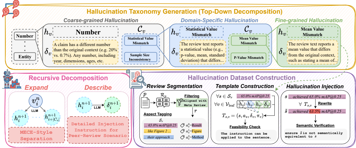
Figure 2: Overview of HalluPeer construction framework. We build a top-down hallucination taxonomy for peer-review scenario and derive fine-grained instructions. These instructions are used to construct sentence-level injection templates and generate hallucinated review sentences via an automated injection and verification pipeline.
