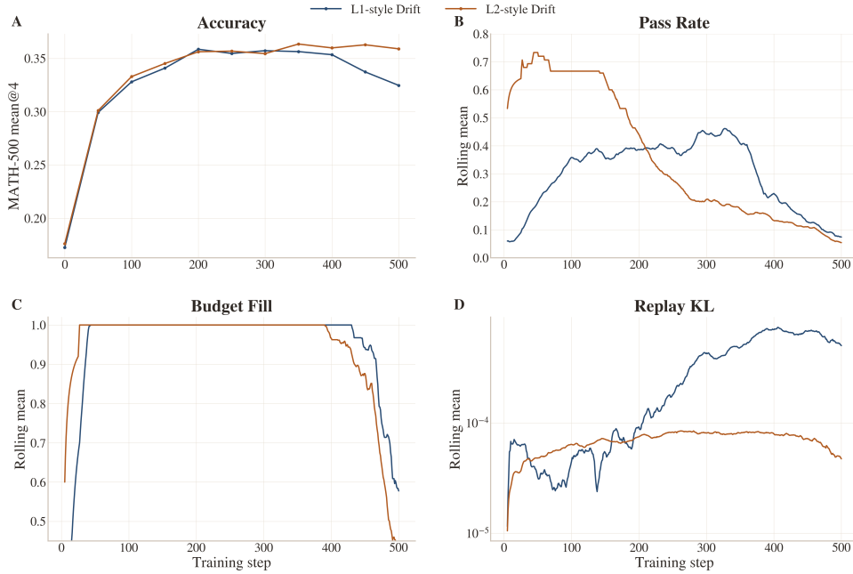
Figure 19: Step-aligned comparison of L1-style and L2-style Drift gating. L2 attains better late-stage validation accuracy while maintaining lower replay mismatch, despite matched or lower replay-budget fulfillment.
