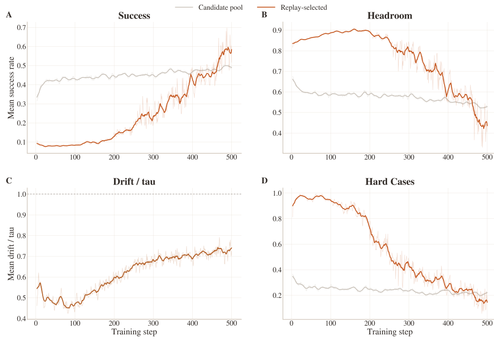
Figure 20: Aggregate properties of the replay groups selected by L2-style Drift gating. Early training concentrates replay on hard, high-Headroom groups; later training moves toward the remaining frontier, and replay usage contracts as that frontier is depleted.
