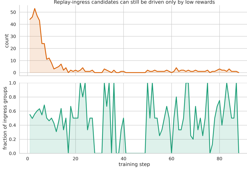
Figure 9: The count and fraction of groups that can enter the replay buffer under the original ingress rule while containing only 0.0 and 0.1 rewards. Such groups contain no answer-correct samples at all, and their within-group reward variation is driven entirely by formatting rather than answer correctness. As the figure shows, these groups are not confined to the very early stage of training, but continue to appear as ingress candidates well into the middle and later stages.
