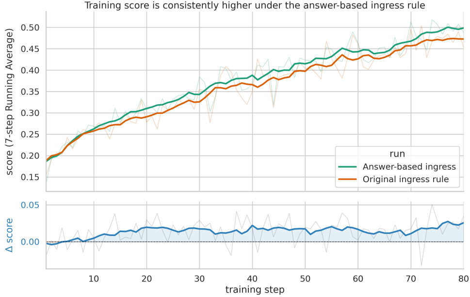
Figure 10: Comparison of training-score trajectories under the original ingress rule and the answer-based ingress rule over the shared early-stage window. The top panel shows the raw trajectories (faint) together with their running averages (bold), while the bottom panel shows the score difference between the two runs over the same window.
