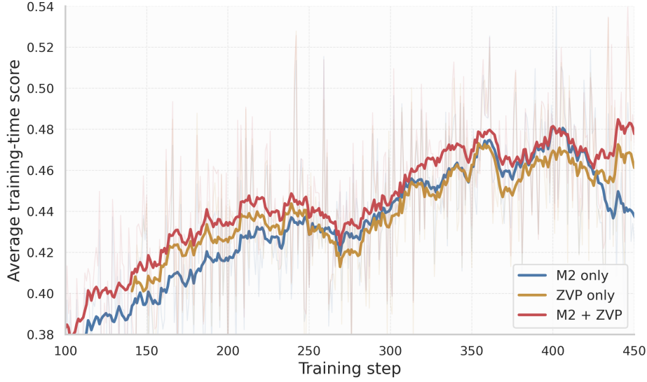
Figure 24: Training-score curves for the mathematical-reasoning component ablation. In the figure legend, M2 denotes Policy Drift only, ZVP denotes Headroom only, and M2 + ZVP denotes full Headroom-Drift Replay.
