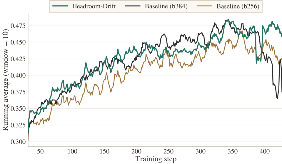
Figure 25: Training-score trajectories under a CISPO-style objective. Headroom-Drift denotes full Headroom-Drift Replay (b256+r128). Baseline (b256) is the on-policy matched control; Baseline (b384) is the on-policy larger control. Running average with window 10.
