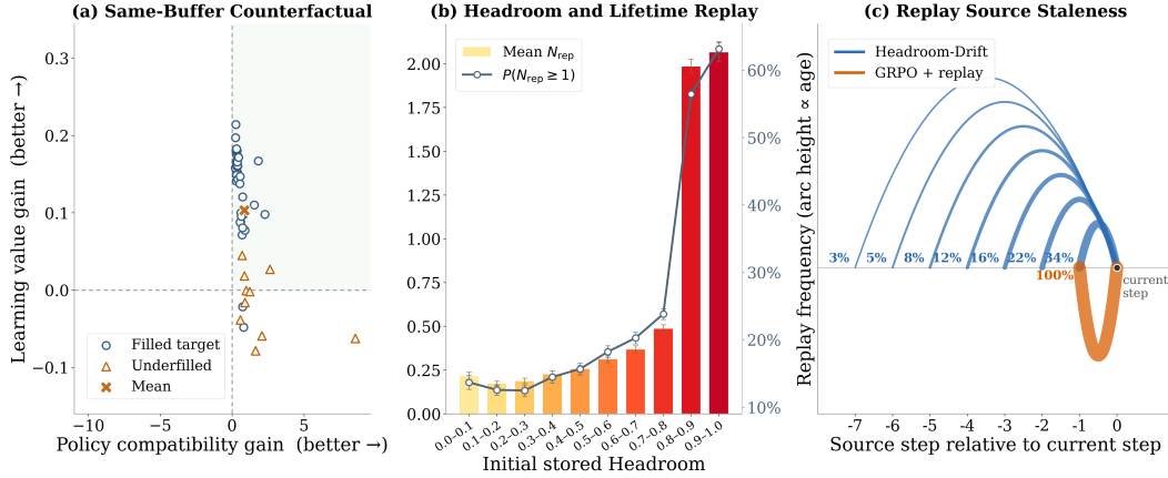
Figure 5: (A) Same-buffer counterfactual against GRPO + replay. (B) Initial stored Headroom and lifetime replay. Bars show mean replay count N_{\text{rep}} , and the line shows P(N_{\text{rep}} \geq 1) . (C) Conceptual view of replay source staleness under Headroom-Drift versus GRPO + replay.
