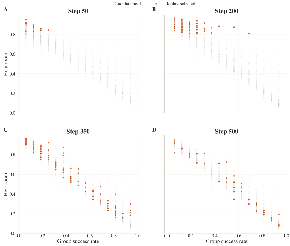
Figure 21: Selection snapshots in the success-rate / Headroom plane at four training stages. Selected groups (orange) concentrate near the upper-left frontier of the candidate cloud (gray), particularly in early and middle training.
