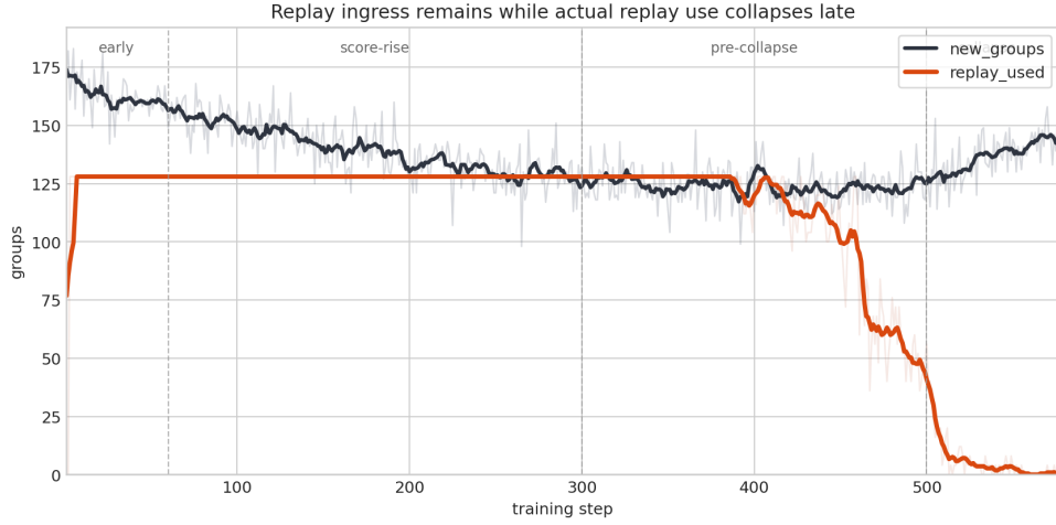
Figure 17: Replay ingress and actual replay use over training. The gray curve shows the number of newly ingressed groups added to the replay buffer at each step, while the orange curve shows the number of replay groups actually used for the update. Although ingress remains substantial into the late stage, actual replay use drops sharply near collapse, suggesting that the late-stage transition is better understood as a contraction of the usable replay subset rather than as a simple ingress collapse.
