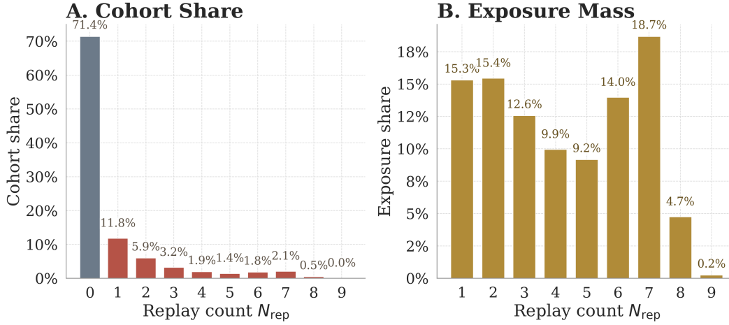
Figure 15: Replay multiplicity and exposure concentration. (A) Cohort share by lifetime replay count N_{\text{rep}} , showing what fraction of groups are replayed 0, 1, 2, ... times. (B) Exposure-mass share by lifetime replay count, showing what fraction of total replay-use events comes from each N_{\text{rep}} cohort. Most groups are never replayed, but a much smaller subset of repeatedly reused groups accounts for a disproportionately large share of total replay exposure.
