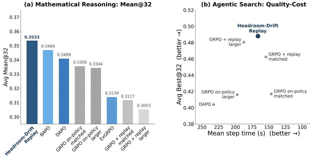
Figure 1: Summary of two representative views. (a) In mathematical reasoning, Headroom-Drift Replay leads on Avg Mean@32 over all baselines. (b) In agentic search, Headroom-Drift combines the highest Avg Best@32 with competitive wall-clock cost.
