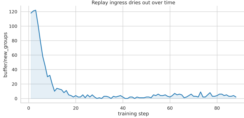
Figure 6: Declining replay-buffer ingress over the course of training in Geometry3K. The batch size is 128.
