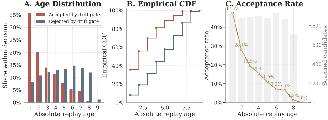
Figure 12: Replay age and Drift-gate compatibility in mathematical-reasoning. (A) Age histogram normalized separately within the accepted and rejected populations. (B) Empirical CDF of replay age for accepted and rejected candidates. (C) Age-conditioned acceptance rate, with the gray bars indicating the number of scanned candidates in each age bucket. Accepted replay is concentrated on younger groups overall, but the two age distributions overlap substantially, and rejection remains non-negligible even at the smallest replay ages. The raw tail counts at large ages are additionally constrained by finite FIFO turnover, so the age-conditioned acceptance rate in Panel (C) is the most direct view of compatibility.
