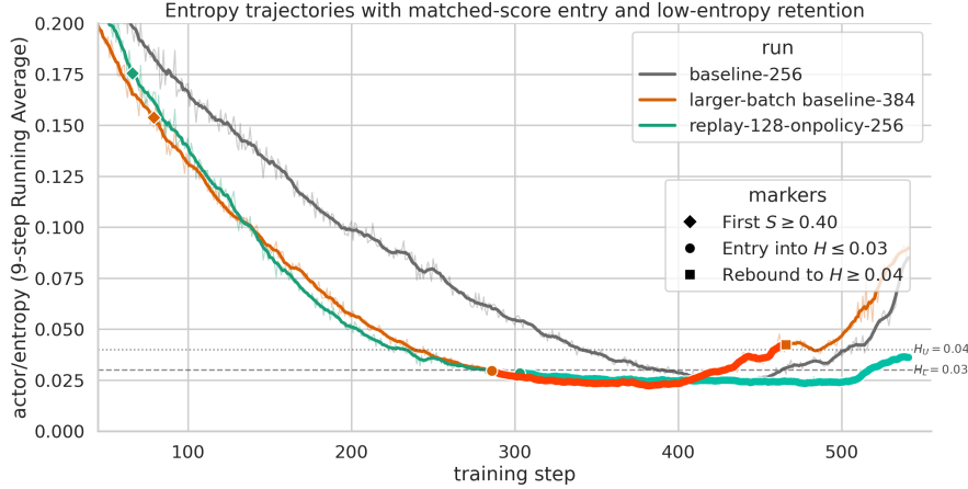
Figure 16: Entropy trajectories for the three runs. The gray GRPO on-policy matched (b256) is shown only as a reference. Diamonds denote first arrival at the shared training-score anchor, circles denote entry into the low-entropy regime, squares denote rebound, and the highlighted segments indicate the retained low-entropy window.
