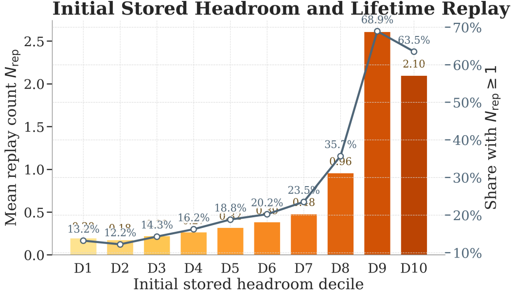
Figure 14: Initial stored Headroom and lifetime replay pressure. Bars show the mean lifetime replay count N_{\text{rep}} for groups in each initial stored-Headroom decile, and the line shows the probability that a group is replayed at least once. Higher initial stored Headroom is associated with both more frequent reuse and a higher probability of entering replay at least once, indicating a real Headroom-driven selection pressure rather than a purely definitional score.
