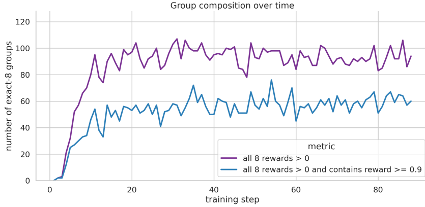
Figure 7: Comparison between the number of exact-8 groups in which all responses satisfy the original success indicator s_i^+ = \mathbf{1}[r_i > 0] and the number of such groups that contain at least one answer-positive response ( a_i = 1 \iff r_i \geq 0.9 ). Under the s_i^+ -based definition, all such groups are treated uniformly as all-success groups, even though they differ in whether they contain answer-correct responses.
