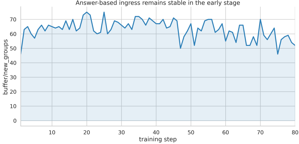
Figure 11: Number of groups newly entering the replay buffer under the answer-based ingress rule during the shared early-stage window. Despite the stricter criterion, replay ingress remains sufficiently active and does not collapse prematurely.
