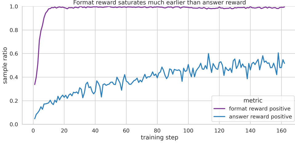
Figure 8: Format reward saturates much earlier than answer reward in Geometry3K.
