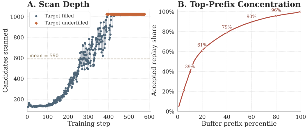
Figure 13: Headroom-ordered prefix truncation in practice. (A) Actual scan depth per training step, measured as the number of buffered candidates examined before replay selection terminates. Blue circles indicate steps that filled the replay target, and orange diamonds indicate underfilled steps. (B) Cumulative share of accepted replay recovered from the top Headroom-ordered buffer prefix. Accepted replay is strongly concentrated near the top prefix of the Headroom-ordered buffer, but later training increasingly requires deeper scans because the Policy Drift gate becomes more selective.
