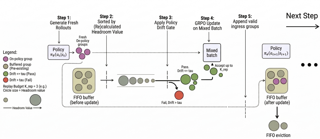
Figure 2: Headroom-Drift Replay in one GRPO step. The current policy generates fresh on-policy groups. Pre-existing buffered groups are ordered by Headroom and filtered by the Policy Drift gate; up to K_{\text{rep}} accepted replay groups are merged with the fresh groups to form the mixed batch for the GRPO update. After the update, fresh groups with non-identical rewards are appended to the FIFO replay buffer.
