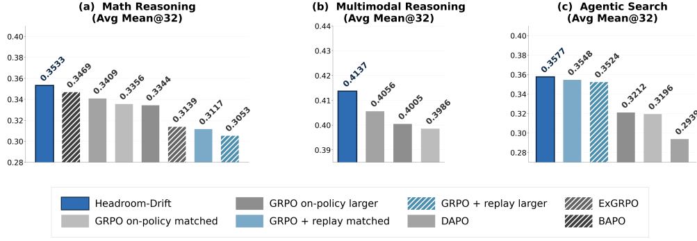
Figure 3: Cross-domain summary with Mean@32.
