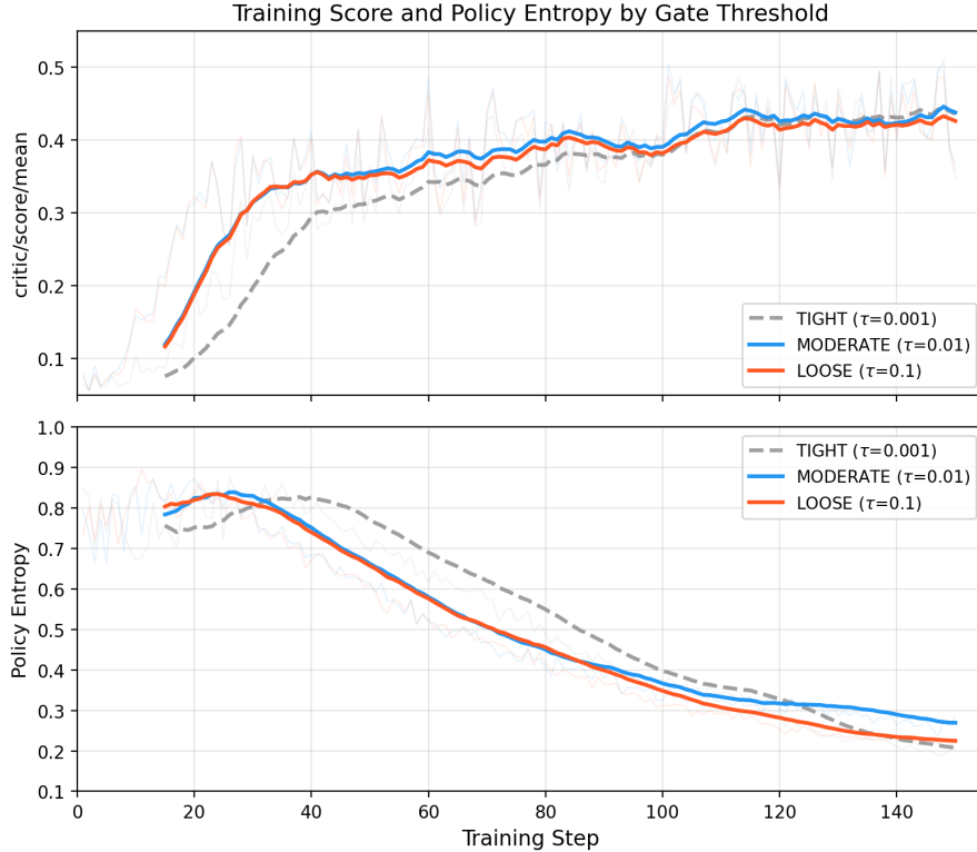
Figure 23: Training score (upper) and policy entropy (lower) over training for the three \tau conditions (running average, window = 15).
