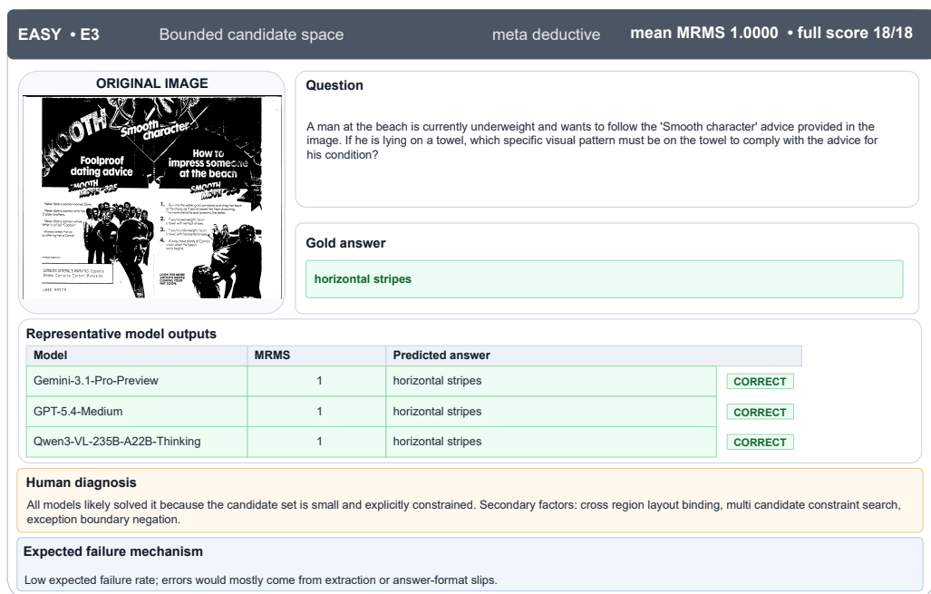
Figure 13: An easy E3 case illustrating a bounded candidate space and a deterministic decision in meta-deductive reasoning.
