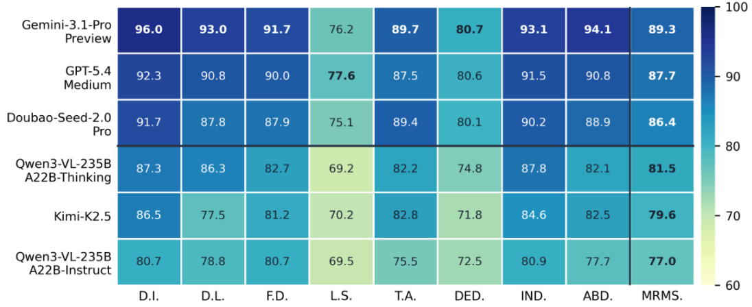
Figure 3: MRMS heatmap for the three highest-ranked closed-source and open-source models from Table 2.
