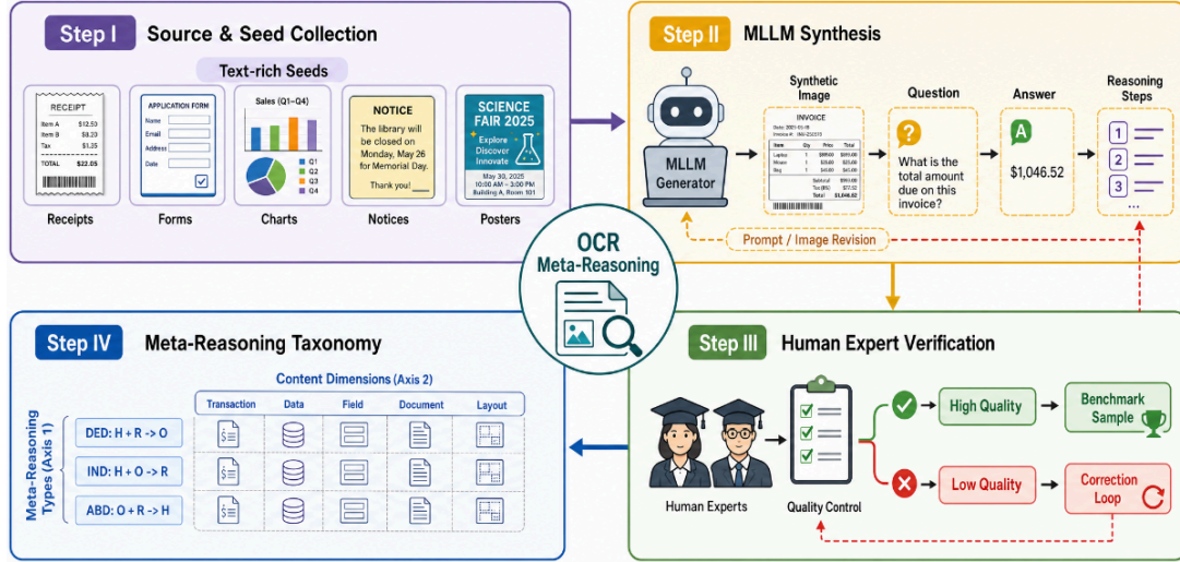
Figure 2: Overview of OCR-MetaReasoning construction. We collect text-rich seeds, synthesize OCR-grounded samples with MLLMs, assess candidates using taxonomy-aligned checklist criteria, and organize valid samples by meta-reasoning type and OCR-object category. We regenerate prompts or images when necessary.
