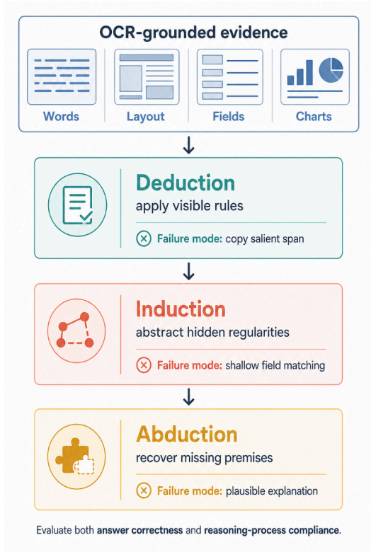
Figure 4: Abstract illustration of OCR-grounded meta-reasoning.
