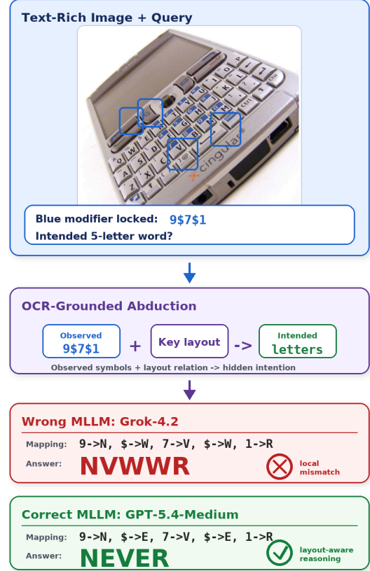
Figure 1: OCR-grounded abduction in OCR-MetaReasoning. The model infers the hidden intention behind “9$7$1” from the keyboard layout, contrasting local symbol matching with layout-aware reasoning.
