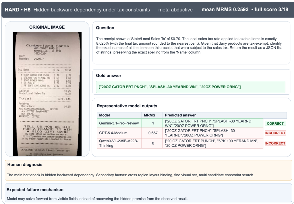
Figure 9: A hard H5 case illustrating hidden backward dependency under tax constraints in meta-abductive reasoning.
