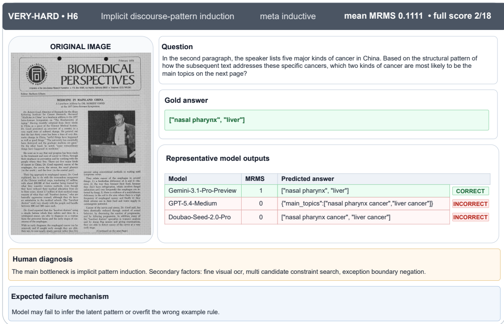
Figure 8: A very-hard H6 case illustrating implicit discourse-pattern induction in meta-inductive reasoning.
