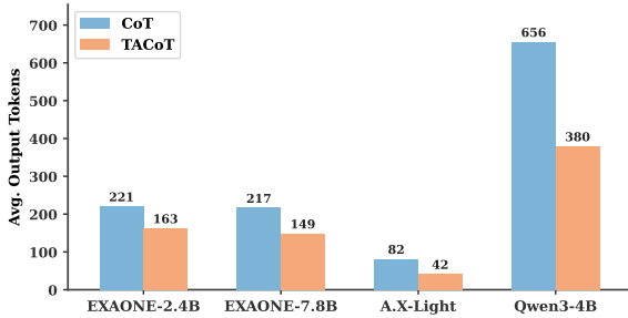
Figure 5: Average output tokens for CoT and TACoT across models. TACoT consistently reduces token cost while preserving most of the accuracy gains of CoT.
