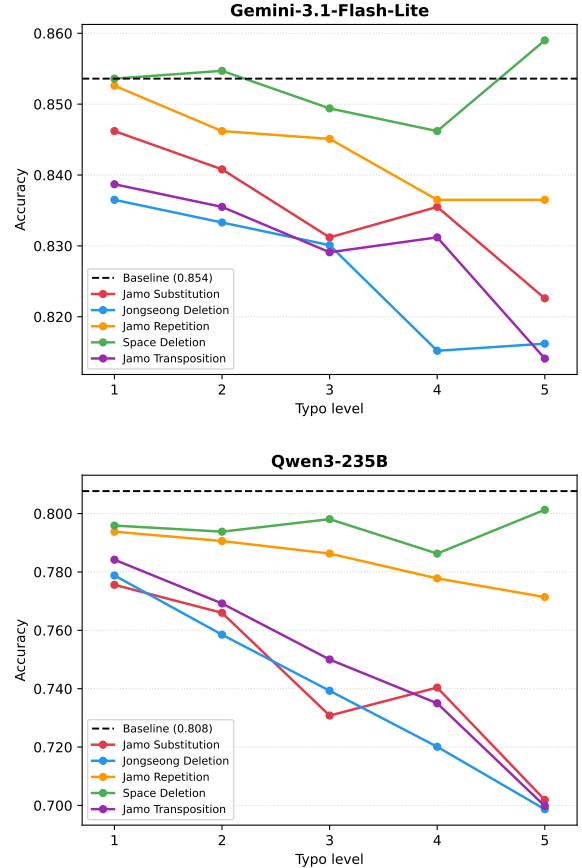
Figure 9: KMMLU accuracy under Korean typo perturbations for API-scale models. Dashed lines indicate clean baseline accuracy.
