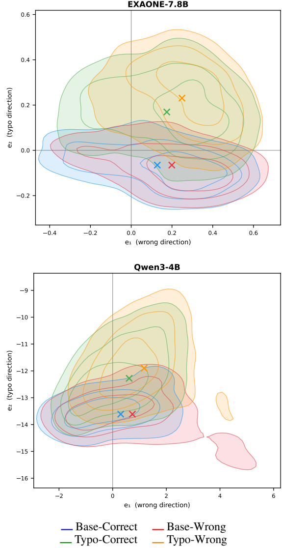
Figure 4: Direction projection of hidden states at the Fisher-selected layer. Full projections for all models are provided in Appendix F.
