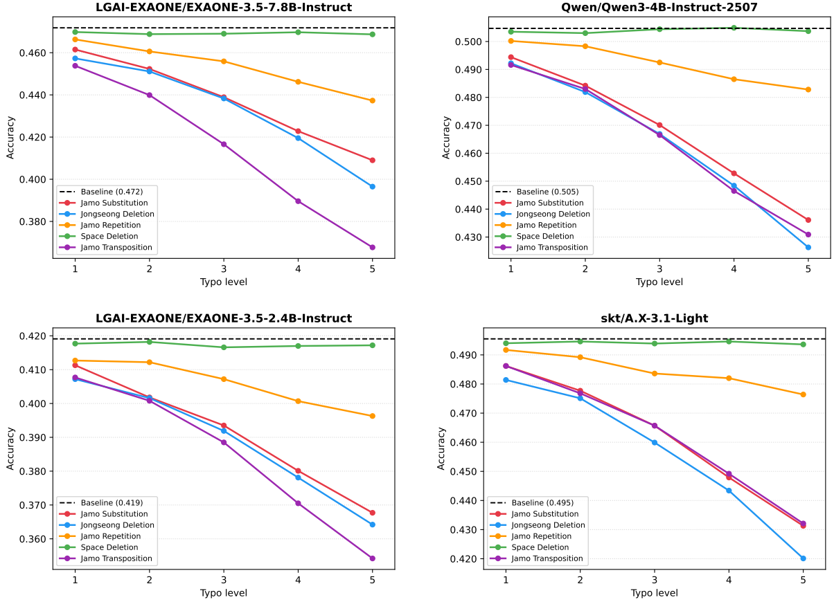
Figure 3: KMMMLU accuracy across five typo intensity levels for all four models. Dashed lines indicate clean baseline accuracy.
