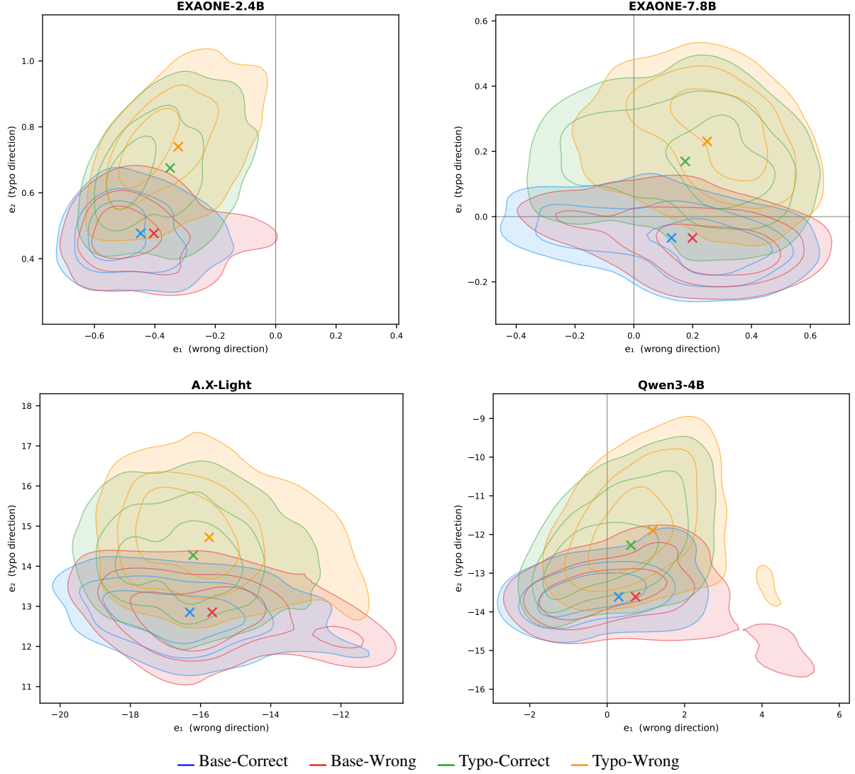
Figure 11: Full direction projections of hidden states at the Fisher-selected typo-sensitive layer for all evaluated models. The horizontal axis corresponds to the clean incorrectness direction, while the vertical axis captures the typo direction orthogonal to it.
