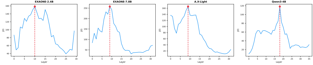
Figure 10: Layer-wise Fisher separation score J(l) between clean and typo hidden states. Dashed vertical lines indicate the selected typo-sensitive layer for each model.
