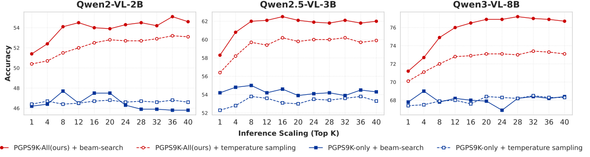
Figure 4: Impact of data diversity on test-time scaling across model sizes. Models trained on PGPS9K-All scale robustly with increasing sample budget, whereas the PGPS9K-only baseline shows limited gains or even degradation.
