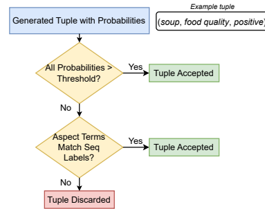
Figure 2: Inference algorithm.
