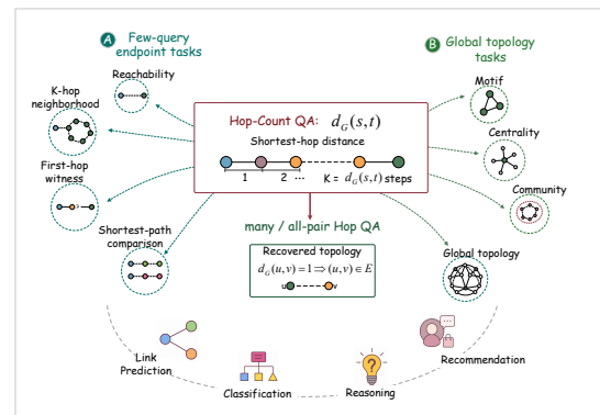
Figure 1: HopQA as a bounded topology diagnostic for testing graph-evidence use on the native generation surface.
