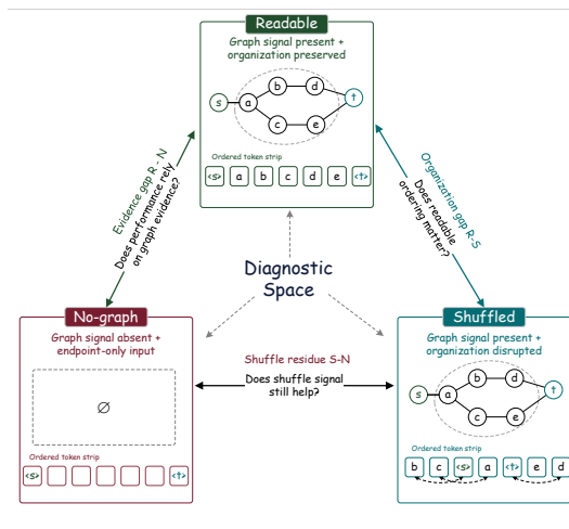
Figure 4: Intervention triangle for the readable, no-graph, and shuffled graph-token interfaces. The triangle shows how the three intervention conditions separate harmful-shuffle, shuffle-robust, and no-graph-saturated regimes.
