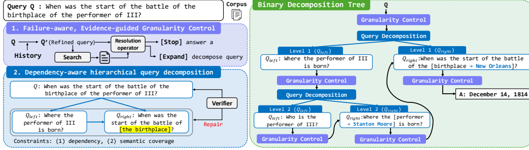
Figure 2: Overview of Hi-Q. Hi-Q treats multi-hop QA as evidence-conditioned search over query granularity. At each node, the resolution operator first tests whether retrieved evidence supports the current query unit. Resolved nodes terminate; unresolved nodes trigger dependency-ordered binary decomposition, where the prerequisite branch is resolved before the dependent branch. A semantic coverage verifier repairs invalid splits before recursion. The resulting binary decomposition tree is determined by corpus support signals rather than by a fixed graph or a predetermined decomposition template.
