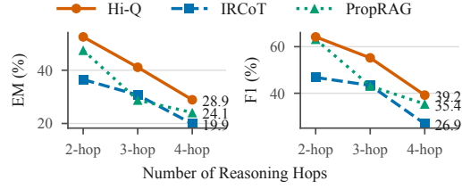
Figure 3: EM, F1 score across hop counts.
