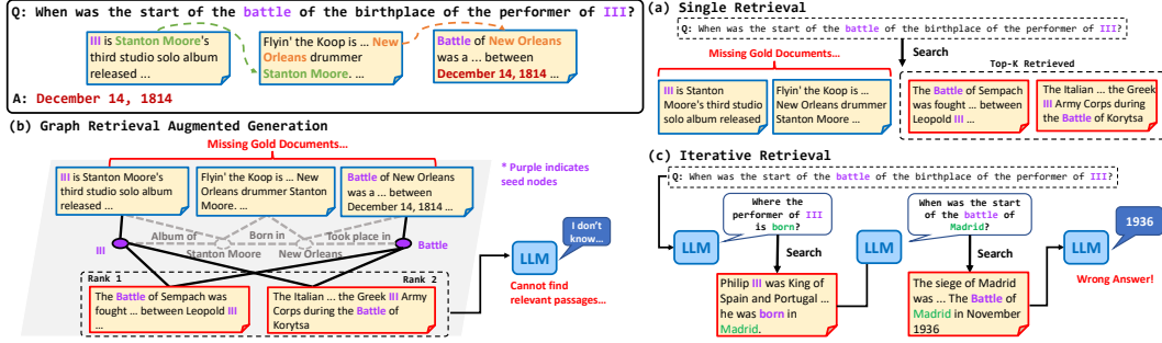
Figure 1: Granularity failures in multi-hop retrieval. (a) Single retrieval, (b) Graph RAG, and (c) iterative retrieval on the same query and corpus.
