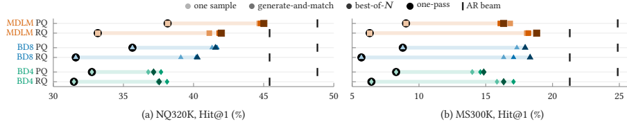
Figure 3: Every diffusion model gains over one sample, and none reaches AR’s beam. Each row: one diffusion model and identifier under four decodings (one sample, generate-and-match, best-of-N, one-pass), darker in that order (bar: their range). Black tick: AR’s beam on the same identifier.
