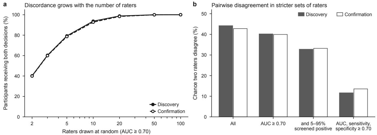
Extended Data Fig. 7: How disagreement depends on which raters are counted . a , Expected share of participants who receive both decisions from k raters with AUC \geq 0.70 drawn at random without replacement (exact), against k ; filled markers and solid line, discovery; open markers and dashed line, confirmation. b , Chance that two different raters disagree about a participant, among all raters, raters with AUC \geq 0.70 , those that also screen 5–95% of participants positive, and those with AUC, sensitivity and specificity all \geq 0.70 ; dark grey, discovery; white, confirmation. Exploratory analyses.
