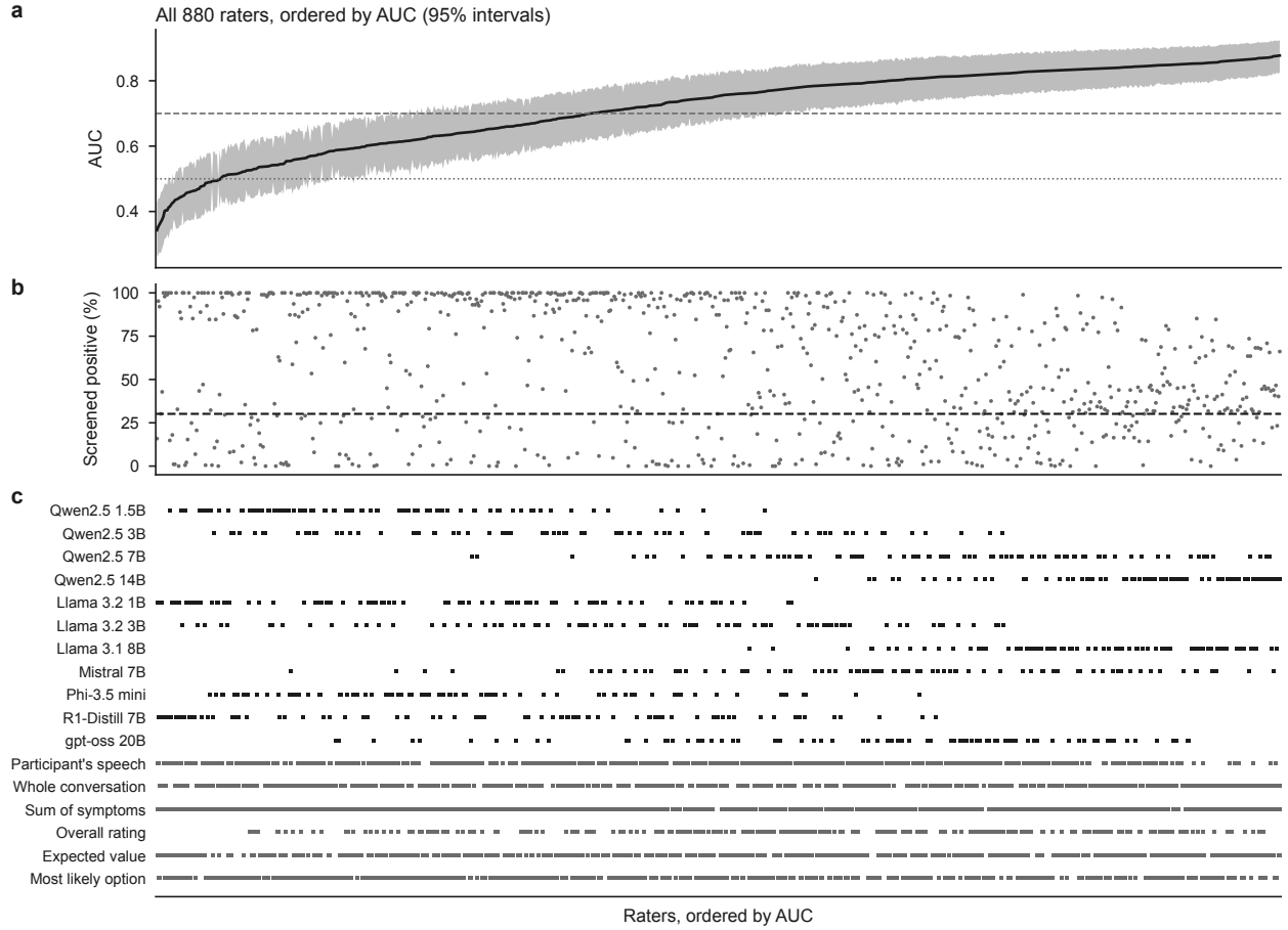
Extended Data Fig. 6: All raters, ordered by accuracy (discovery). a , AUC of every rater, ordered, with 95% bootstrap intervals; dotted line, chance; dashed line, 0.70. b , Share screened positive by the same raters; dashed line, self-reported prevalence. c , The choices that make up each rater.
