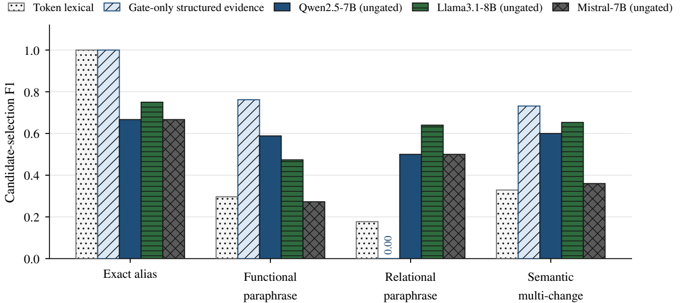
Figure 3. Candidate-selection F1 across the four semantic-challenge families, each containing 12 cases. Ungated LLMs exceed token lexical and gate-only on relational paraphrases; gate-only performs better on functional paraphrases and semantic multi-change requests. Family-level exact-set comparisons do not remain significant after Holm correction.
