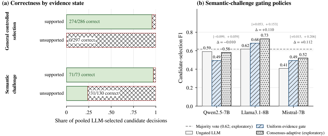
Figure 4. Deterministic evidence and exploratory gating. (a) Correctness of supported and unsupported ungated selections, pooled across three models. The general-and-safety group includes 120 cases; the semantic-challenge group includes 48. (b) Semantic F1 for ungated, uniformly gated, and consensus-adaptive selections. The dashed line marks three-model majority-vote F1. Printed values give the adaptive-minus-ungated F1 difference with its paired-bootstrap 95% confidence interval.
