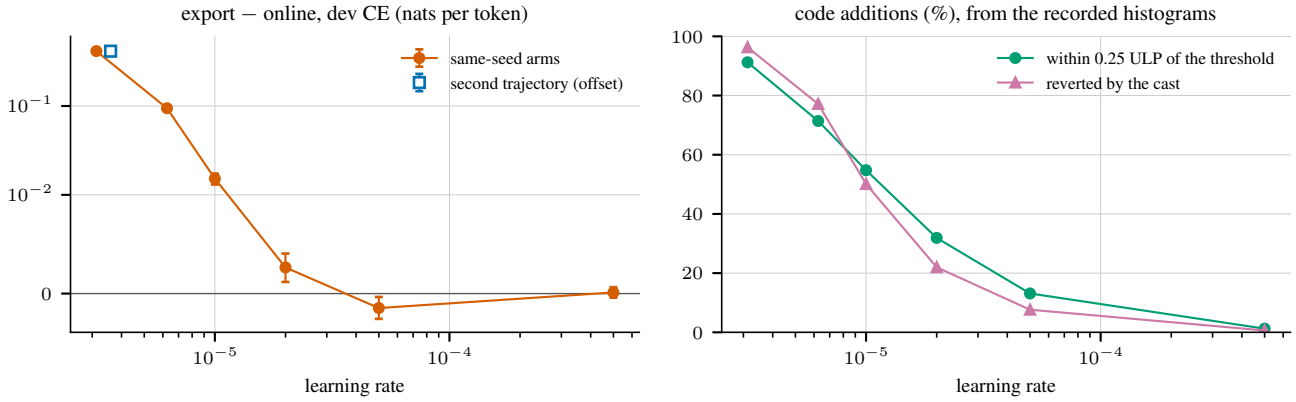
Figure 3. Falcon-E-1B-Base, the documented export across fine-tuning learning rates (fp32 latents, one trajectory per arm). Left: export minus online dev cross-entropy with 95% paired row-bootstrap intervals, on a symmetric log scale; the open square is the second trajectory at the lowest rate, offset horizontally for visibility. Right: descriptive summaries of each endpoint’s recorded margin histogram, the share of code additions within 0.25 bf16 ULP of the threshold and the share the cast reverts; they are counts, not measurements of latent displacement. Lines connect the declared rates for reading; no curve or between-rate difference was tested.
