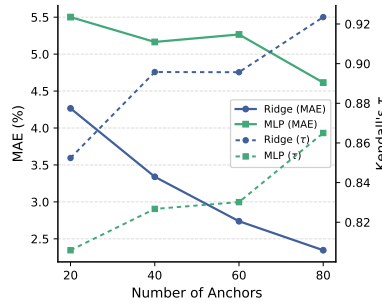
Figure 6 | Ablation on network architecture on BFCL.
