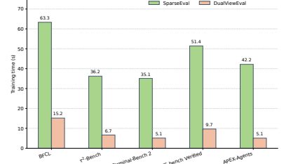
Figure 10 | Efficiency Analysis. DualViewEval is more efficient than SparseEval method.
