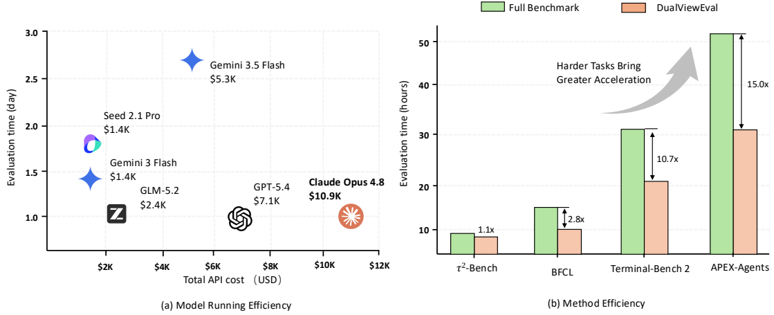
Figure 1 | Motivation and effect of agent-benchmark compression. (a) Runtime and API cost of representative model configurations on APEX-Agents benchmark. (b) Evaluation time for the full benchmark and the miniset selected by DualViewEval. Bars report average runtime and arrows indicate the acceleration from full evaluation to the miniset.
