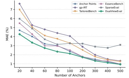
Figure 7 | Error Trend on BFCL. DualViewEval consistently outperforms baselines.
