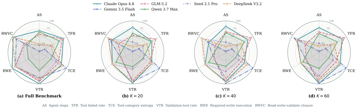
Figure 11 | Process profiles of six APEX-Agents models on the full benchmark and DualViewEval minisets at K \in \{20, 40, 60\} .
