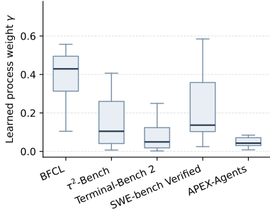
Figure 8 | Distribution of the learned \gamma for each benchmark.
