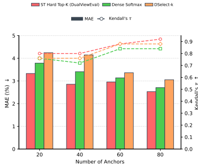
Figure 5 | Miniset-selector ablation on Apex-Agents.
