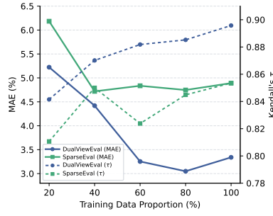
Figure 9 | Effect of the training-data proportion on BFCL.
