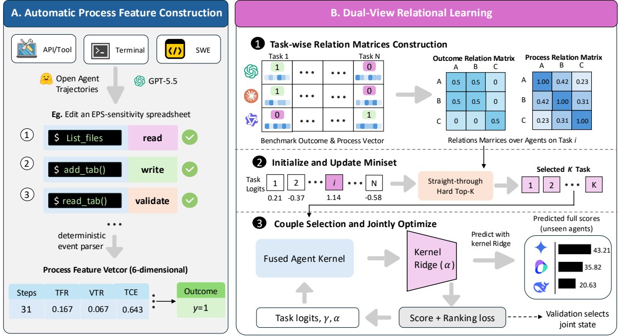
Figure 4 | Overview of DualViewEval. An APEX-Agents trajectory illustrates automatic extraction of six process measurements. Task-wise outcome and process relations are then fused to jointly optimize an exact-size hard Top- K miniset and a Kernel Ridge predictor using score and ranking feedback.
