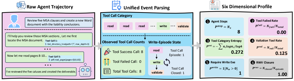
Figure 3 | Example of automatic process measurement construction.
