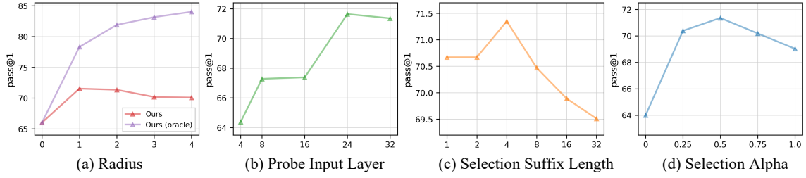
Figure 4: Ablation studies on four design choices of PILL.
