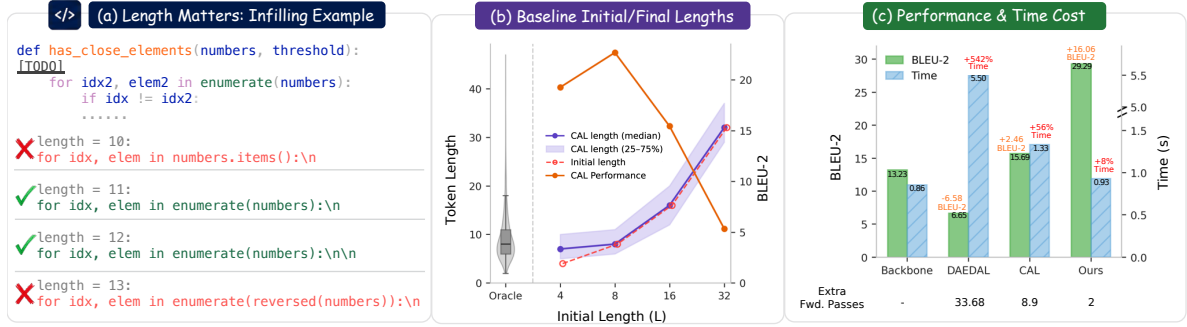
Figure 1: Motivation and Performance of PILL. (a) For DLM infilling tasks, correctness is sensitive to the span lengths. (b) Baselines must preset an initial length L and their final length stays tied to it, whereas PILL requires no preset length. (c) PILL attains the best performance with minimal overhead compared to fixed-length generation with backbones. Baselines are reported at initial length L = \{4, 8, 16, 32\} .
