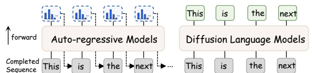
Figure 3: Forward-pass targets in ARMs and DLMs.
