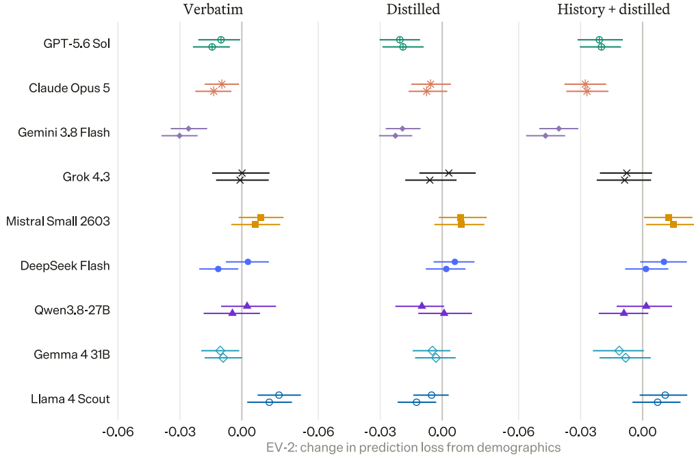
Figure 9. EV-2: does personal information improve prediction over demographics alone? Each point gives the change in average prediction error for one model and repetition among the same 430 people. Points left of zero indicate improvement, and points right of zero indicate worsening; the two points per row represent separate generations. Lines show paired 95 percent participant-bootstrap intervals, and an interval crossing zero leaves the direction uncertain. The three panels add original self-descriptions, distilled descriptions, or survey history plus distilled descriptions. These primary comparisons use jointly valid answers; Table 9 also accounts for unanswered questions.
