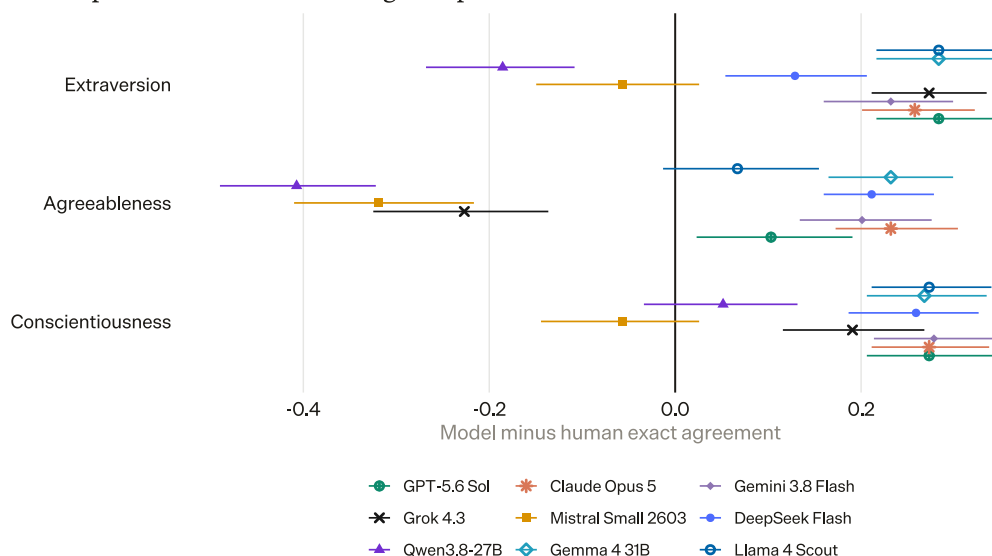
Figure 4. IV-1: repeated-answer agreement in Bainbridge sample 1. Each point compares a model with humans on one of three identically worded item pairs. Zero means equal repeat agreement, positive values mean that the model repeats itself more often, and negative values mean that it repeats itself less often. Lines show paired 95 percent participant-bootstrap intervals. Matching human agreement, rather than maximising consistency, is the comparison of interest.
