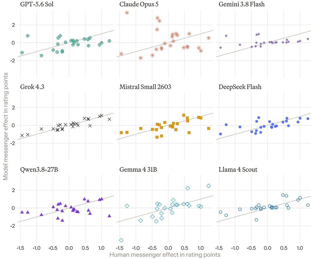
Figure 8. EV-3: messenger-effect recovery in FSD3587. Each panel shows 24 contrasts on the 0–10 argument-rating scale. Points on the diagonal match the human effect; departures show its attenuation, amplification, or reversal. Values with opposite signs indicate reversal. The scorecard retains model-minus-human error intervals for each contrast.
