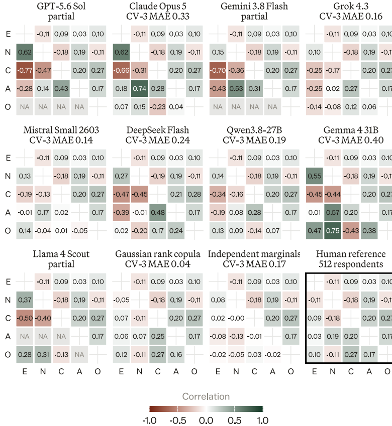
CV-3: Big Five relationships in SAPA
