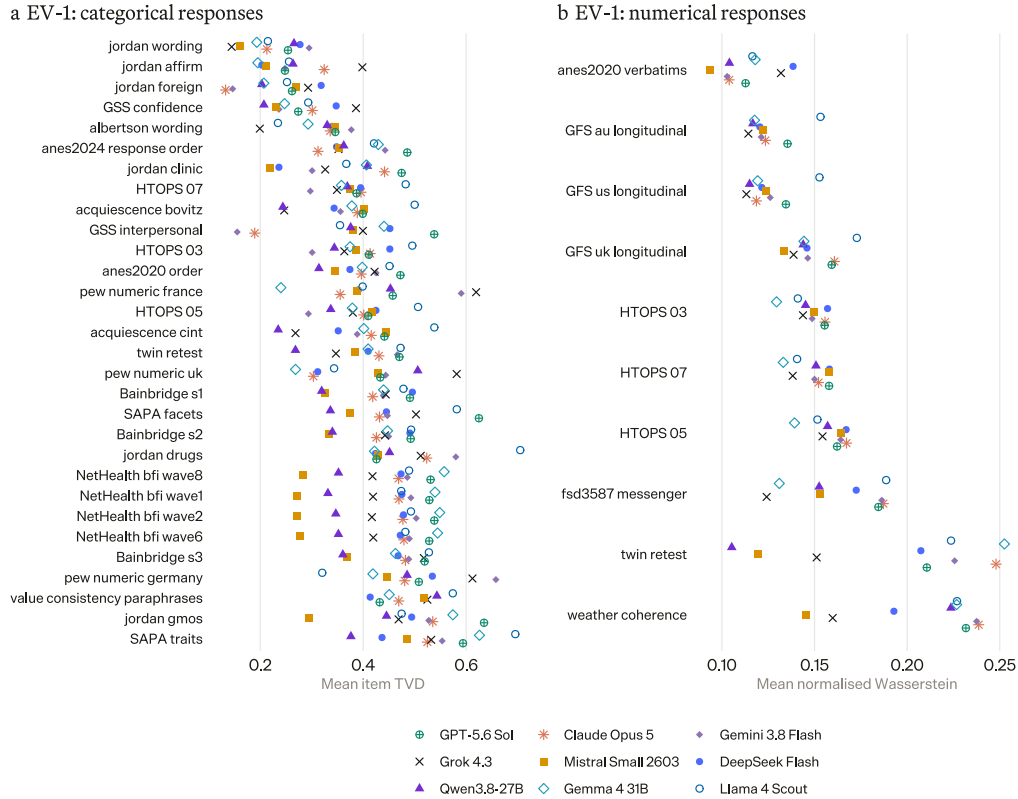
Figure 7. EV-1: response-distribution error by dataset and model. Points show average item-level error for the first generation, with smaller values indicating closer human agreement. The left panel compares categorical answer frequencies using total variation distance; the right compares numerical responses using Wasserstein distance divided by the response range. Both have zero at exact agreement, but they measure different discrepancies. Only tasks with complete estimable item support enter these means.
