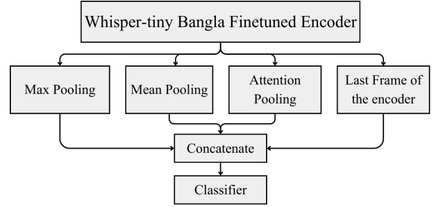
Figure 1: Our proposed model architecture with Whisper-tiny encoder finetuned in Bangla, multi-scale pooling and a classifier.
