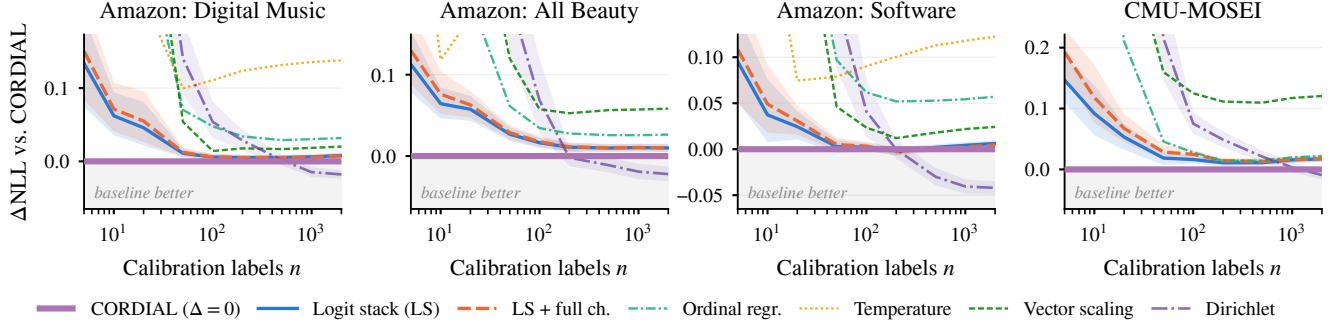
Fig. 1. Test NLL of each calibrator minus that of CORDIAL (above zero: CORDIAL better) against the number of calibration labels n , 7B reader, means over 20 label subsets; bands: paired 95% bootstrap intervals for the three strongest baselines. The logit stack (LS) combines temperature scaling, vector scaling, and ordinal regression. Curves above a panel’s range are cut.
