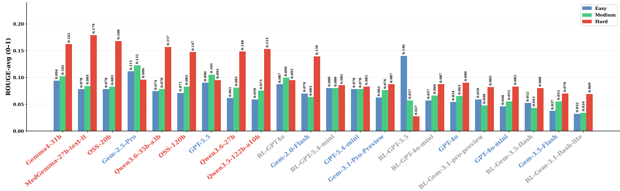
Figure 10: ROUGE-avg scores across all models and difficulty tiers (Label color: Blue = RAG Proprietary; Red = RAG Local; Gray = Baseline)
