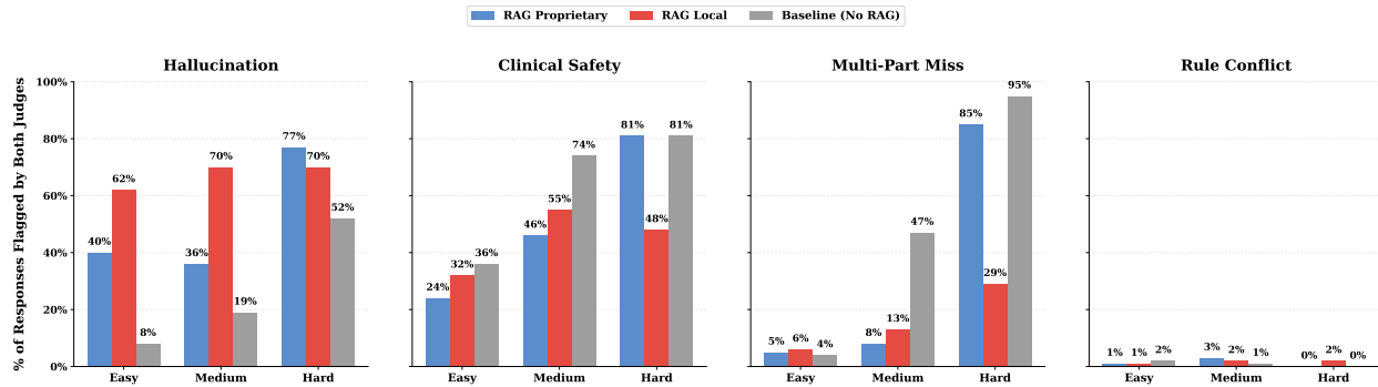
Figure 7: LLM-as-a-Judge Binary Flags Assessment by Model Types and Difficulty Tiers
