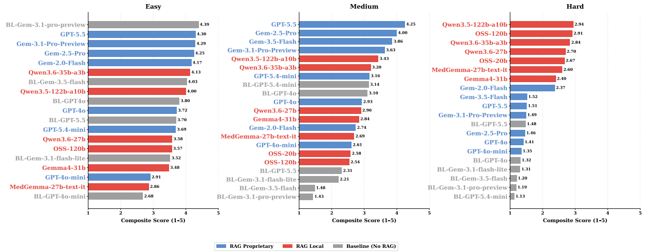
Figure 5: LLM-as-a-Judge Scores for all difficulty tiers
