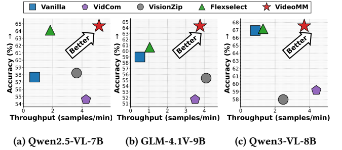
Figure 1: VideoMM sets a new accuracy–efficiency frontier on LongVideoBench, achieving a 6.13× inference speedup with a 7.4% accuracy gain over the vanilla baseline, and a 2.73× speedup over FlexSelect without accuracy loss.
