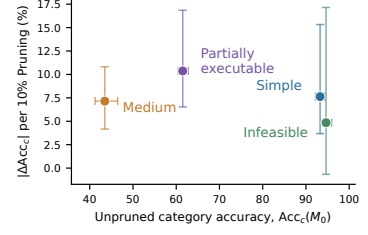
Figure 6: |\Delta\text{Acc}_c| per additional 10% pruning versus mean \text{Acc}_c(M_0) across public datasets.
