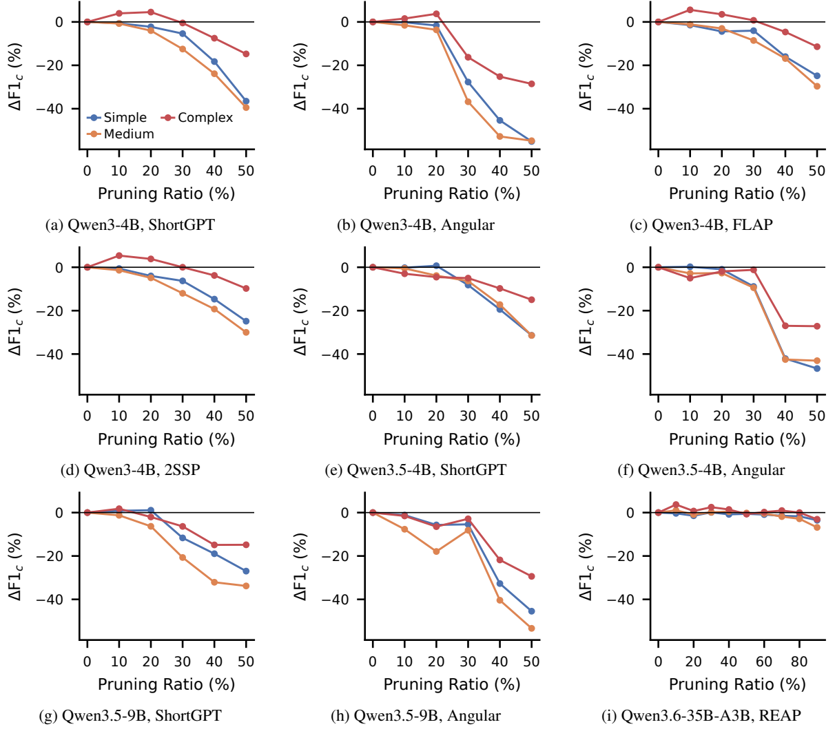
Figure 20: SHTC: operation-level F1 of the task-complexity categories. \Delta F1_c relative to M_0 for the complexity categories present in the source against pruning ratio. Each subfigure is one LLM and pruning method.
