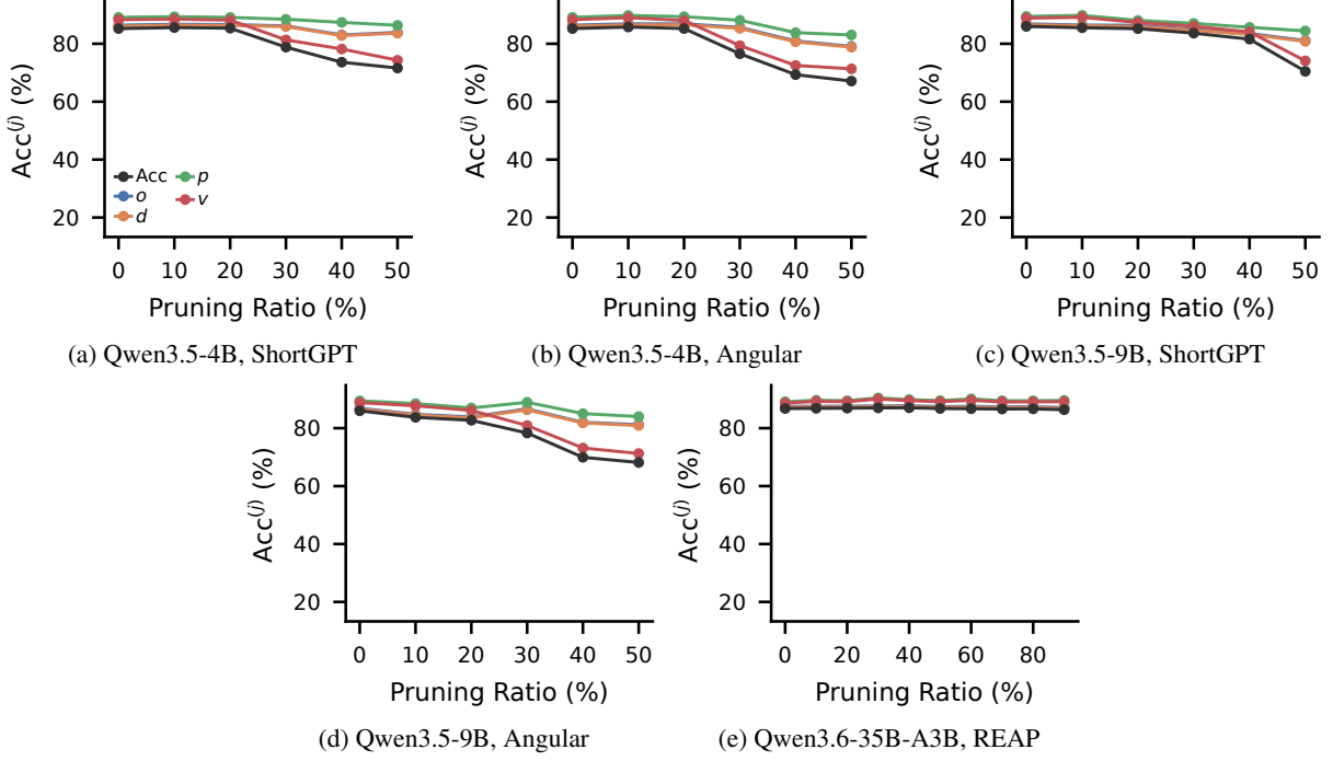
Figure 9: HomeBench: action-component accuracy for the remaining LLM-pruning combinations. Acc together with the four action components o , d , p , v against pruning ratio. Each subfigure is one LLM and pruning method. Qwen3-4B results are in Figure 2.
