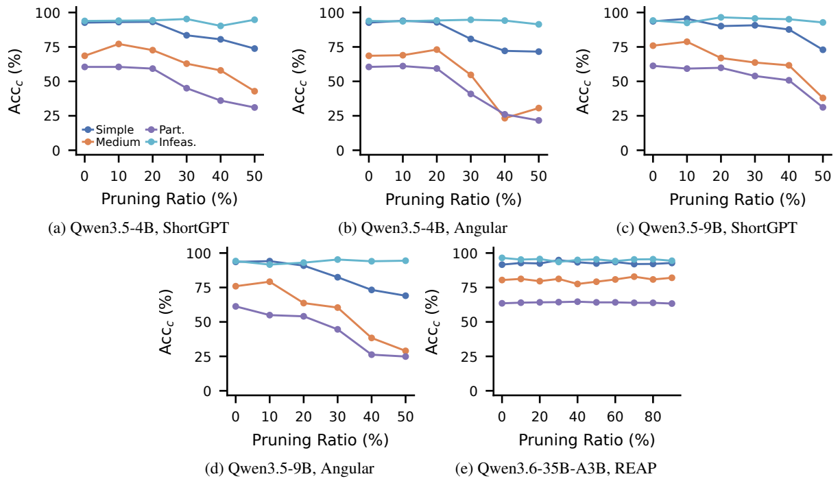
Figure 12: HomeBench: accuracy of task-complexity categories for the remaining LLM-pruning combinations. Acc_c for the complexity categories present in the source against pruning ratio. Each subfigure is one LLM and pruning method. Qwen3-4B results are in Figure 3.
