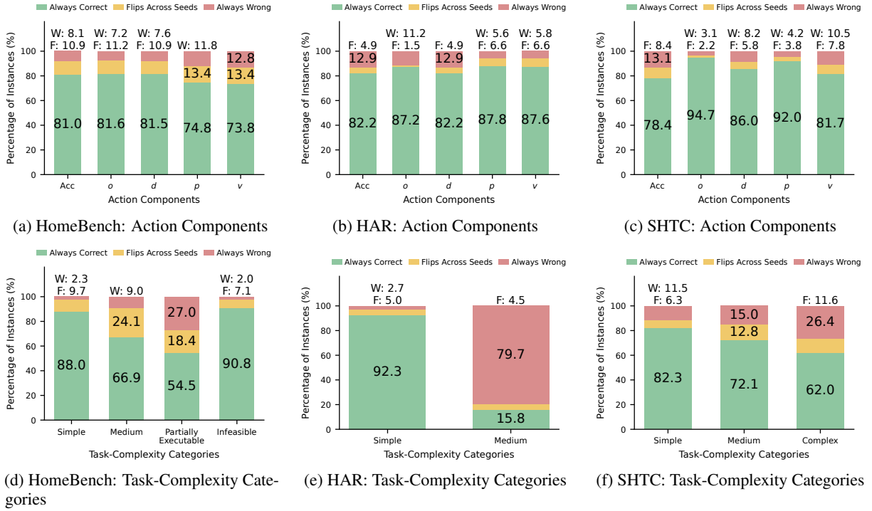
Figure 22: Qwen3.6 MoE robustness across seeds by action component and task-complexity level. Labels prefixed by C, F, or W above a bar denote Always Correct, Flips Across Seeds, or Always Wrong.
