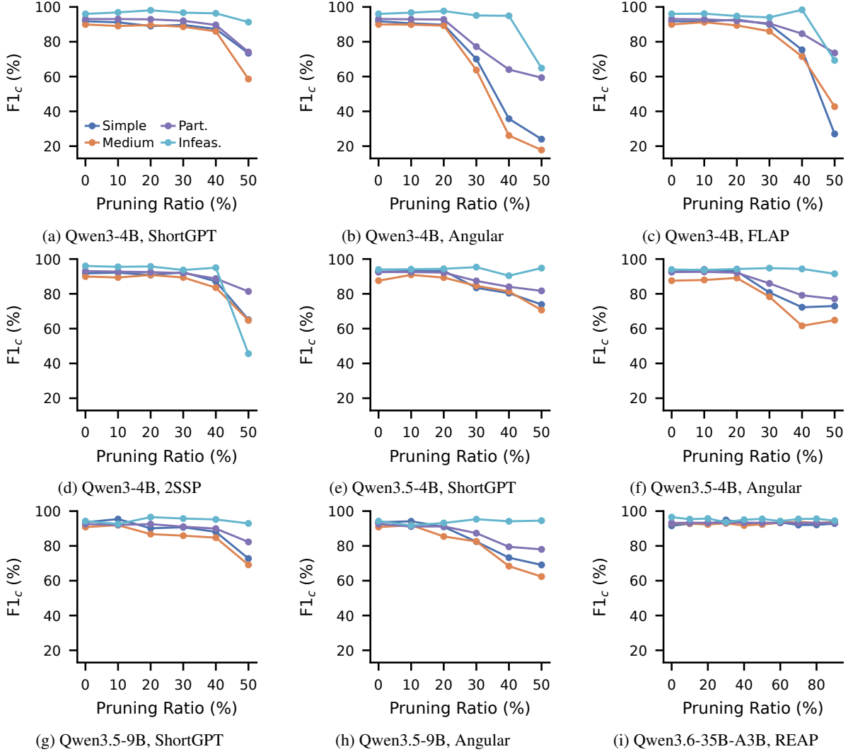
Figure 18: HomeBench: operation-level F1 of the task-complexity categories. F1_c for the complexity categories present in the source against pruning ratio. Each subfigure is one LLM and pruning method.
