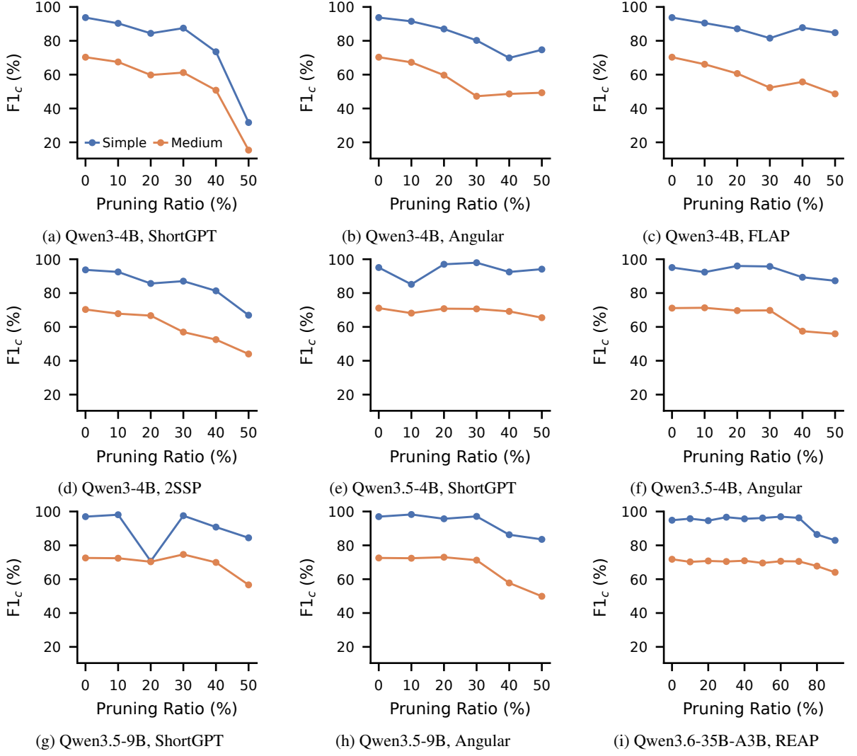
Figure 19: HAR: operation-level F1 of the task-complexity categories. F1_c for the complexity categories present in the source against pruning ratio. Each subfigure is one LLM and pruning method.
