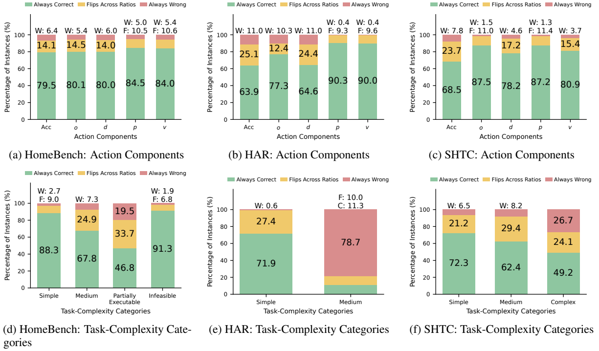
Figure 21: Qwen3.6 MoE robustness across REAP pruning ratios by action component and task-complexity level. Labels prefixed by C, F, or W above a bar denote Always Correct, Flips Across Ratios, or Always Wrong.
