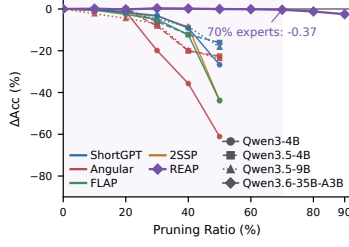
Figure 4: Average \Delta\text{Acc} of different LLMs under different pruning methods across three datasets.
