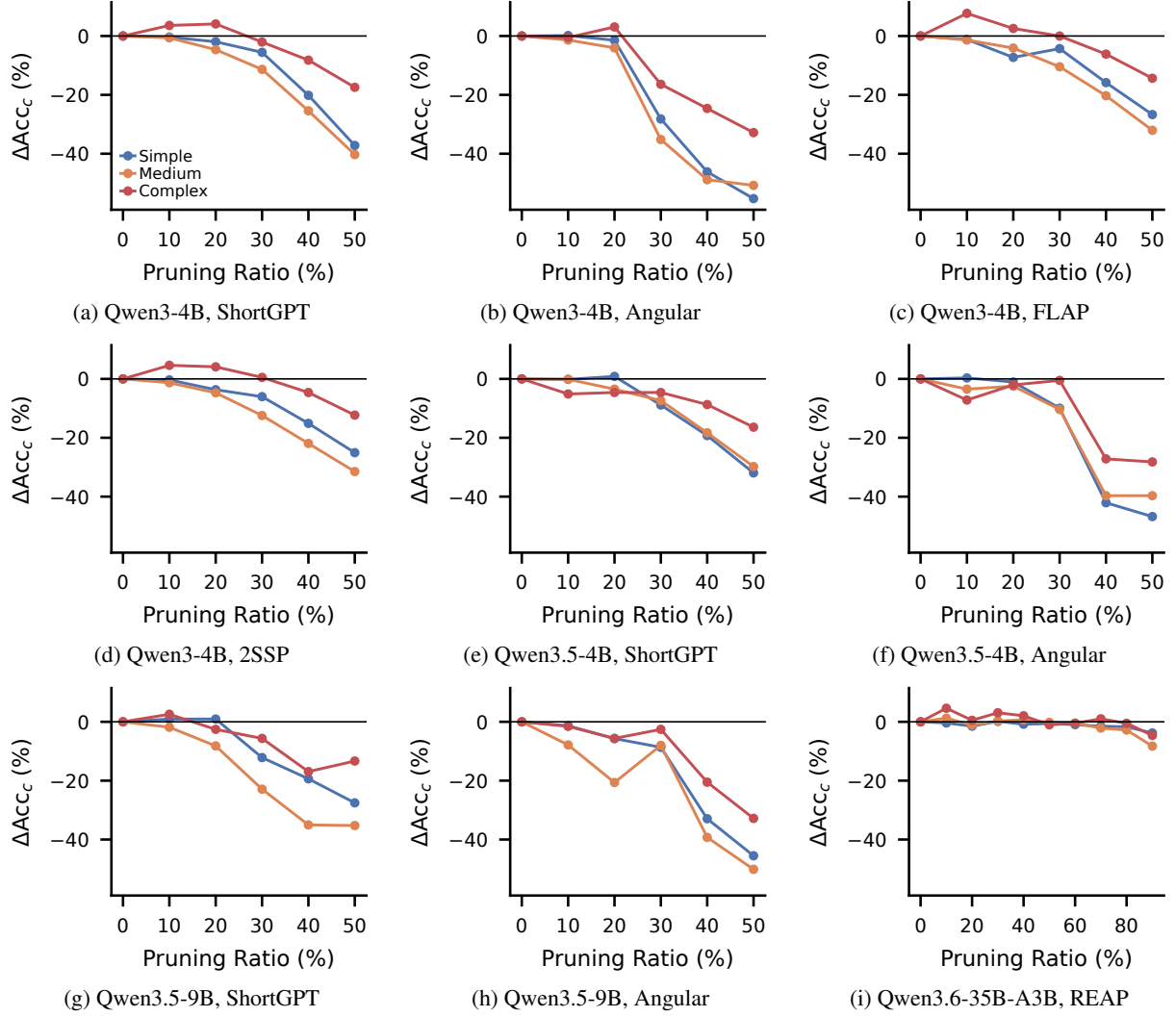
Figure 14: SHTC: accuracy of task-complexity categories. \Delta Acc relative to M_0 for the complexity categories present in the source against pruning ratio. Each subfigure is one LLM and pruning method.
