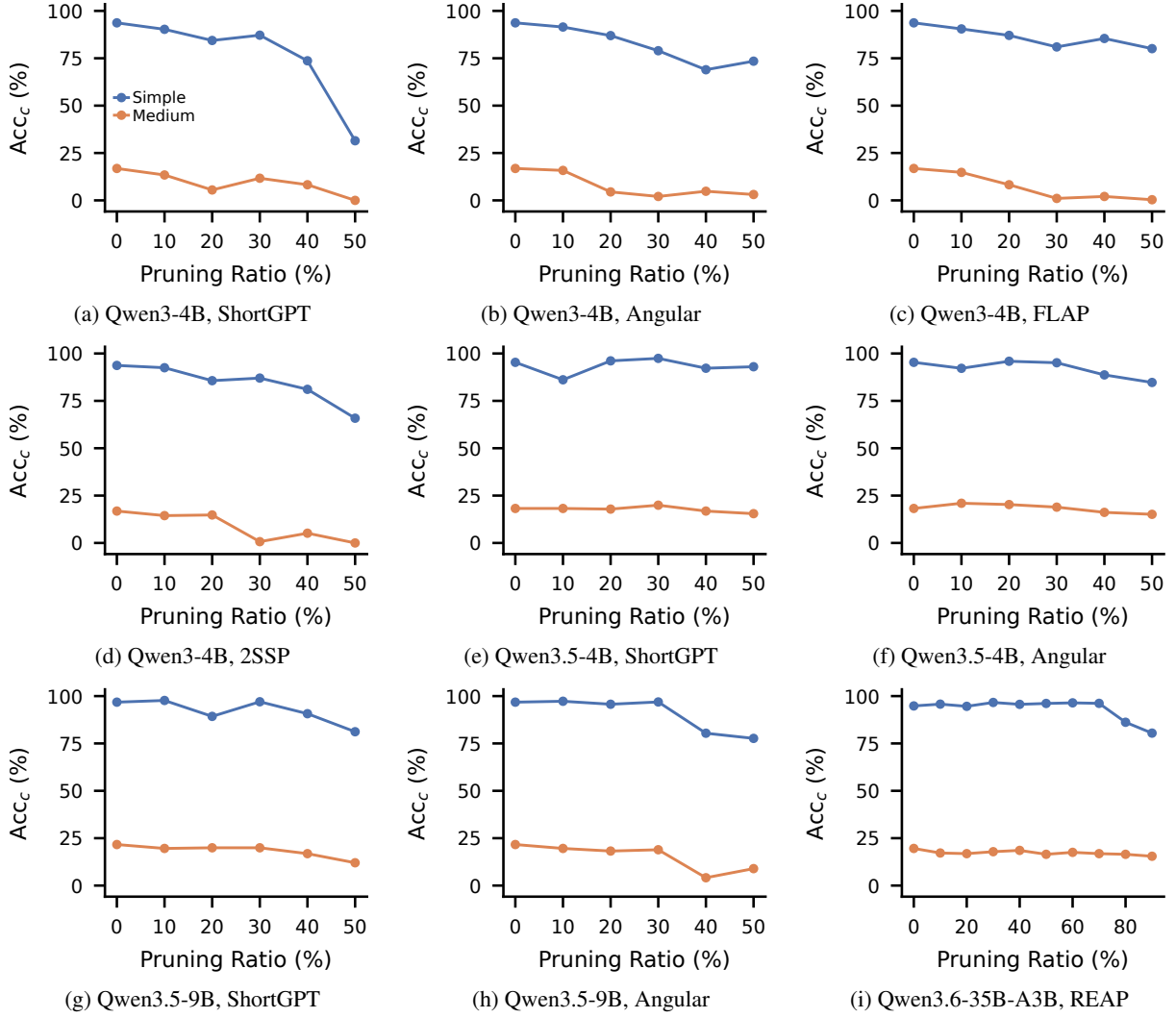
Figure 13: HAR: accuracy of task-complexity categories. Acc_c for the complexity categories present in the source against pruning ratio. Each subfigure is one LLM and pruning method.
