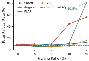
Figure 7: False-refusal rate on executable HomeBench requests.
