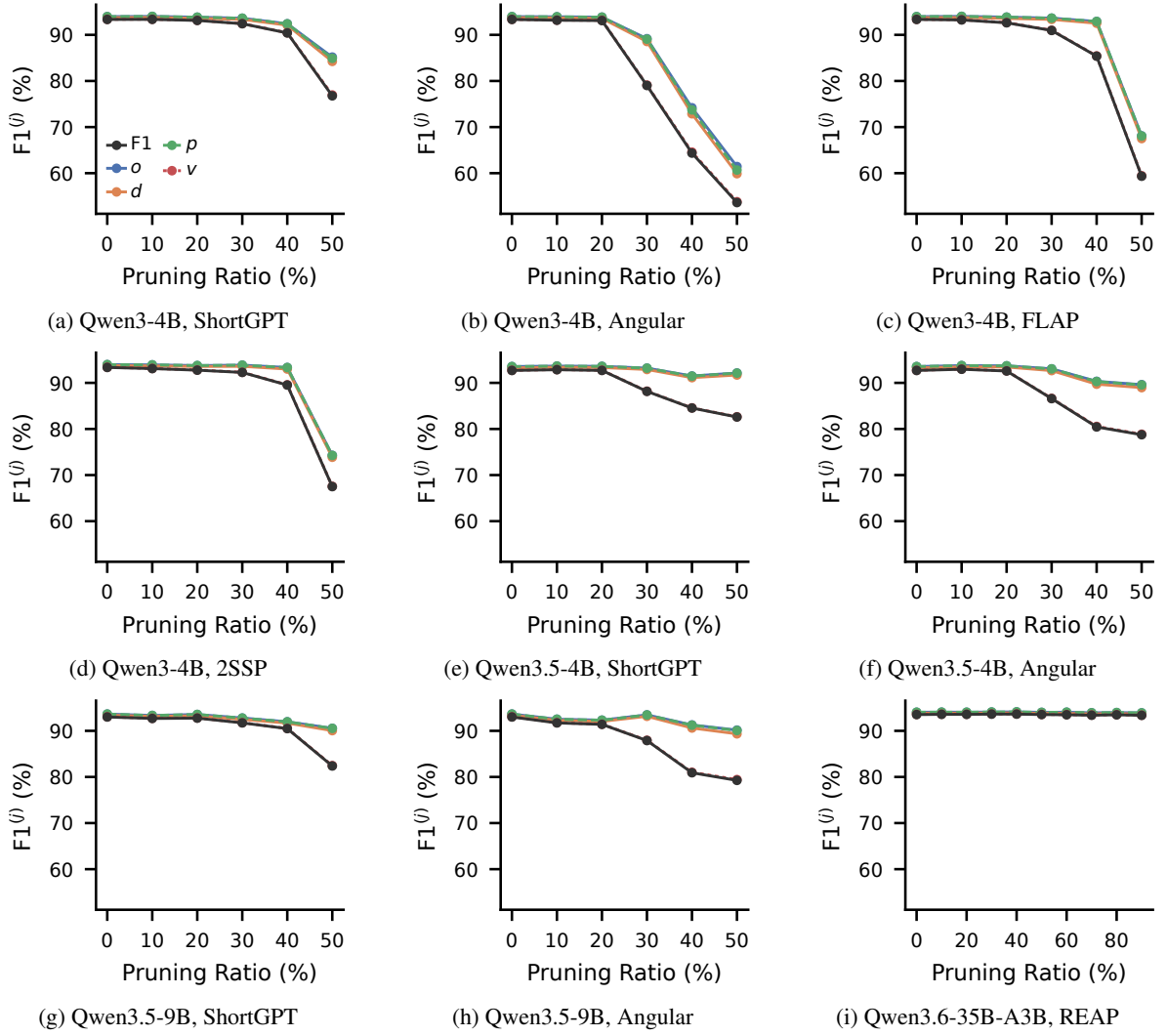
Figure 15: HomeBench: operation-level F1 of the action components. F1 together with the four action components o , d , p , v against pruning ratio. Each subfigure is one LLM and pruning method.
