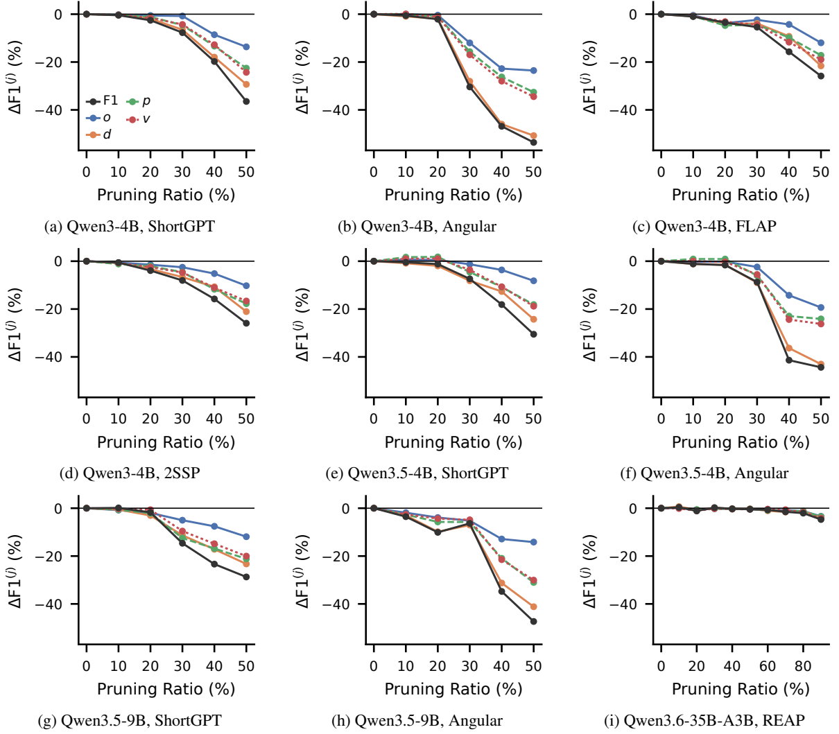
Figure 17: SHTC: operation-level F1 of the action components. \Delta F1 relative to M_0 together with the four action components o, d, p, v against pruning ratio. Each subfigure is one LLM and pruning method.
