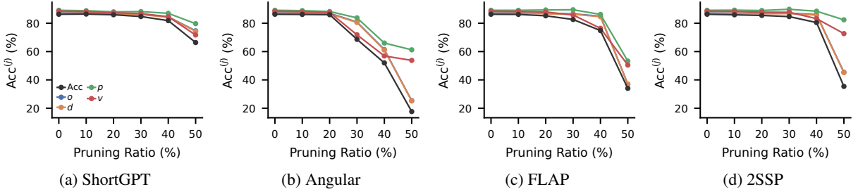
Figure 2: HomeBench action-component accuracy across pruning ratios for four pruning methods in Qwen3-4B.
