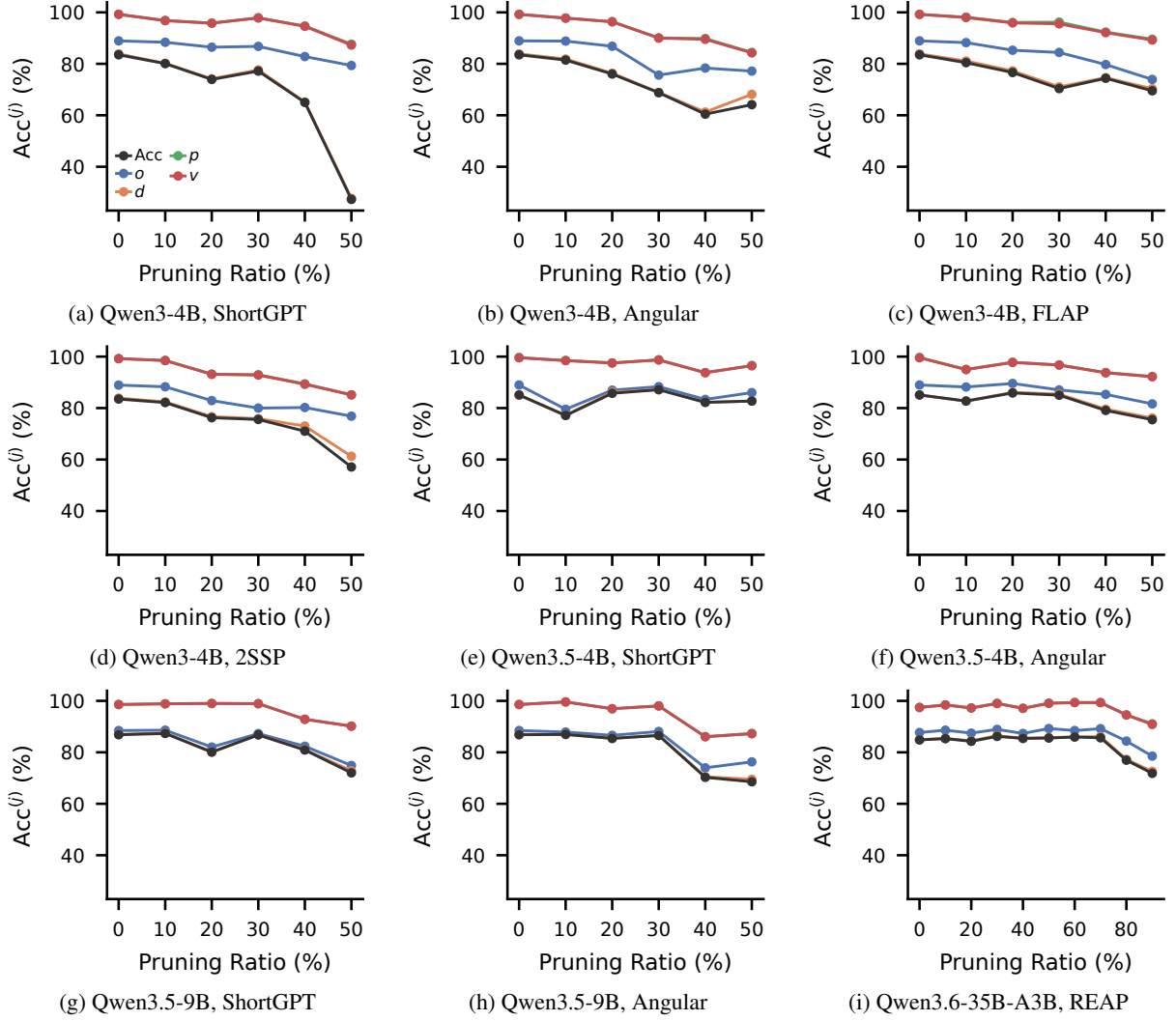
Figure 10: HAR: action-component accuracy. Acc together with the four action components o, d, p, v against pruning ratio. Each subfigure is one LLM and pruning method.
