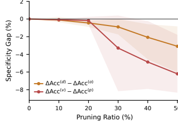
Figure 5: Specificity gaps \Delta\text{Acc}^{(d)} - \Delta\text{Acc}^{(o)} and \Delta\text{Acc}^{(v)} - \Delta\text{Acc}^{(p)} across dense pruning configurations.
