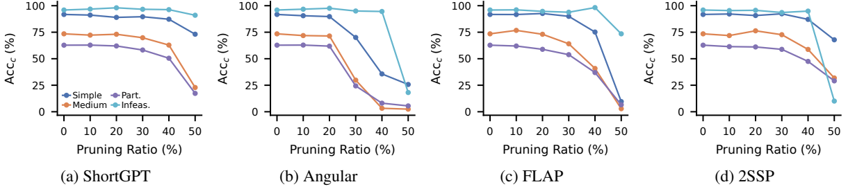
Figure 3: HomeBench complexity-level accuracy across pruning ratios for four pruning methods in Qwen3-4B.
