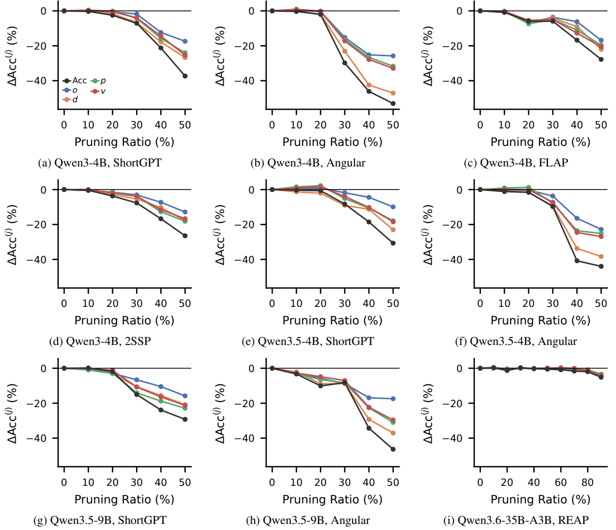
Figure 11: SHTC: action-component accuracy. \Delta \text{Acc} relative to M_0 together with the four action components o, d, p, v against pruning ratio. Each subfigure is one LLM and pruning method.
