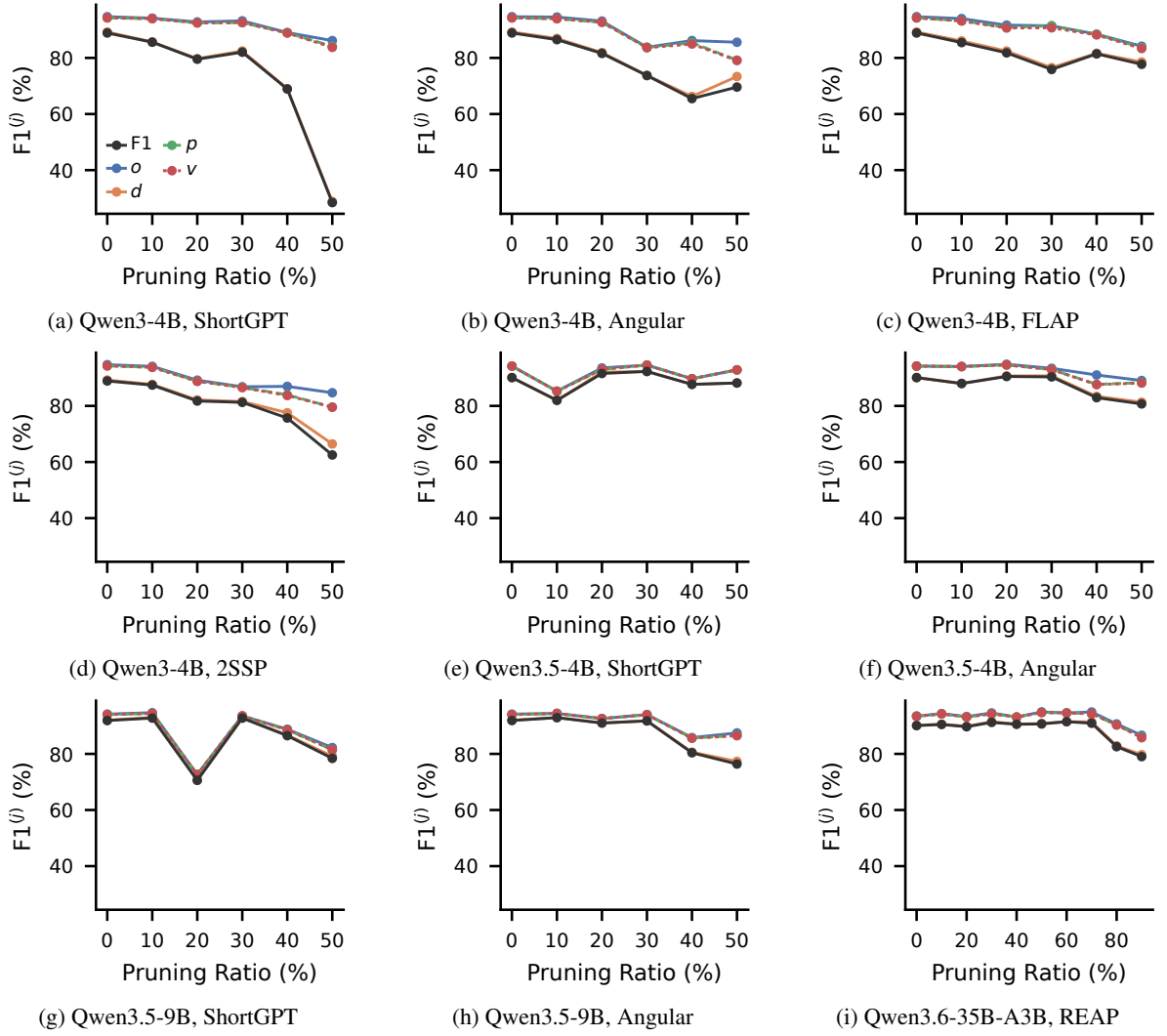
Figure 16: HARM: operation-level F1 of the action components. F1 together with the four action components o, d, p, v against pruning ratio. Each subfigure is one LLM and pruning method.
